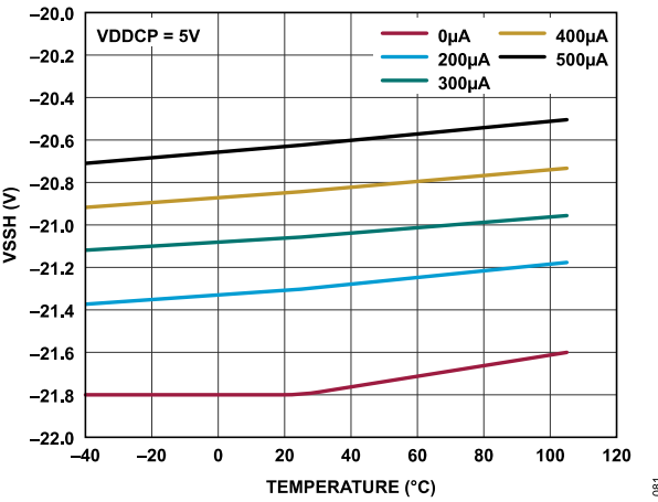
Figure 80. VSSH vs. Temperature for Various VSSH Loads, VDDCP = 5 V
