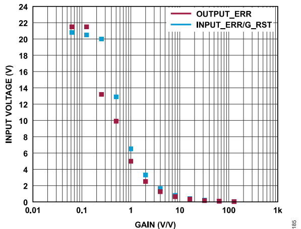
Figure 79. Positive Error Trip Thresholds with Single-Ended Input
