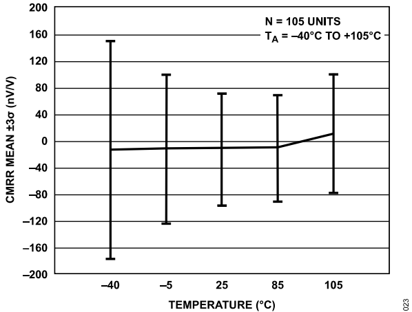
Figure 23. CMRR Mean \pm 3\sigma vs. Temperature (Gain = 128 V/V)
