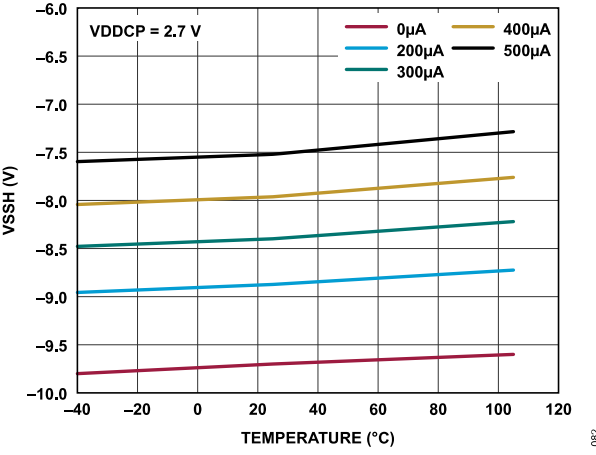
Figure 81. VSSH vs. Temperature for Various VSSH Loads, VDDCP = 2.7 V
