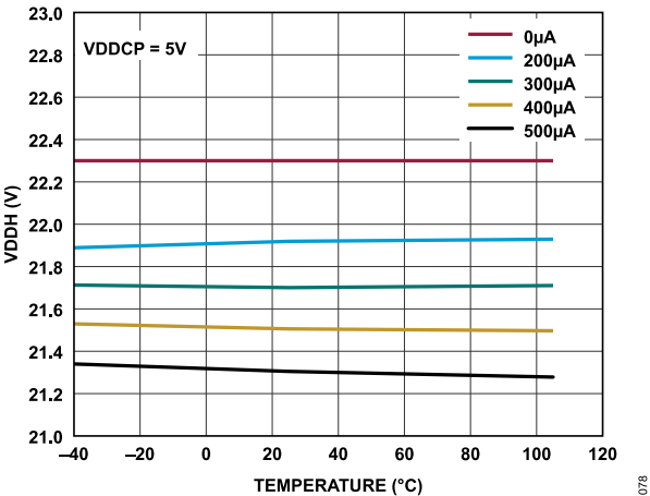
Figure 77. VDDH vs. Temperature for Various VDDH Loads, VDDCP = 5 V
