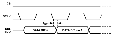
Figure 4. SPI Register Read Timing Diagram
