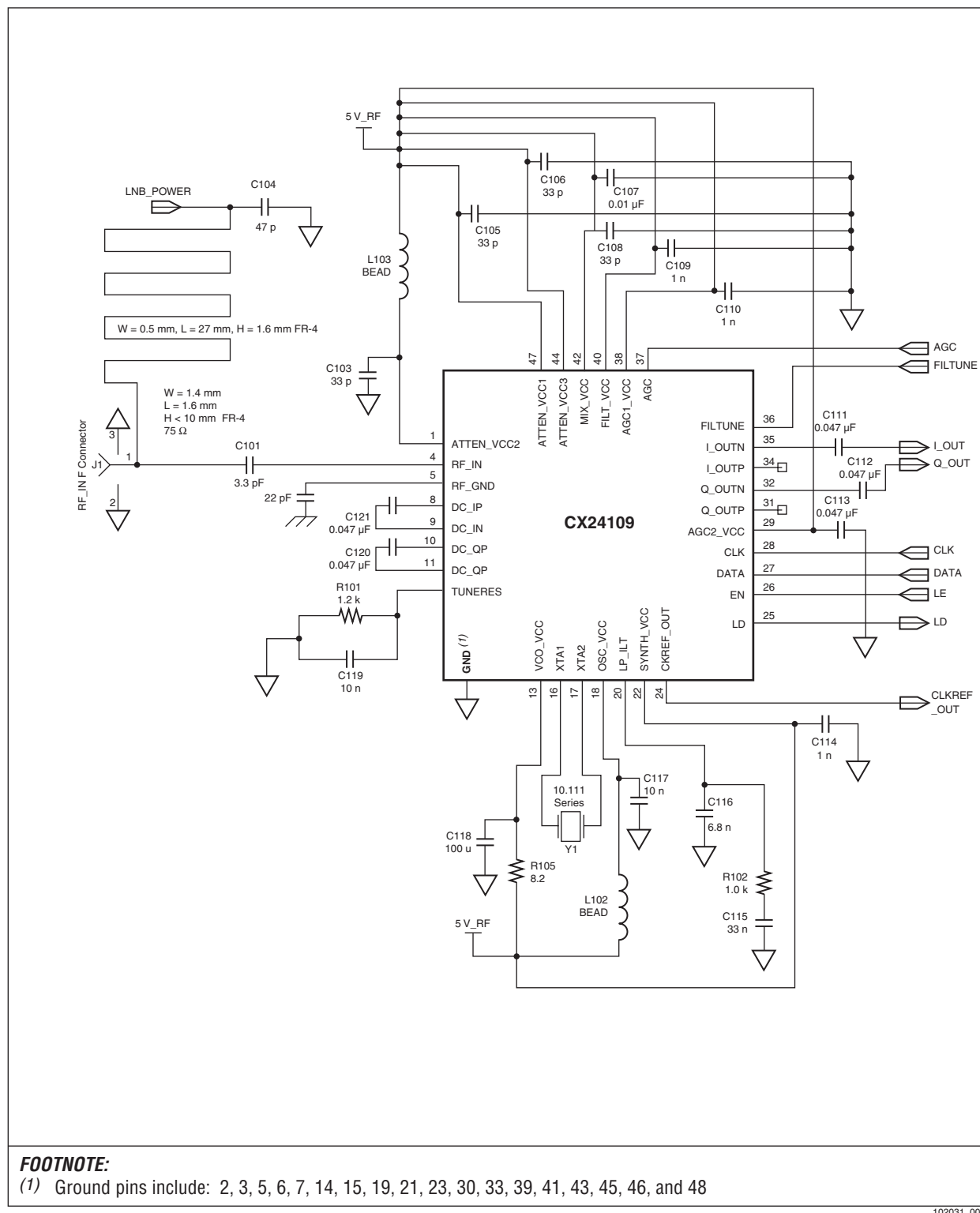
Figure 6. Simplified Application Schematic (Page 1 of 2)
