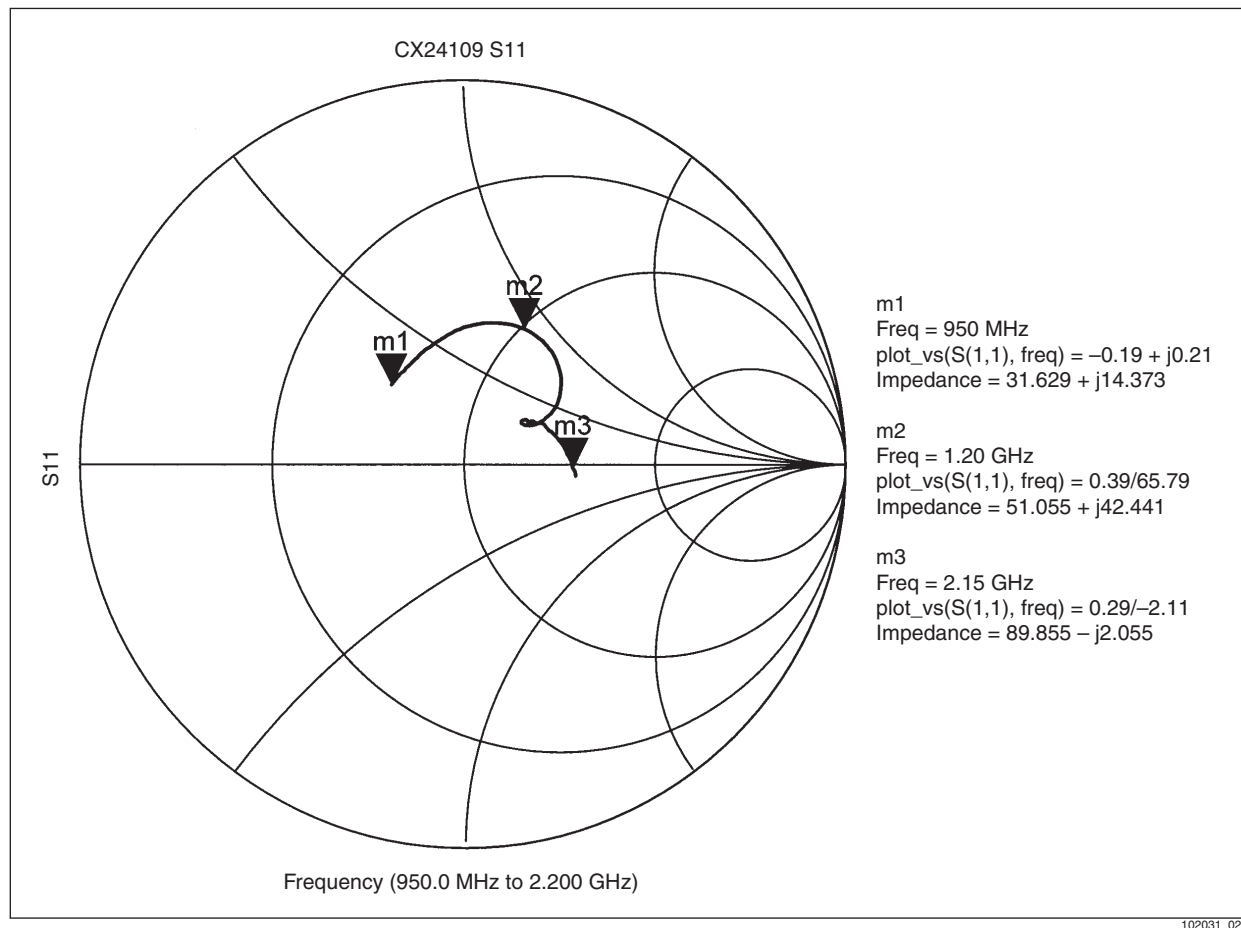
Figure 8. Reflection Coefficient at Input of CX24109
