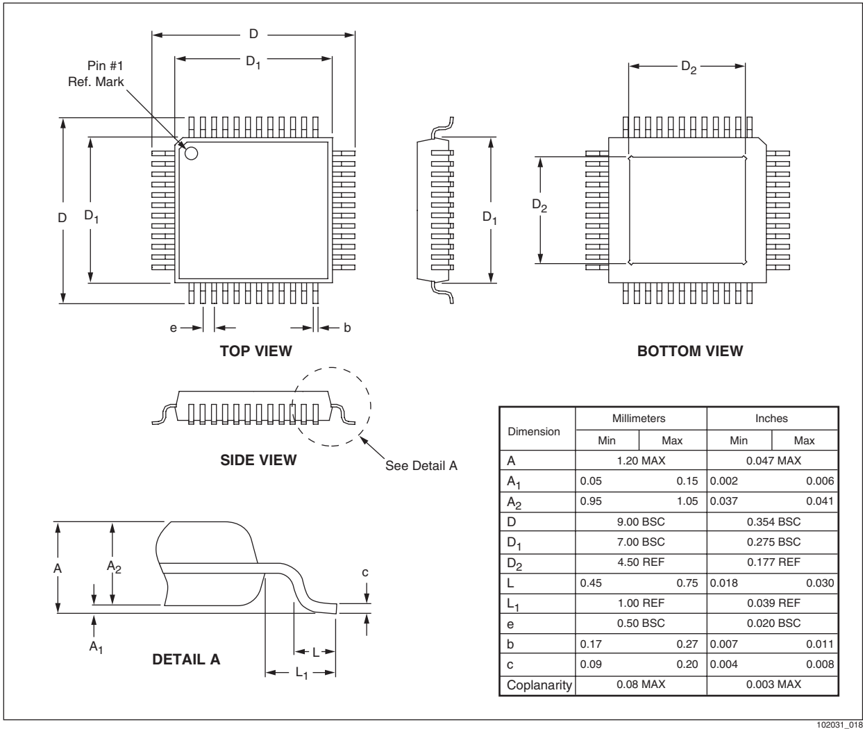
Figure 17. 48-pin eTQFP Package Diagram
