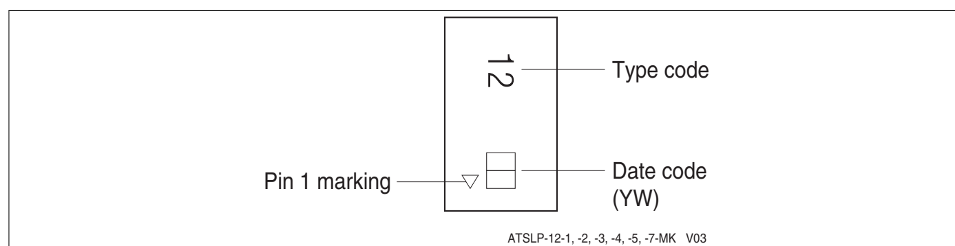
Figure 12: Marking Specification (top view)
