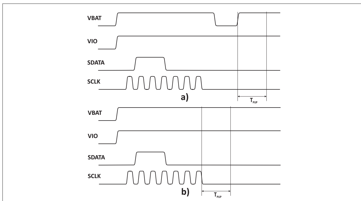
Figure 3: Power-Up Settling Time Definition: a) when the device is already in Active Mode. b) when changing from Low Power Mode to Active Mode.
