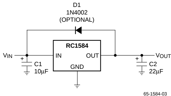
Figure 1. Optional Protection Diode
