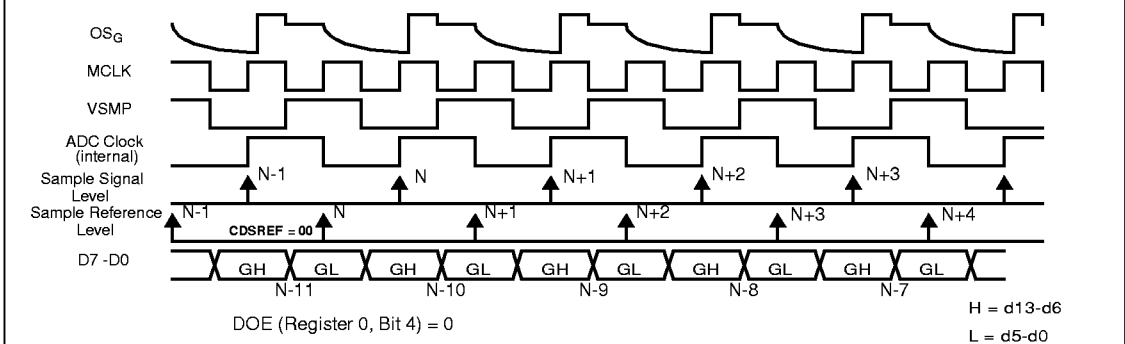
Diagram 6: Divide by 2 Monochrome Mode Sample and Data Output Timing (Green Input shown)
