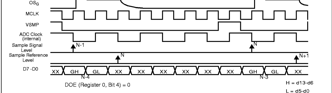
Diagram 4: Divide by 8 Monochrome Mode Sample and Data Output Timing (Green Input Shown)
