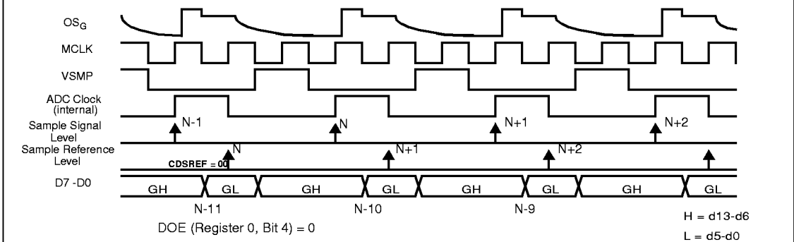
Diagram 5: Divide by 3 Monochrome Mode Sample and Data Output Timing (Green Input shown)
