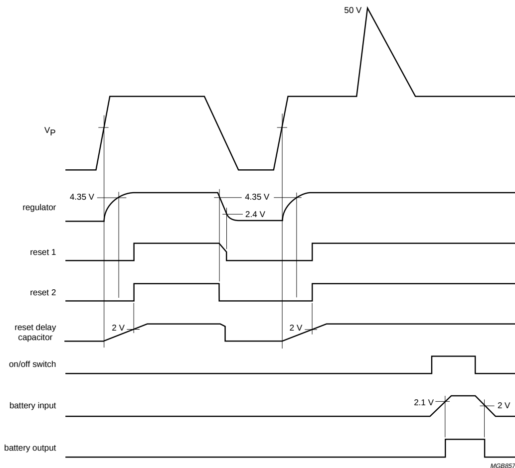
Fig.3 Timing diagrams.
