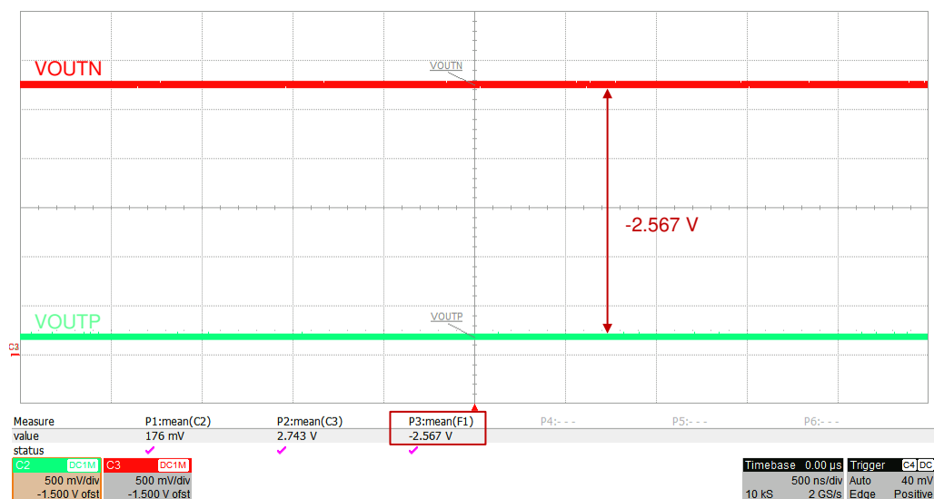
Figure 7-5. Typical Fail-Safe Output of the AMC3330-Q1
