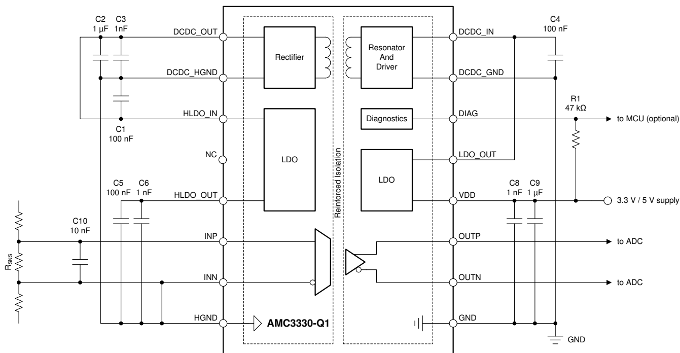
Figure 9-1. Decoupling the AMC3330-Q1
