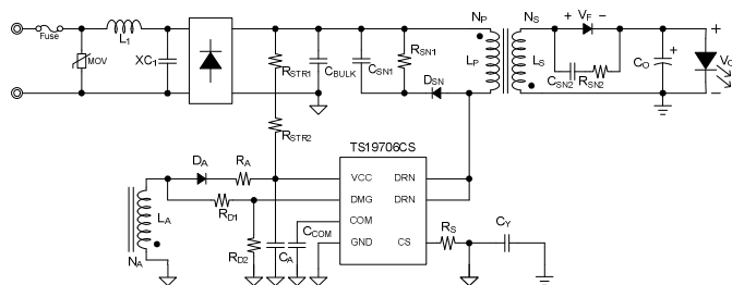
Flyback Converter
