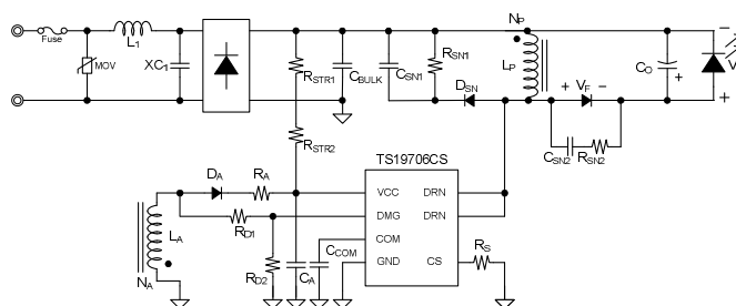
Buck-Boost Converter
