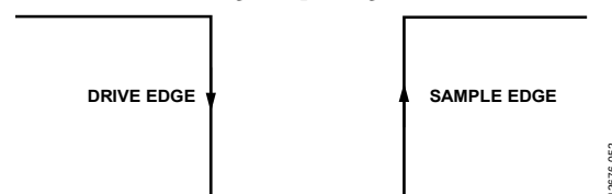
Figure 42. SPI Mode 3 SCLK Edges
