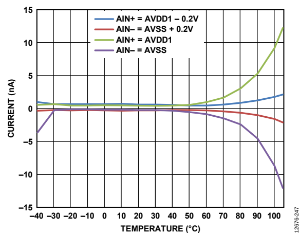
Figure 38. Analog Input Current vs. Temperature
