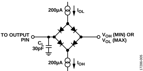
Figure 5. Load Circuit for the SDO Timing Diagram
