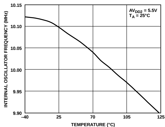
Figure 60. Internal Oscillator Frequency vs. Temperature
