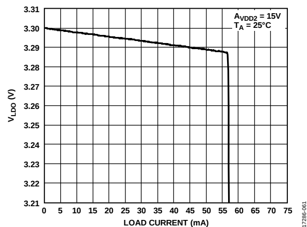
Figure 61. V LDO vs. Load Current
