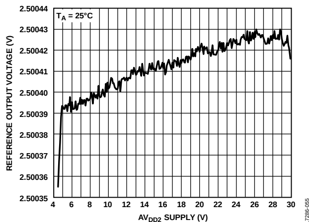
Figure 55. Reference Output Voltage vs. AV_{DD2} Supply
