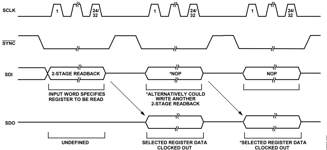
Figure 72. Two-Stage Readback Example
