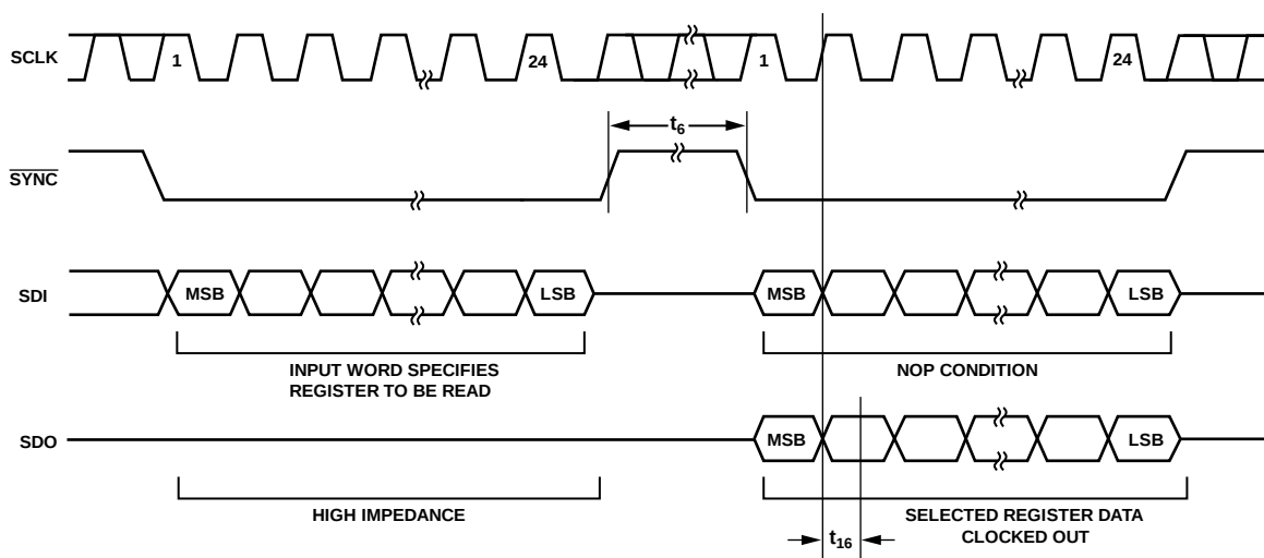
Figure 3. Readback Timing Diagram
