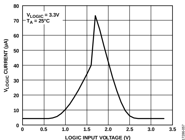
Figure 57. V LOGIC Current vs. Logic Input Voltage
