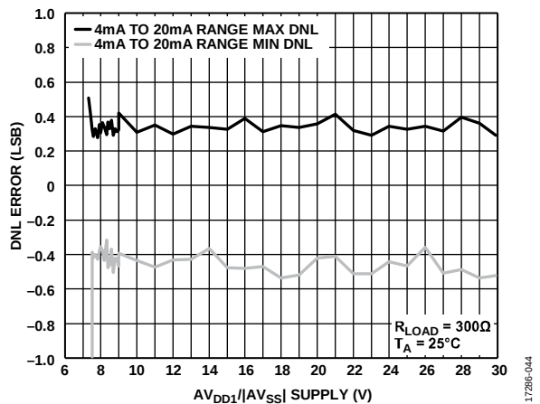
Figure 44. DNL Error vs. AV_{DD1}/AV_{SS} Supply, Internal R_{SET}
