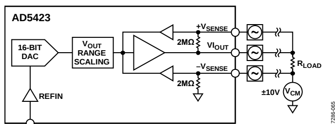
Figure 65. Voltage Output Load Connection
