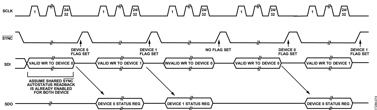
Figure 74. Shared \overline{\text{SYNC}} Autostatus Readback Example
