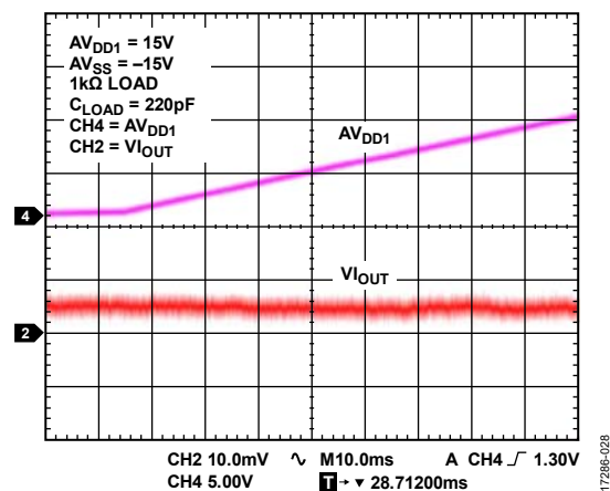
Figure 28. V_{OUT} vs. Time on Power Up
