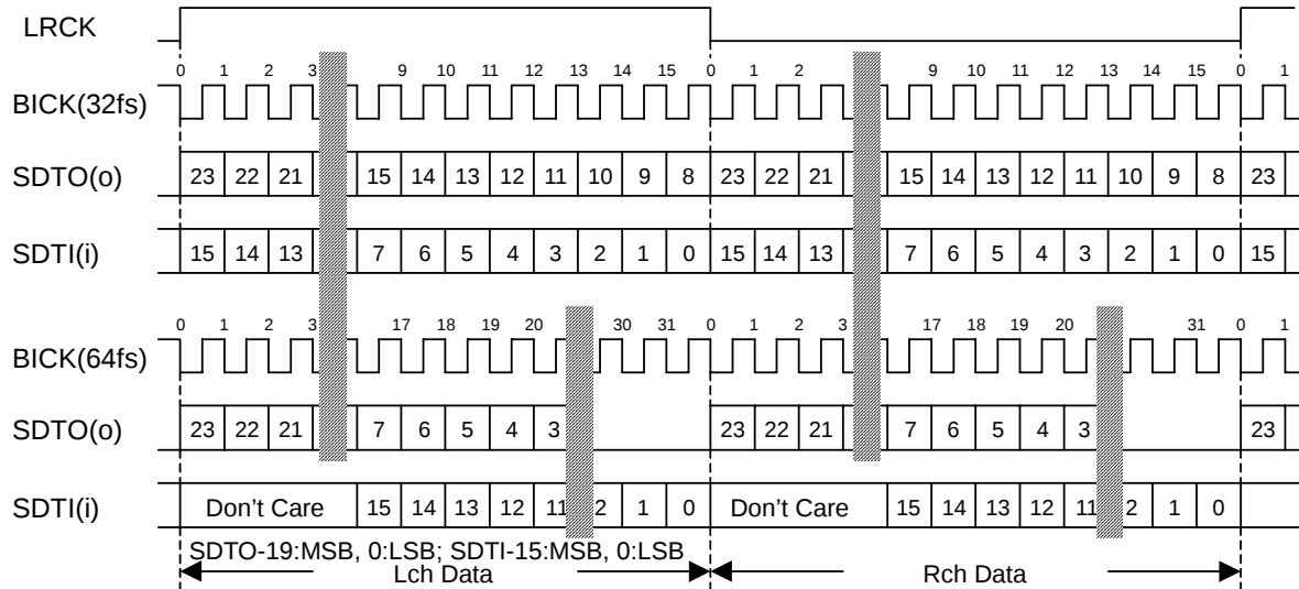
Figure 1. Mode 0 Timing
