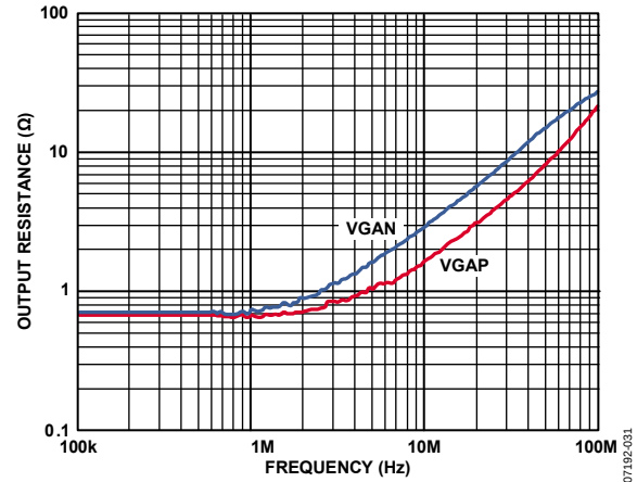
Figure 31. Output Resistance vs. Frequency for the VGA/Preamplifier See Figure 60
