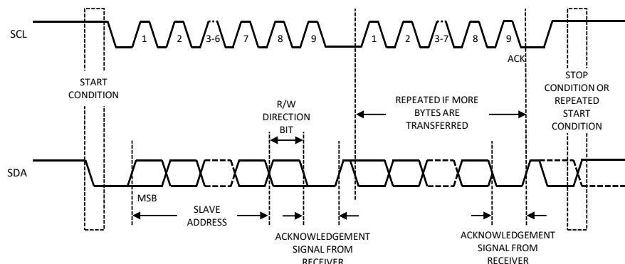
Figure 2. Data Transfer on I 2 C Serial Bus
