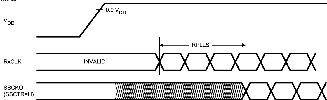
FIGURE 9. FPD-Link Receiver Phase Lock Loop Wake-Up Time
