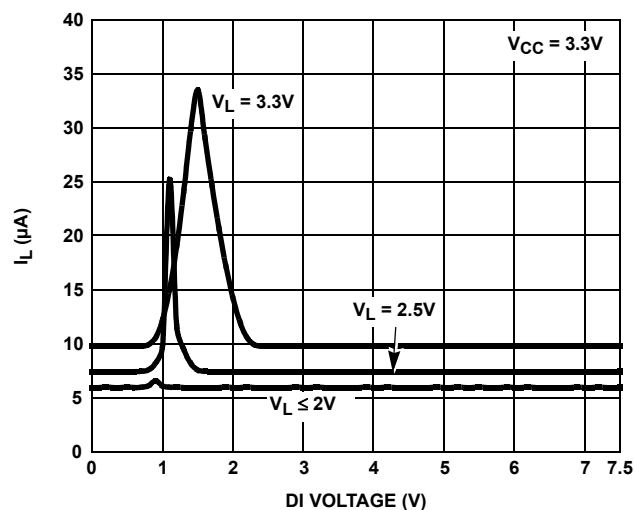
FIGURE 9. V_L SUPPLY CURRENT vs LOGIC PIN VOLTAGE
