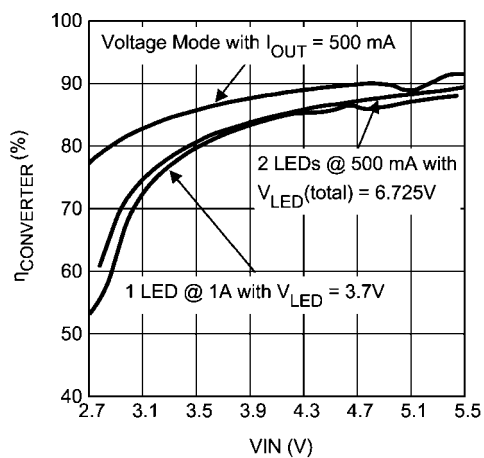
Converter Efficiency vs V_{IN}
