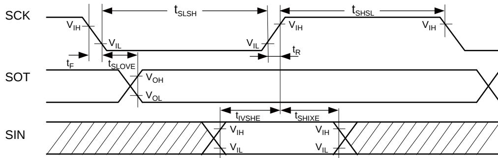
External shift clock mode
