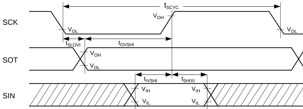
Internal shift clock mode
