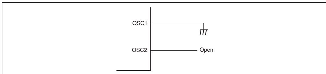
Figure 22.8 Pin Handling when Subclock is not Used
