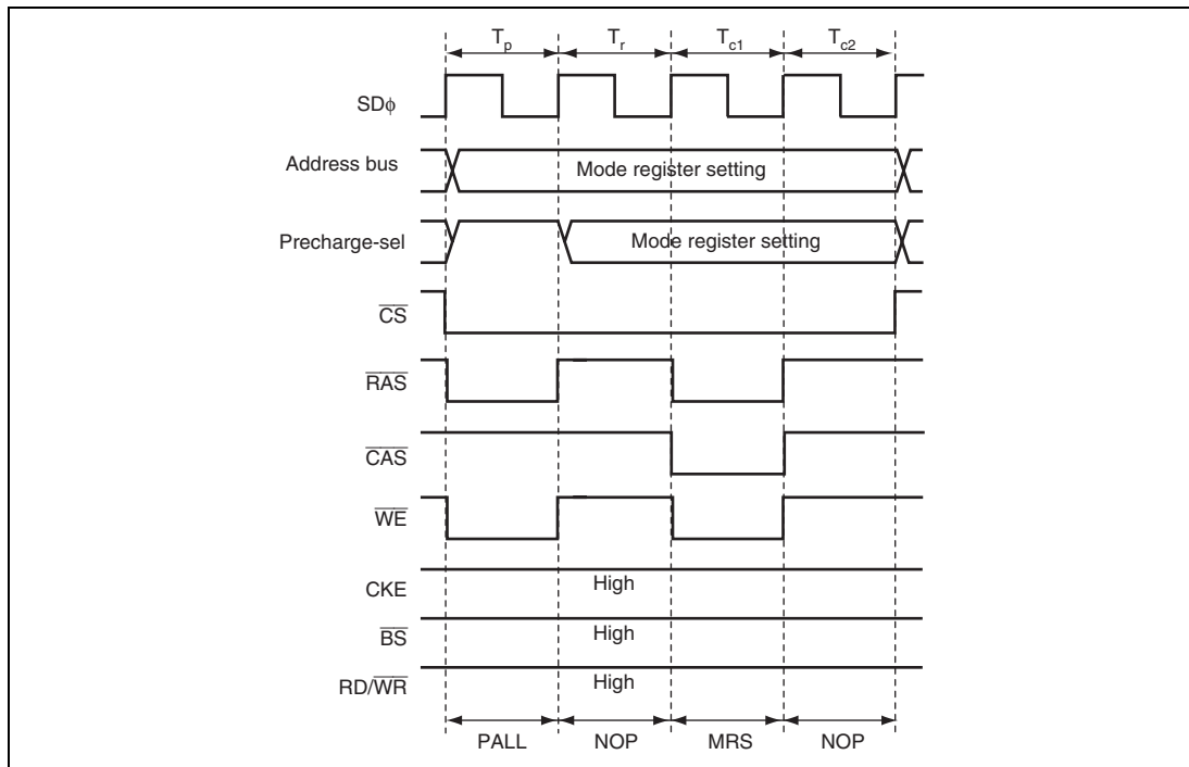
Figure 6.81 Timing of Setting SDRAM Mode Register
