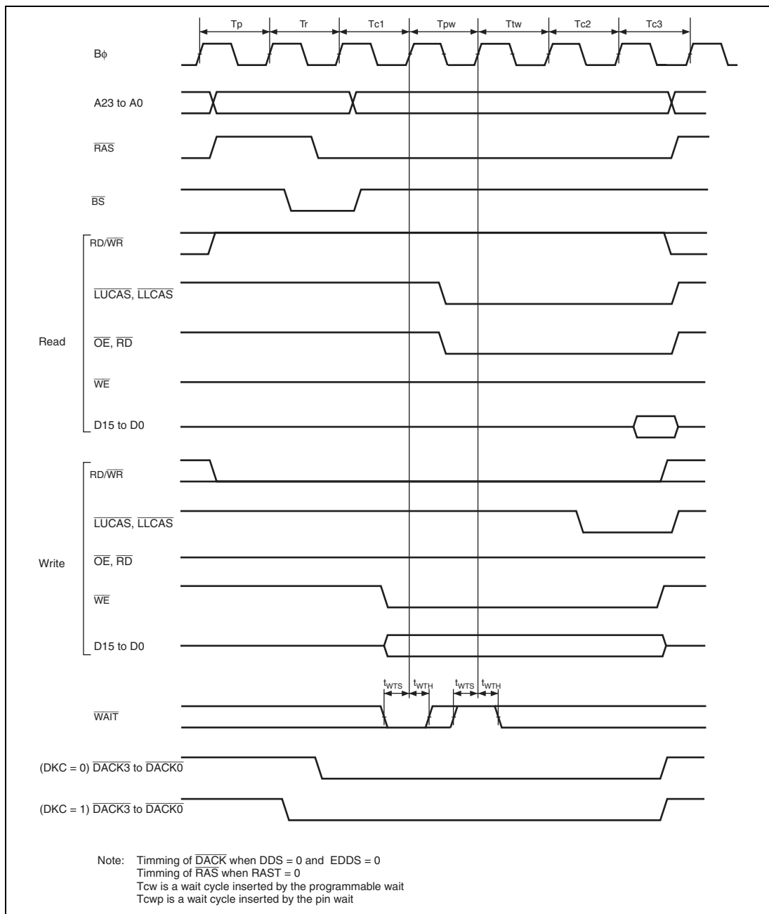
Figure 25.23 DRAM Access Timing: Three-State Access, One Wait
