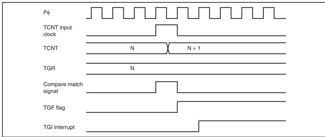
Figure 10.38 TGI Interrupt Timing (Compare Match)
