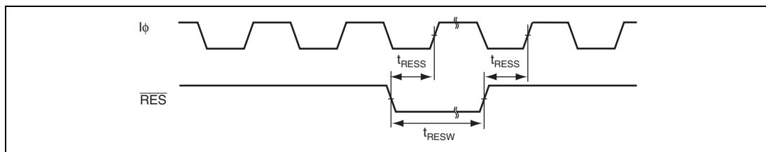
Figure 25.6 Reset Input Timing
