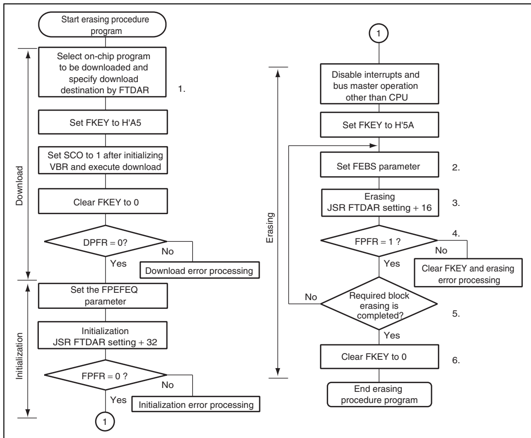
Figure 21.14 Erasing Procedure in User Program Mode
