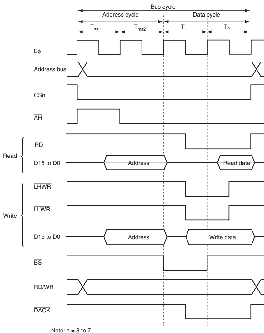
Figure 6.32 16-Bit Access Space Access Timing (ABWHn = 0, ABWLn = 1)
