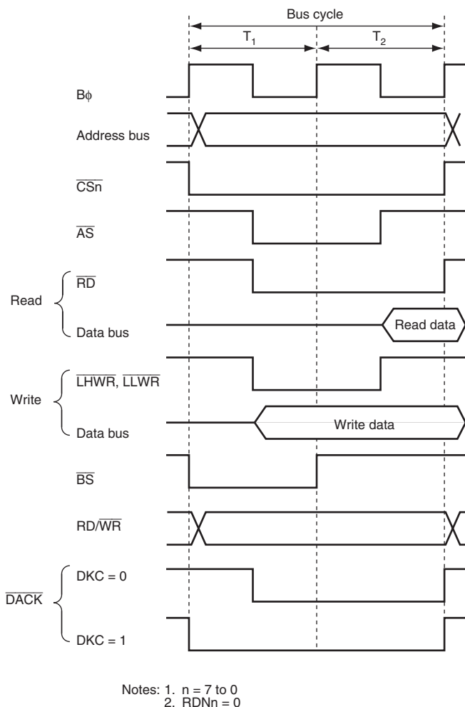
Figure 6.24 \overline{\text{DACK}} Signal Output Timing
