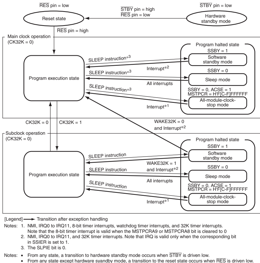
Figure 23.1 Mode Transitions
