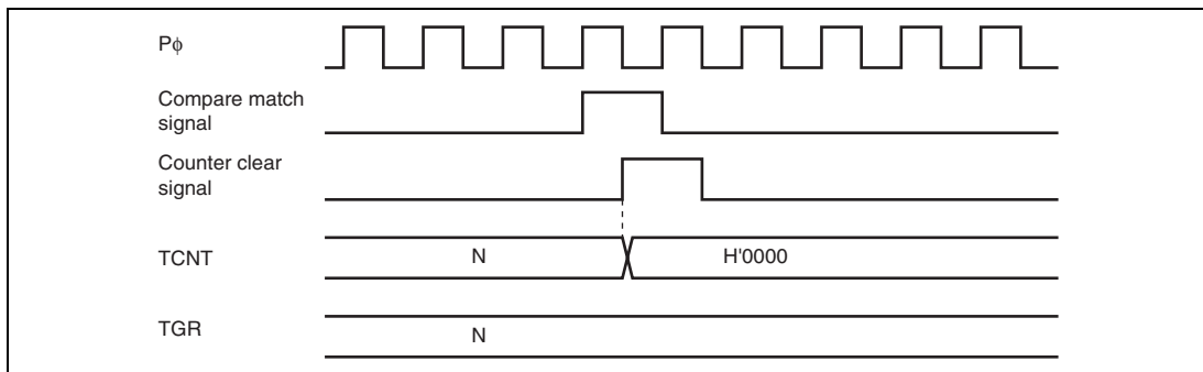
Figure 10.34 Counter Clear Timing (Compare Match)
