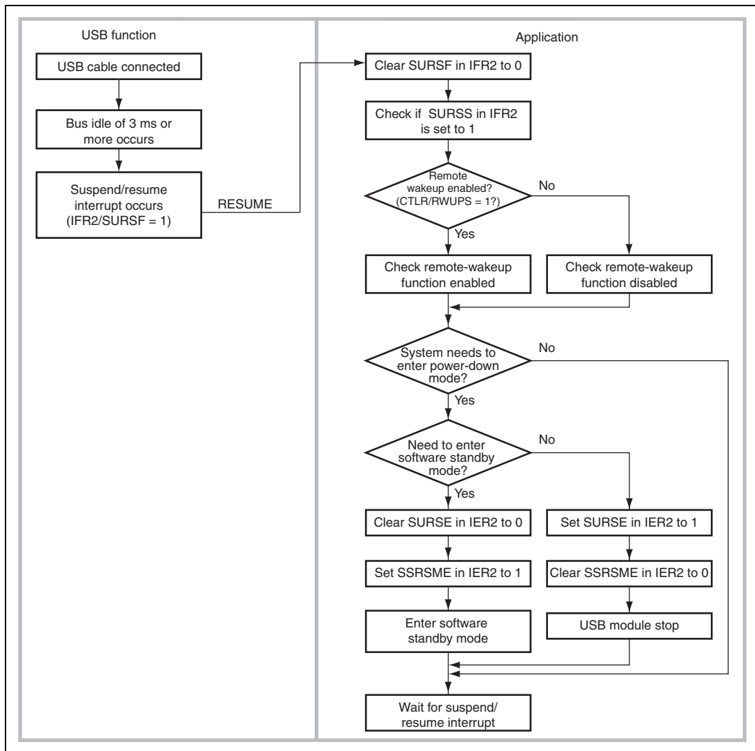
Figure 16.4 Suspend Operation
