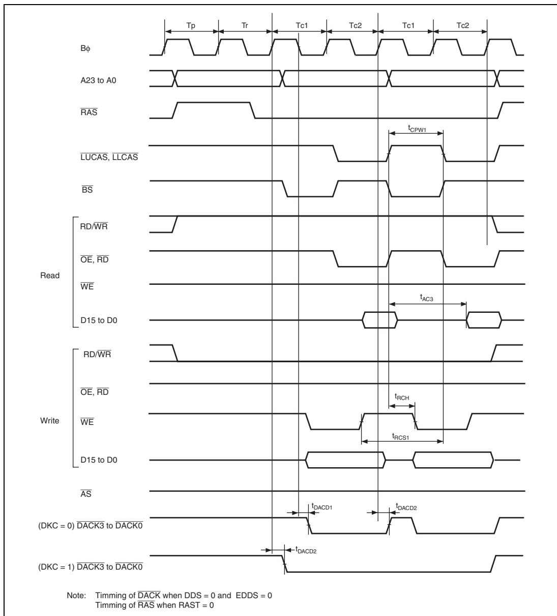
Figure 25.21 DRAM Access Timing: Two-State Burst Access
