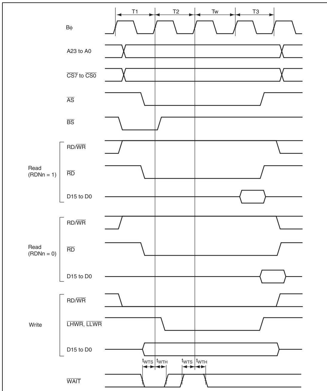
Figure 25.10 Basic Bus Timing: Three-State Access, One Wait
