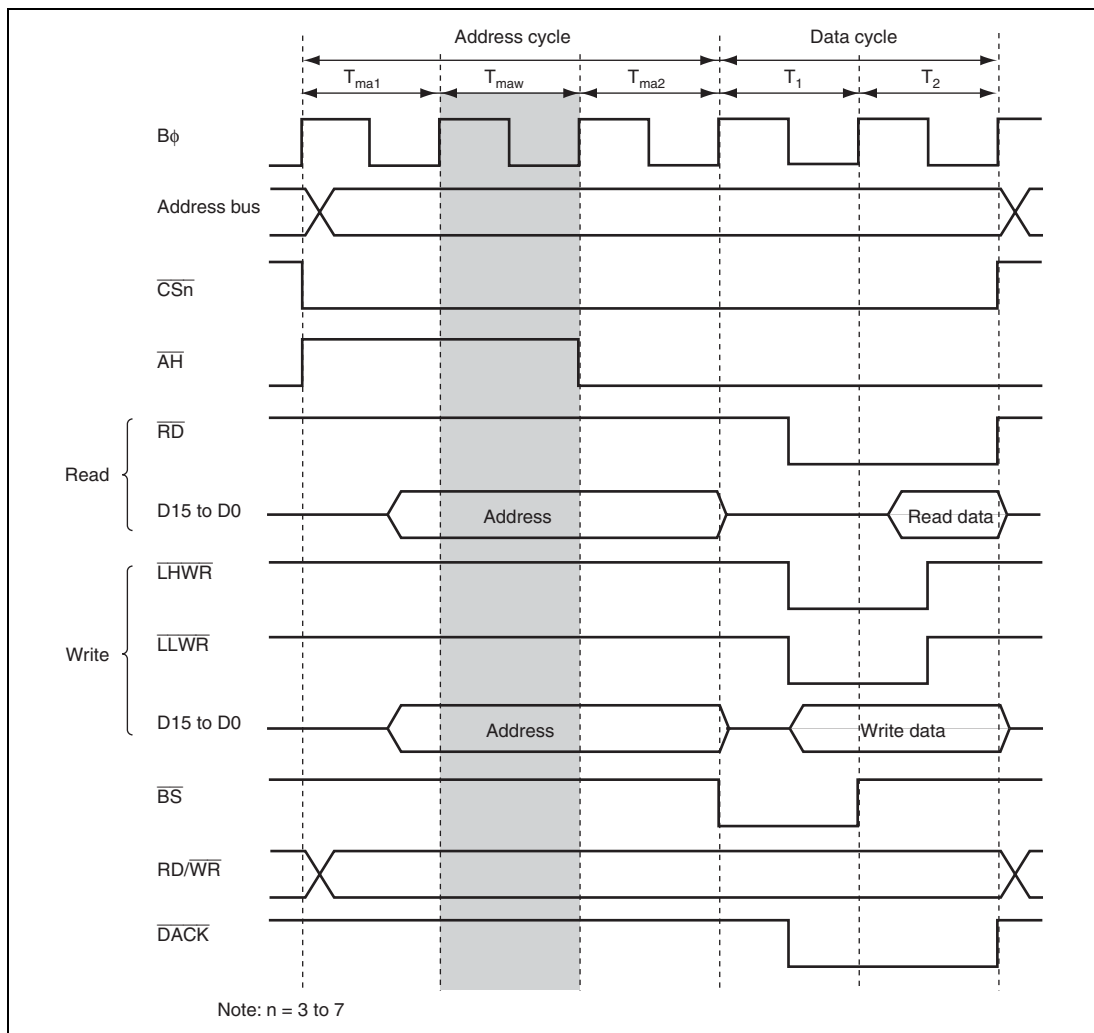
Figure 6.33 Access Timing of 3 Address Cycles (ADDEX = 1)
