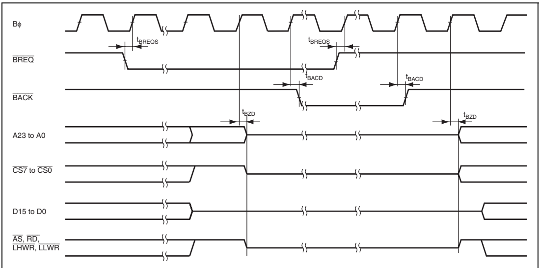
Figure 25.33 External Bus Release Timing
