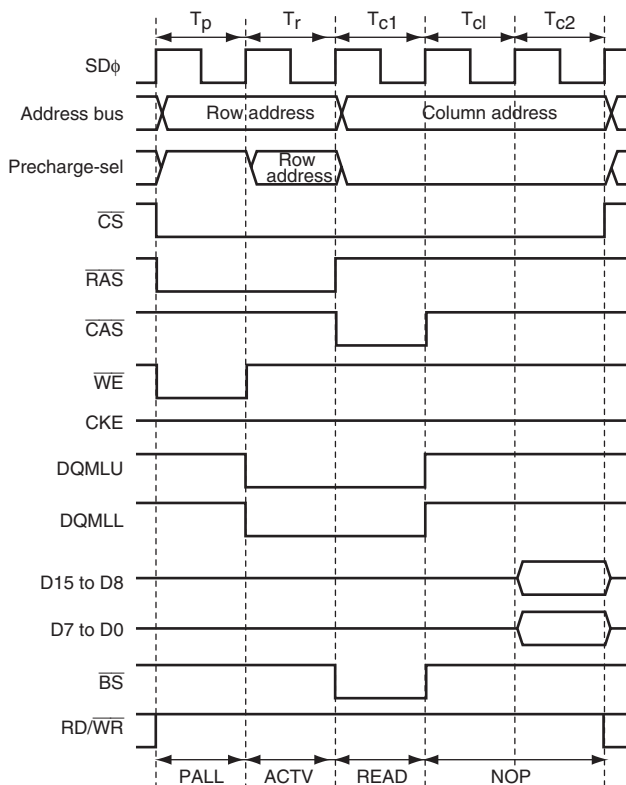
Figure 6.60 SDRAM Basic Read Access Timing (CAS Latency = 2)
