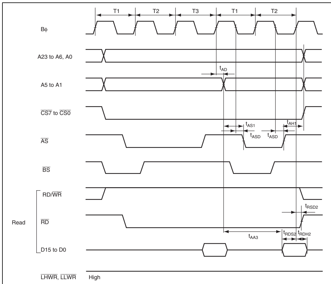
Figure 25.16 Burst ROM Access Timing: Two-State Burst Access
