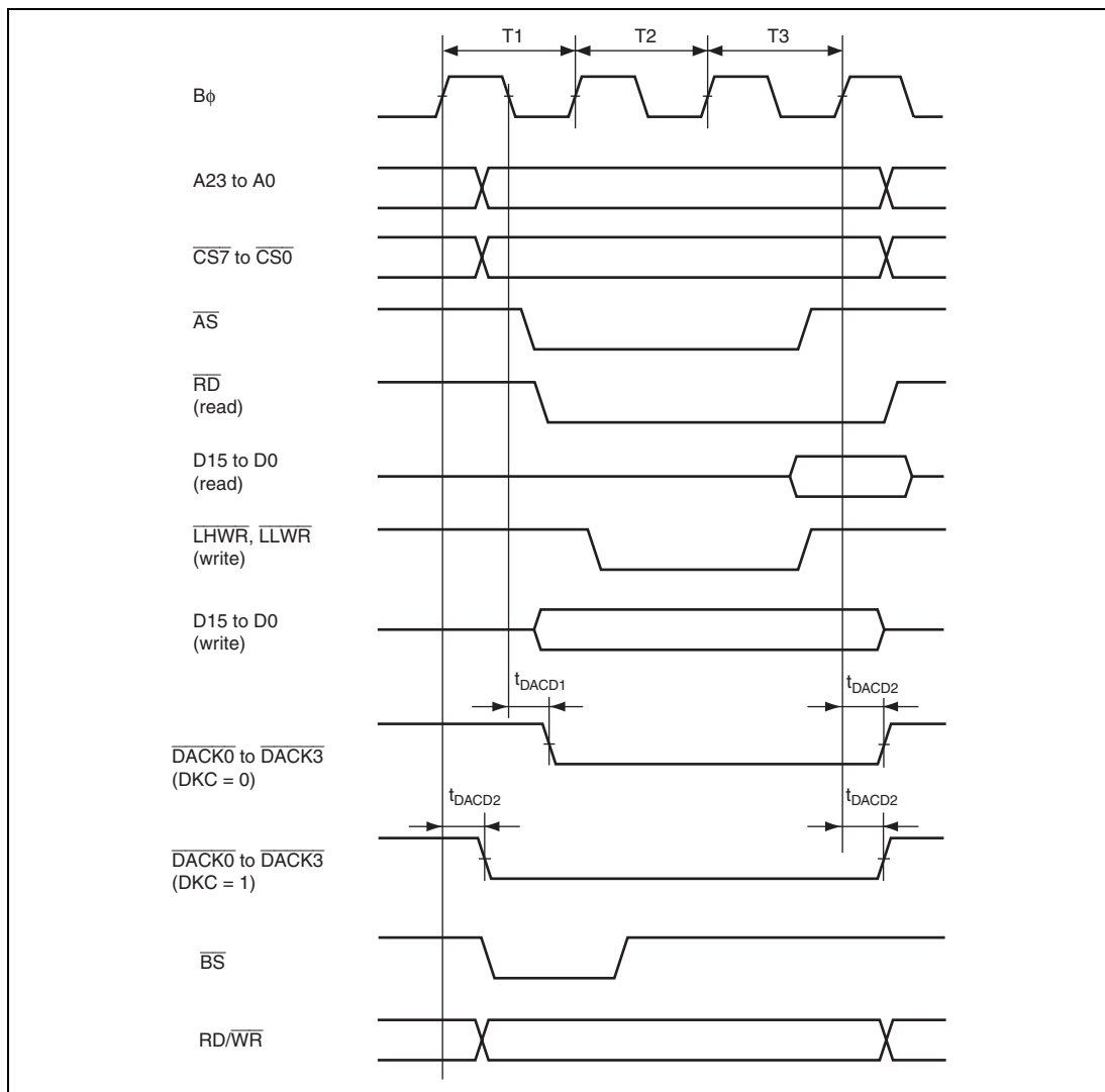
Figure 25.38 DMAC Single-Address Transfer Timing: Three-State Access
