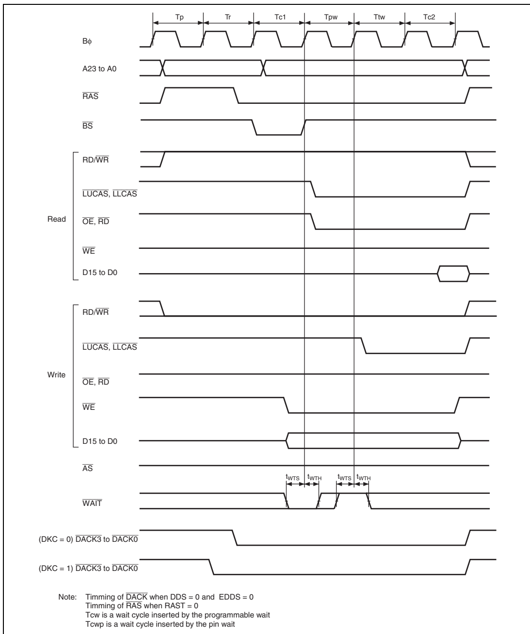
Figure 25.20 DRAM Access Timing: Two-State Access, One Wait
