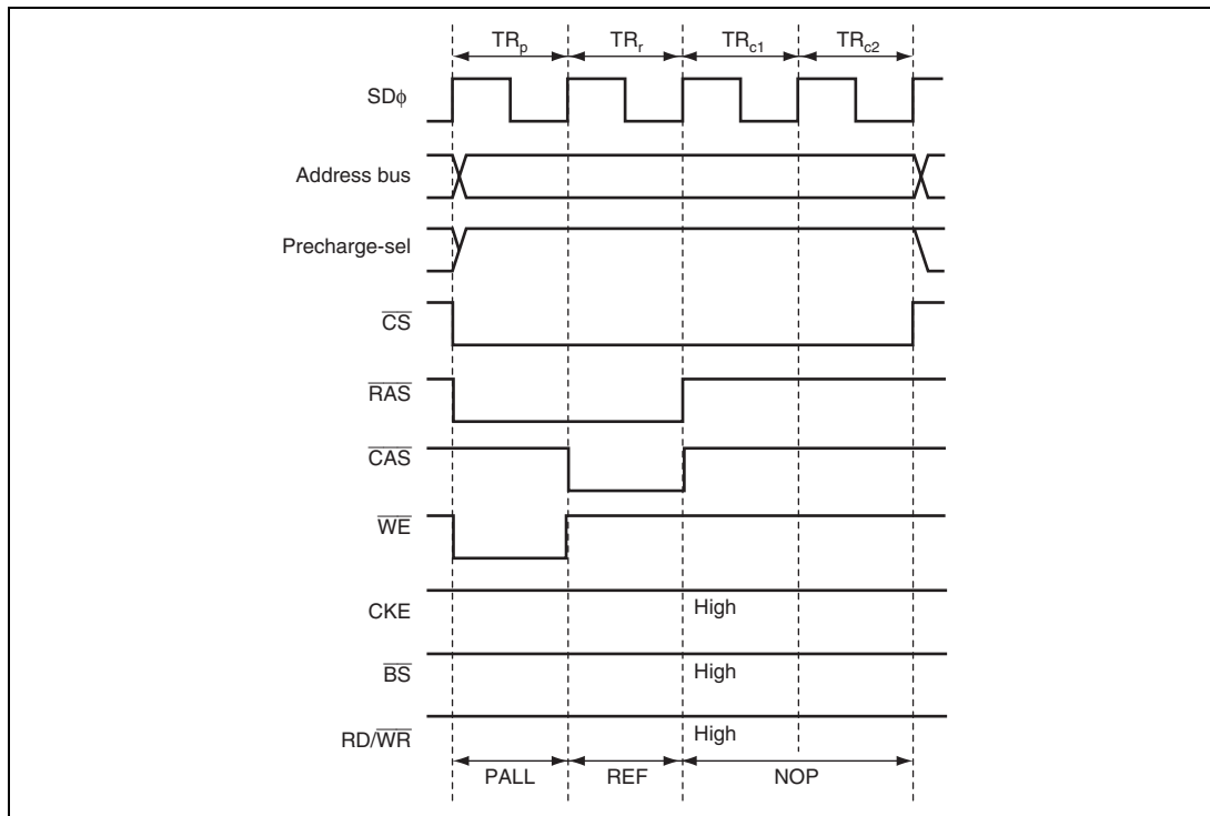
Figure 6.76 Auto-Refresh Operation
