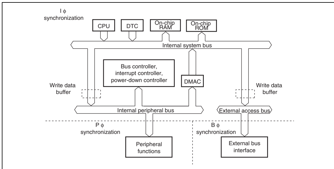
Figure 6.5 Internal Bus Configuration
