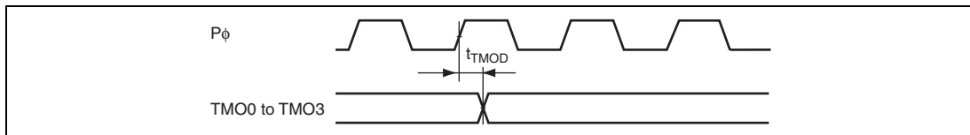
Figure 25.43 8-Bit Timer Output Timing
