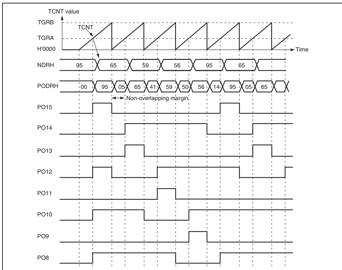
Figure 11.9 Non-Overlapping Pulse Output Example (4-Phase Complementary)
