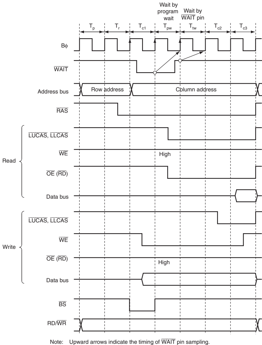
Figure 6.44 Example of Wait Cycle Insertion Timing for 3-Cycle Column Address Output
