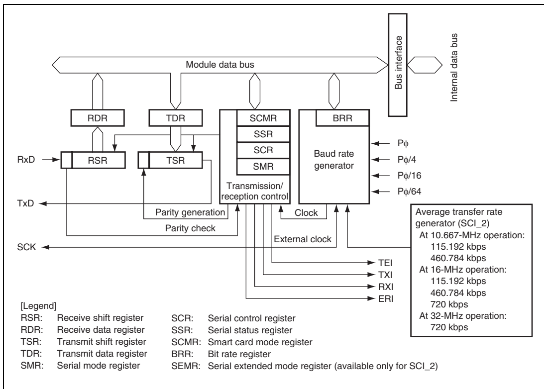
Figure 15.1 Block Diagram of SCI_0, 1, 2, and 4
