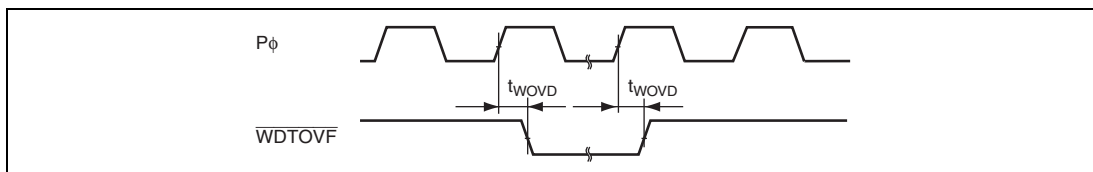
Figure 25.46 WDT Output Timing
