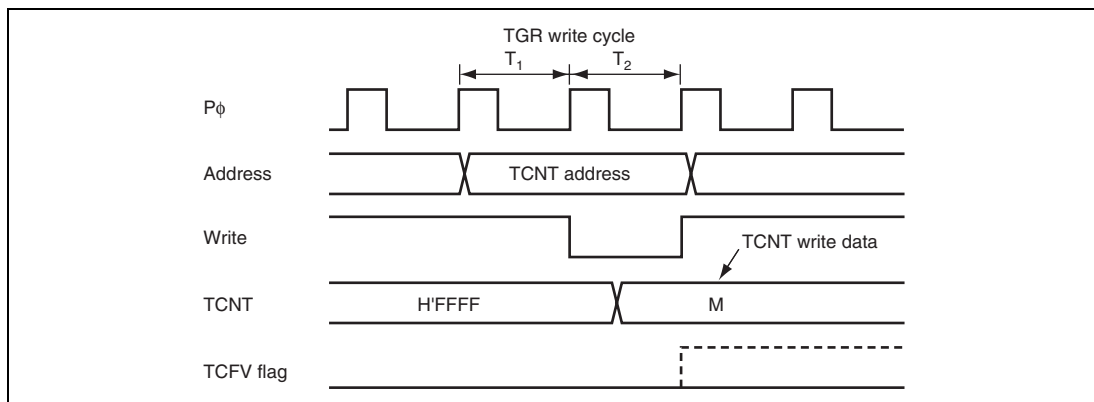
Figure 10.54 Conflict between TCNT Write and Overflow
