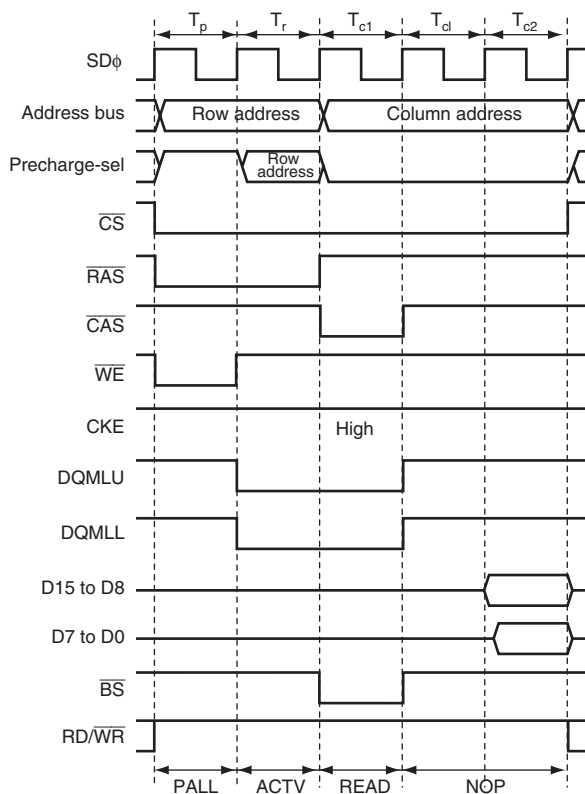
Figure 6.70 Control Timing Example of Word Control by DQM in 16-Bit Access Space (Read Access with Lowest Bit of Address = B'0, CAS Latency = 2)
