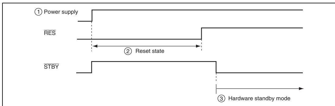
Figure 23.4 Timing Sequence at Power-On
