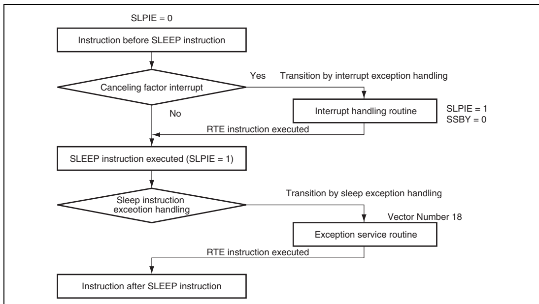
Figure 23.7 When Canceling Factor Interrupt is Generated Immediately before SLEEP Instruction Execution (Sleep Instruction Exception Handling Initiated)
