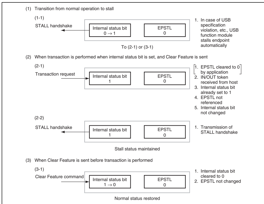
Figure 16.19 Automatic Stall by USB Function Module
