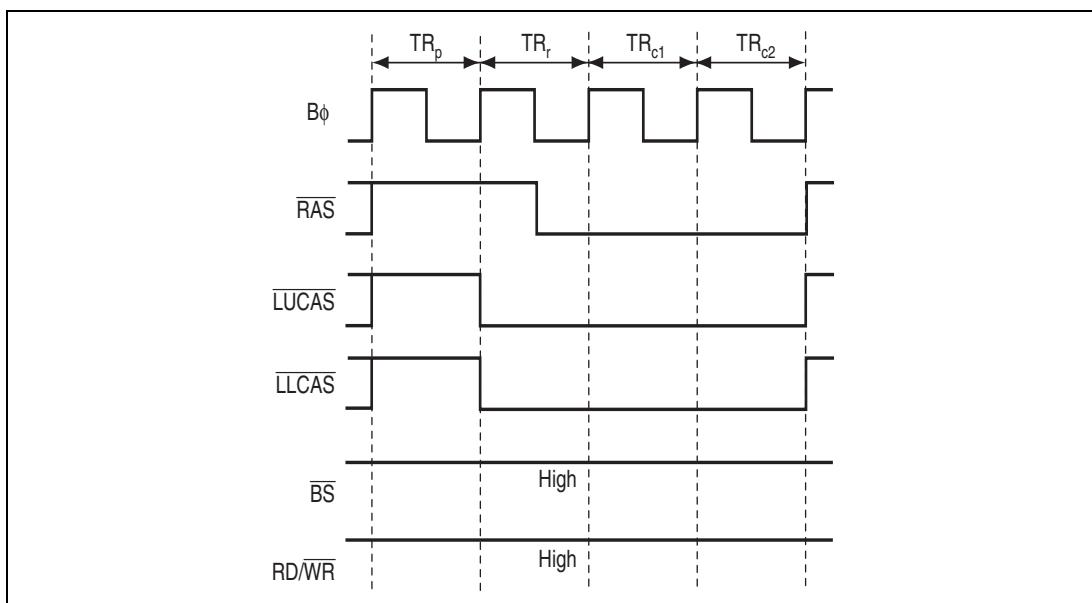
Figure 6.54 CBR Refresh Timing
