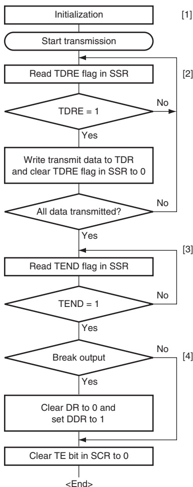
Figure 15.10 Example of Serial Transmission Flowchart
