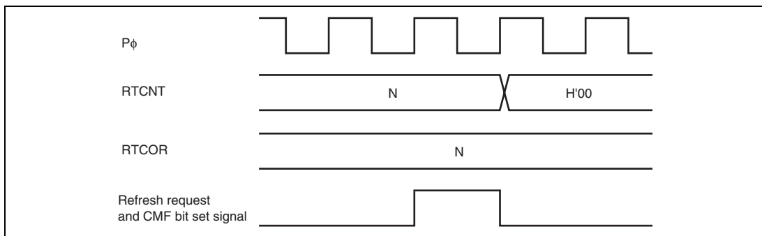
Figure 6.53 Compare Match Timing
