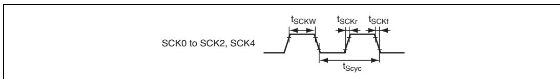
Figure 25.47 SCK Clock Input Timing
