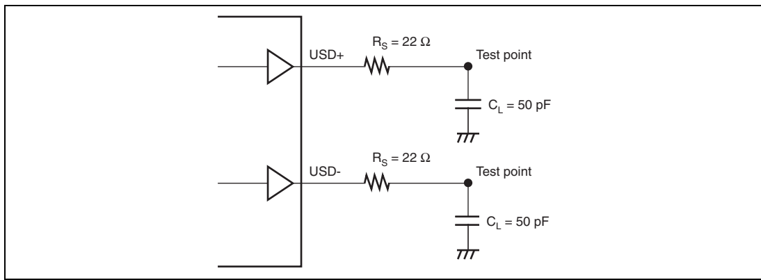
Figure 25.52 Load Condition
