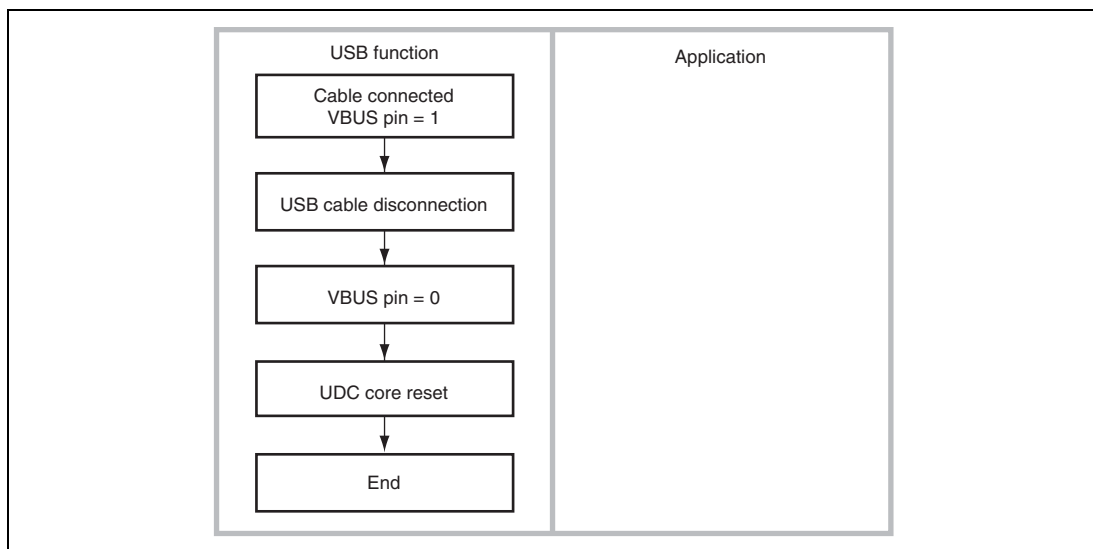
Figure 16.3 Cable Disconnection Operation
