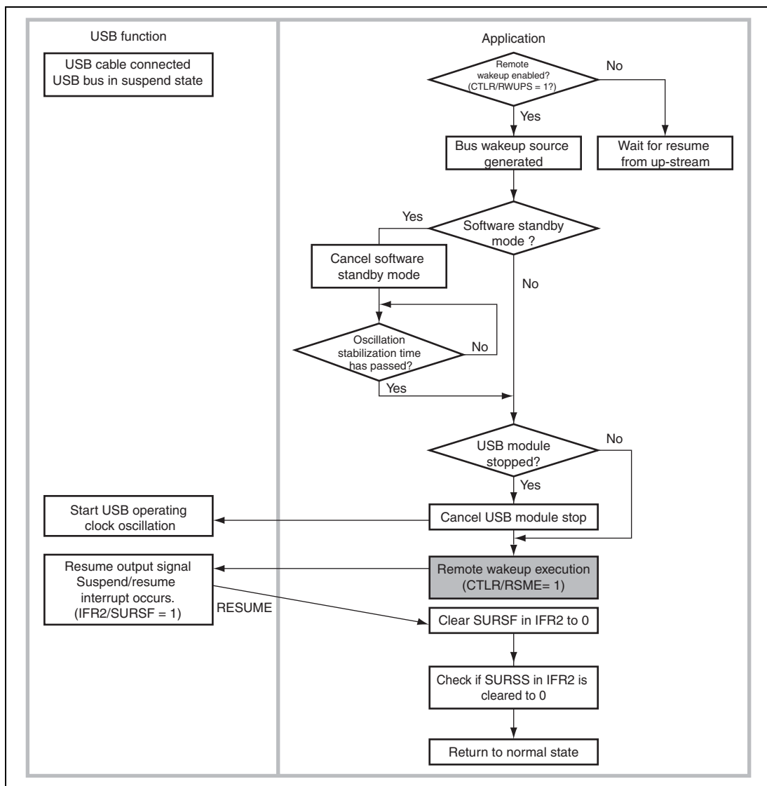
Figure 16.8 Remote-Wakeup
