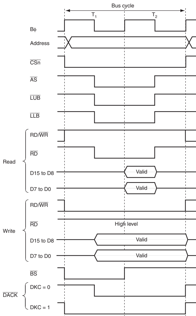
Figure 6.28 \overline{DACK} Signal Output Timing
