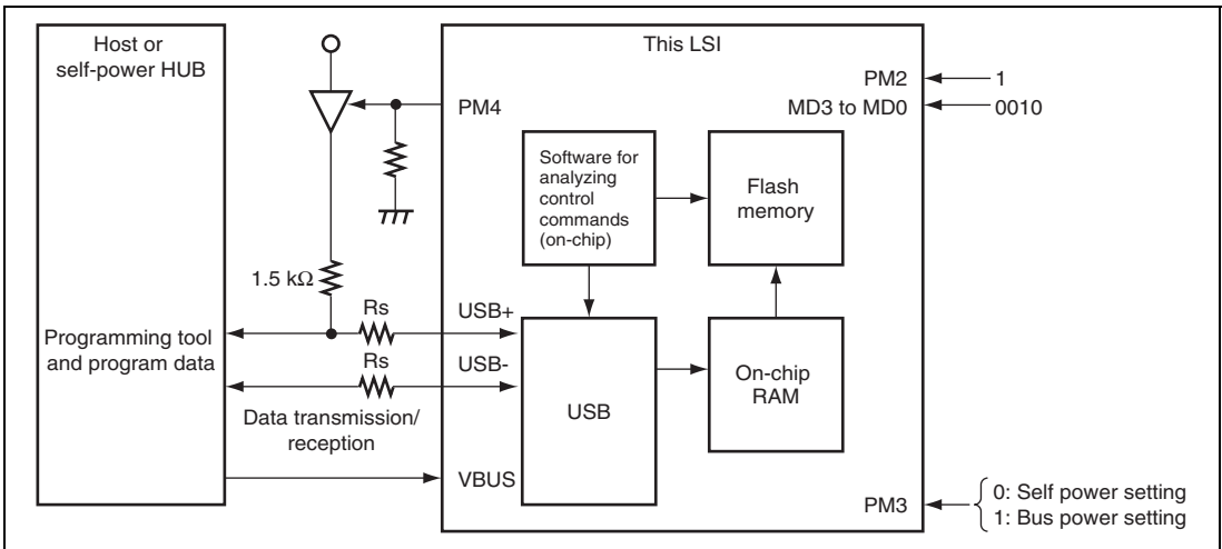
Figure 21.9 System Configuration in USB Boot Mode
