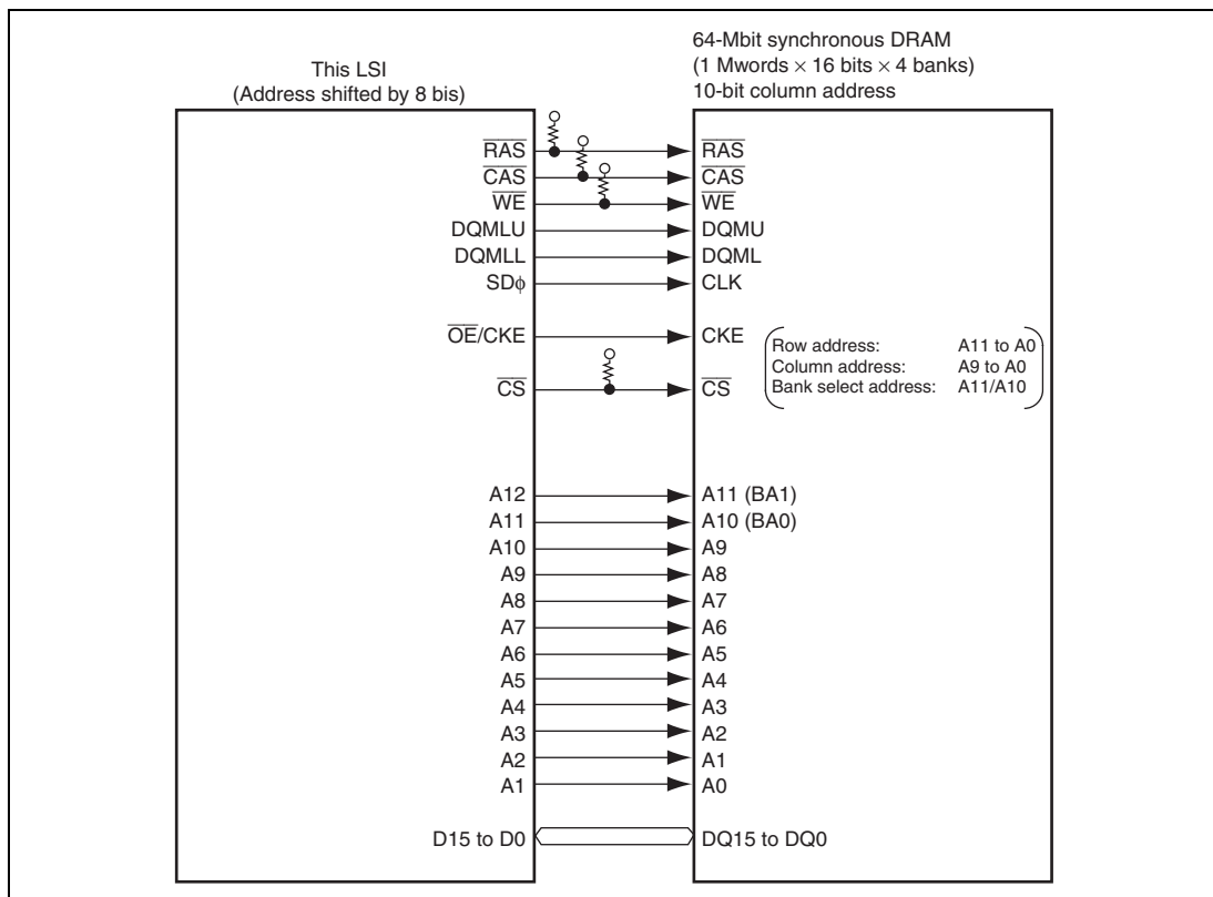
Figure 6.71 Connection Example of DQM Byte/Word Control
