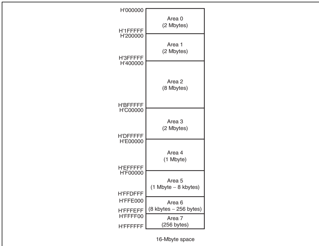
Figure 6.8 Address Space Area Division
