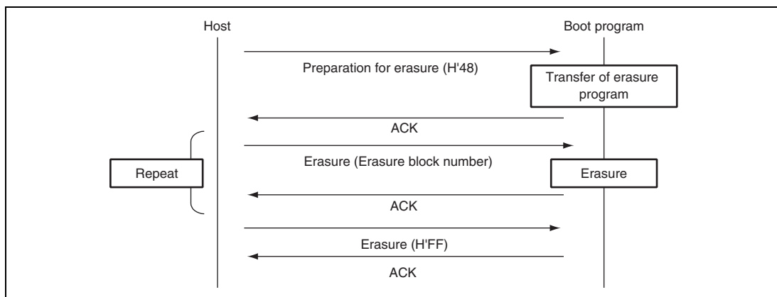
Figure 21.25 Erasure Sequence
