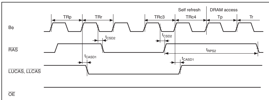
Figure 25.27 Self-Refresh Timing (After Leaving Software Standby: RAS\bar{T} = 0 )
