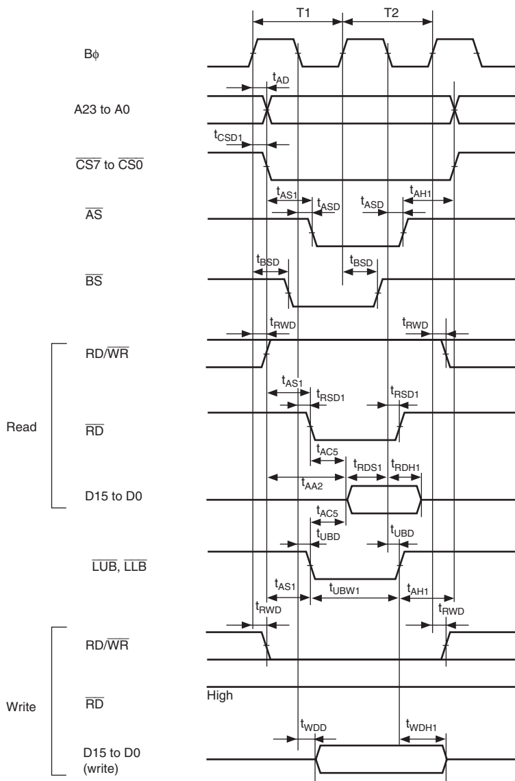
Figure 25.13 Byte Control SRAM: Two-State Read/Write Access
