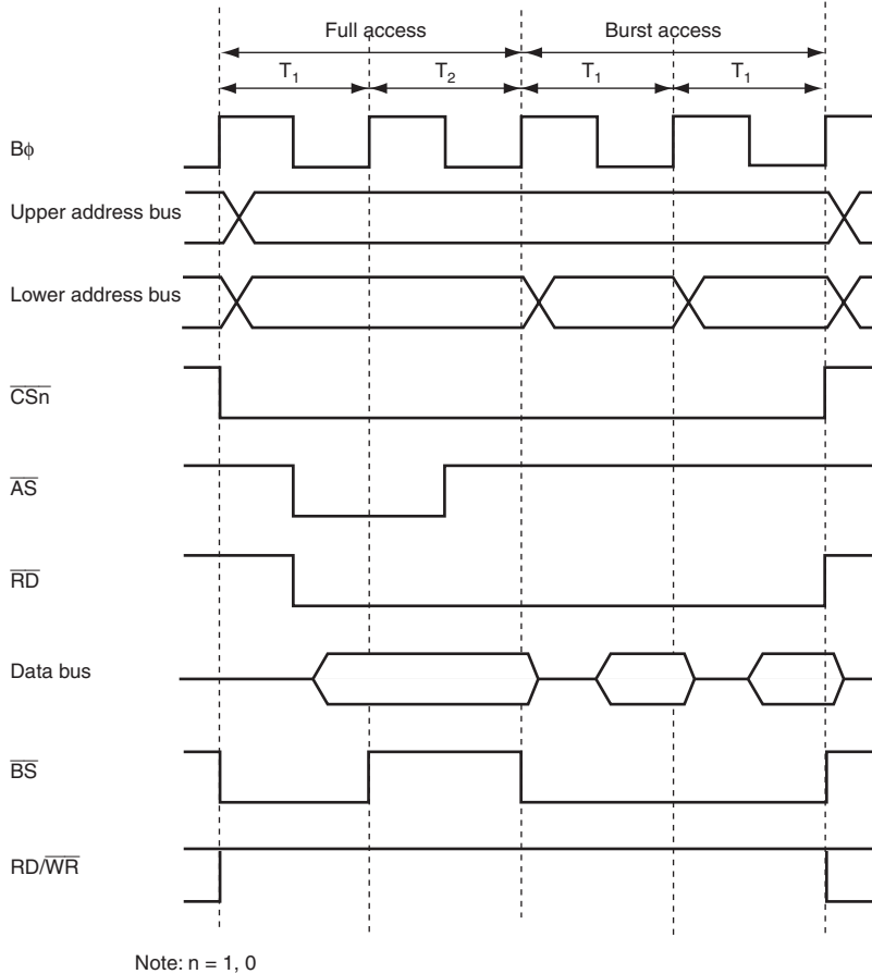
Figure 6.30 Example of Burst ROM Access Timing ( ASTn = 0 , One Burst Cycle)
