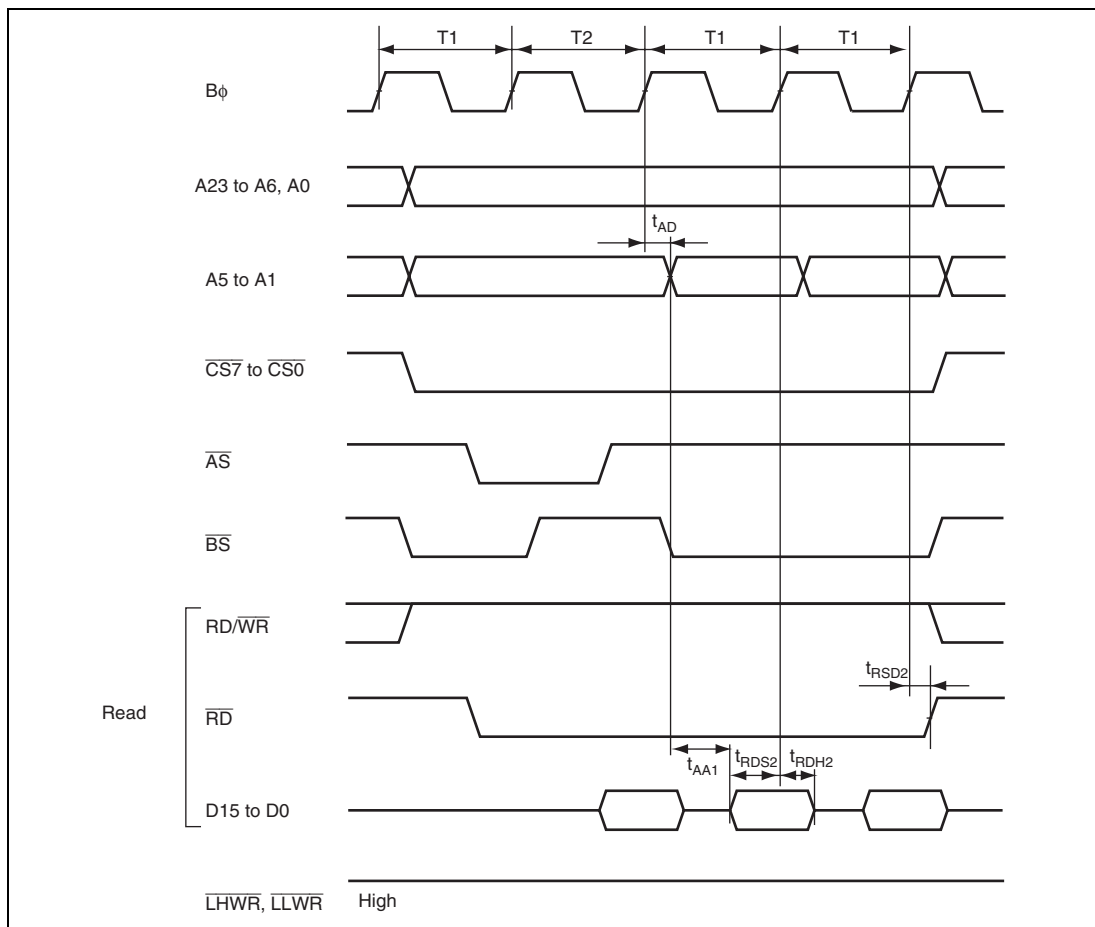
Figure 25.15 Burst ROM Access Timing: One-State Burst Access
