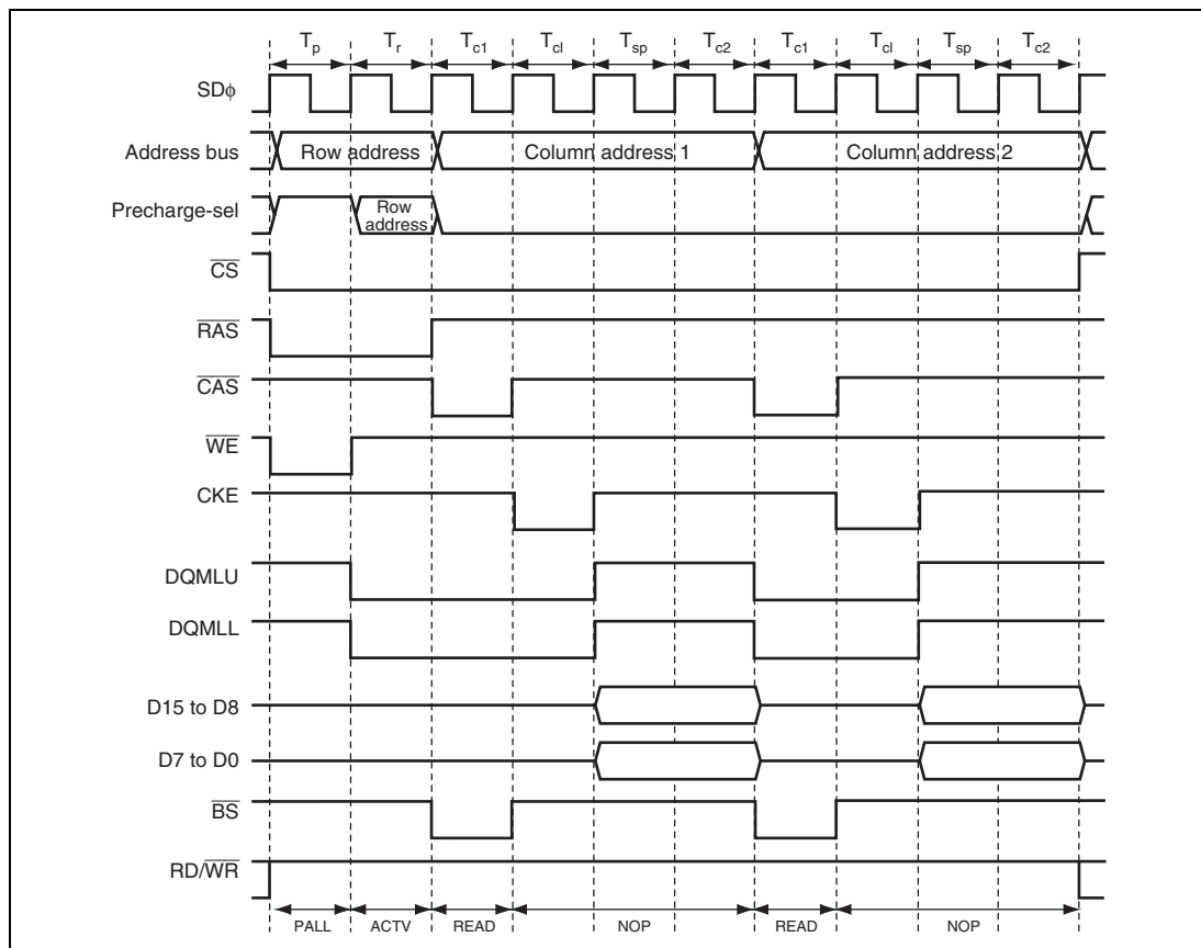
Figure 6.67 Read Timing Example when CKSPE = 1 (CAS Latency = 2)
