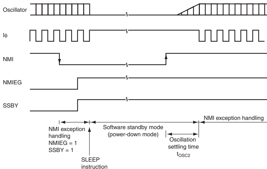
Figure 25.3 Oscillation Settling Timing after Software Standby Mode
