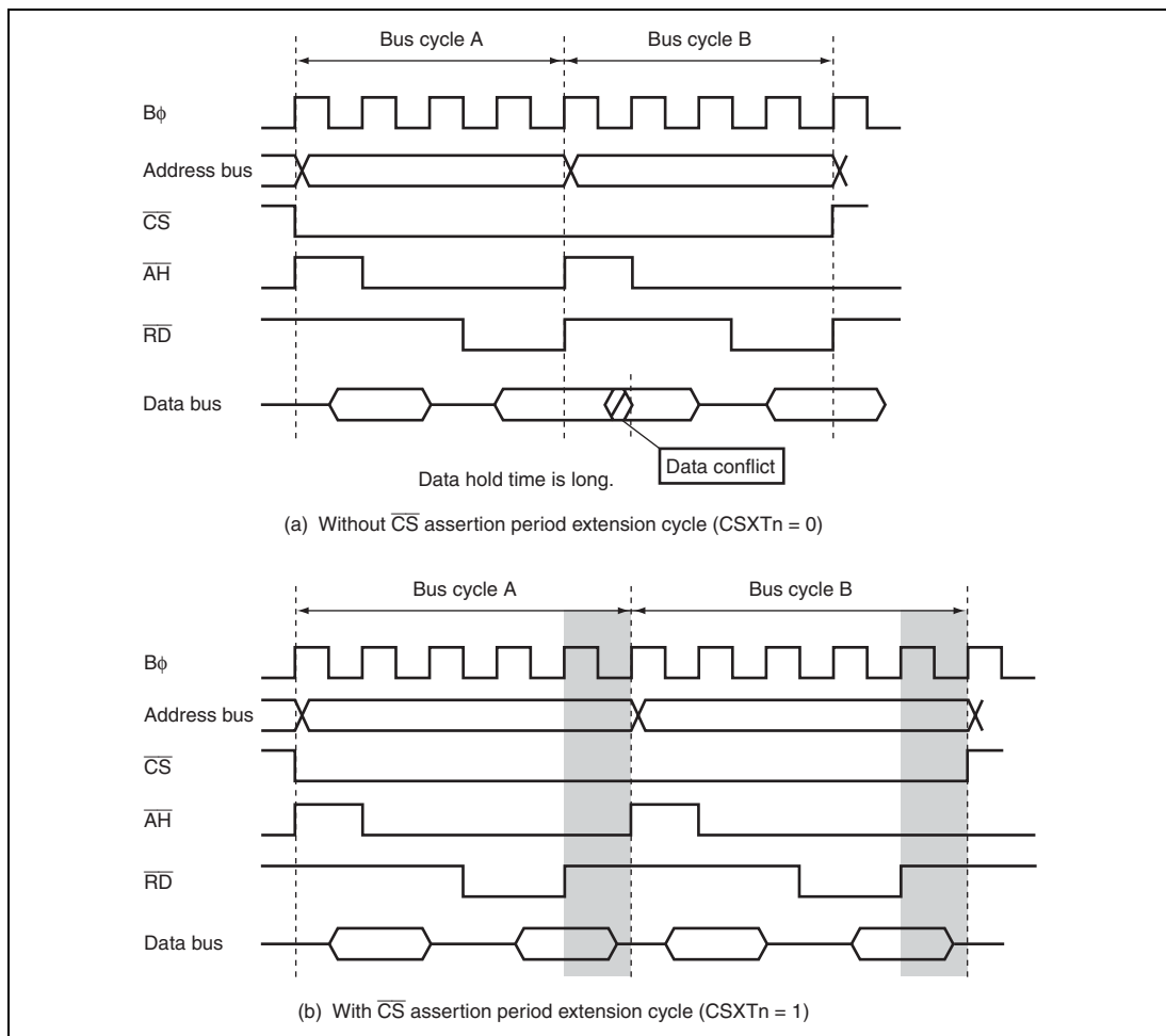
Figure 6.36 Consecutive Read Accesses to Same Area (Address/Data Multiplexed I/O Space)
