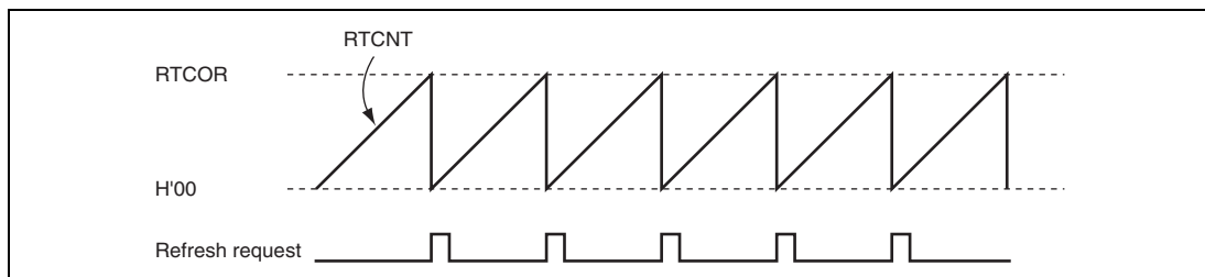
Figure 6.52 RTCNT Operation
