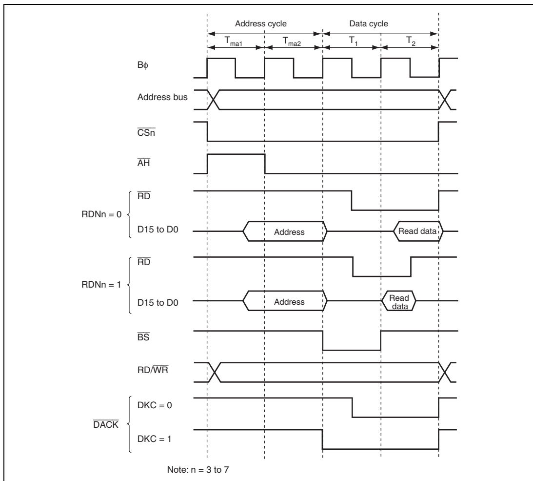
Figure 6.37 \overline{\text{DACK}} Signal Output Timing
