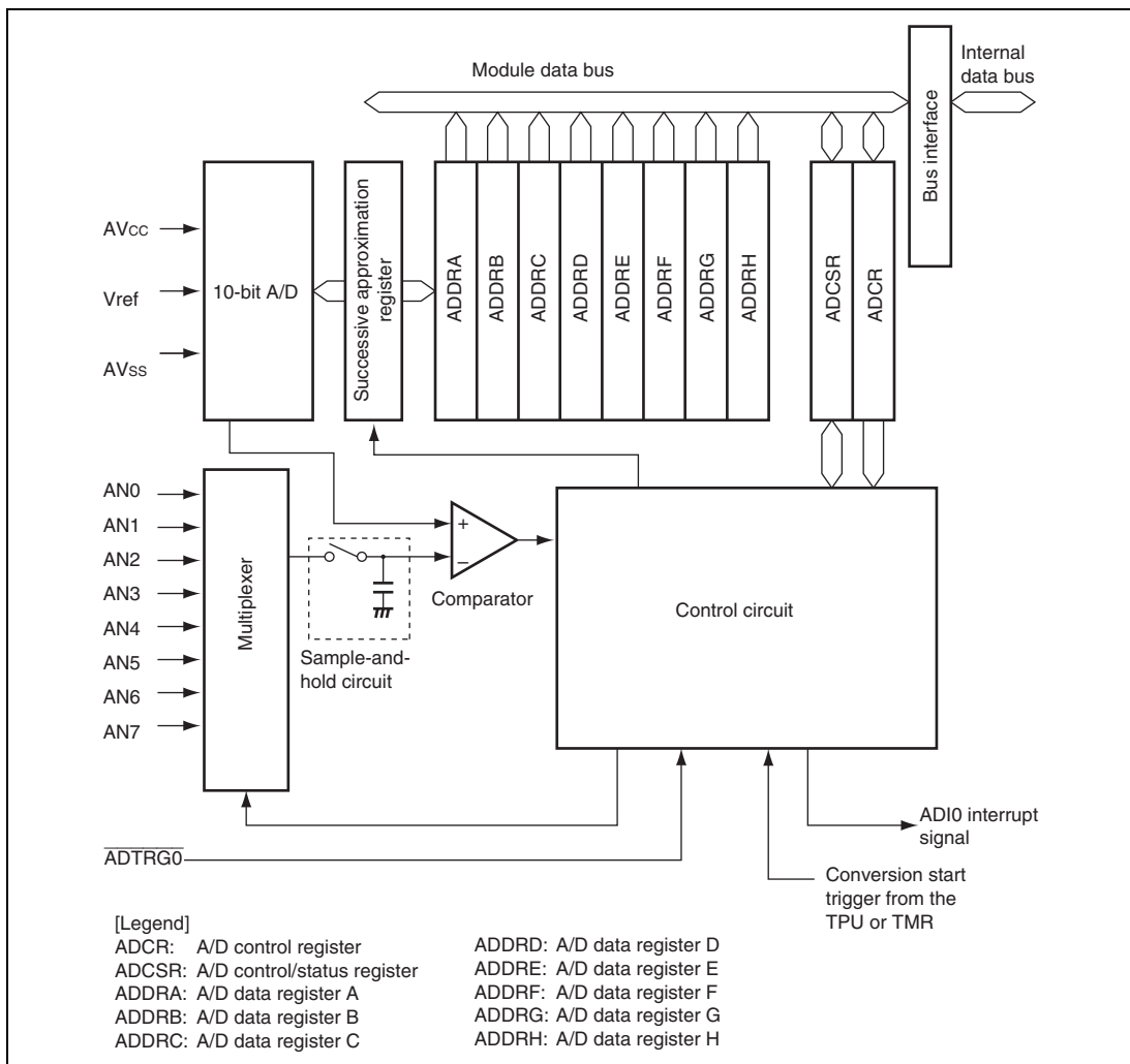
Figure 18.1 Block Diagram of A/D Converter
