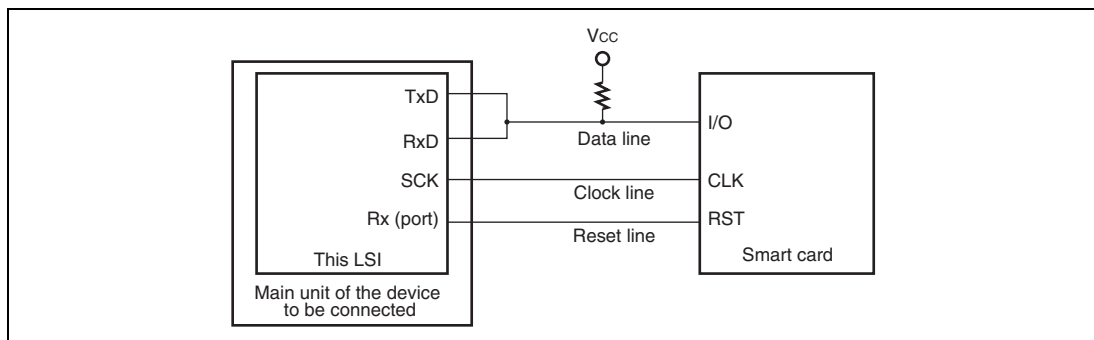
Figure 15.24 Pin Connection for Smart Card Interface
