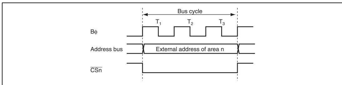
Figure 6.9 \overline{CSn} Signal Output Timing ( n = 0 to 7)
