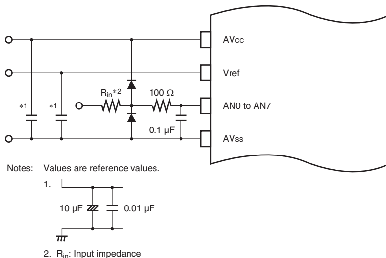
Figure 18.9 Example of Analog Input Protection Circuit
