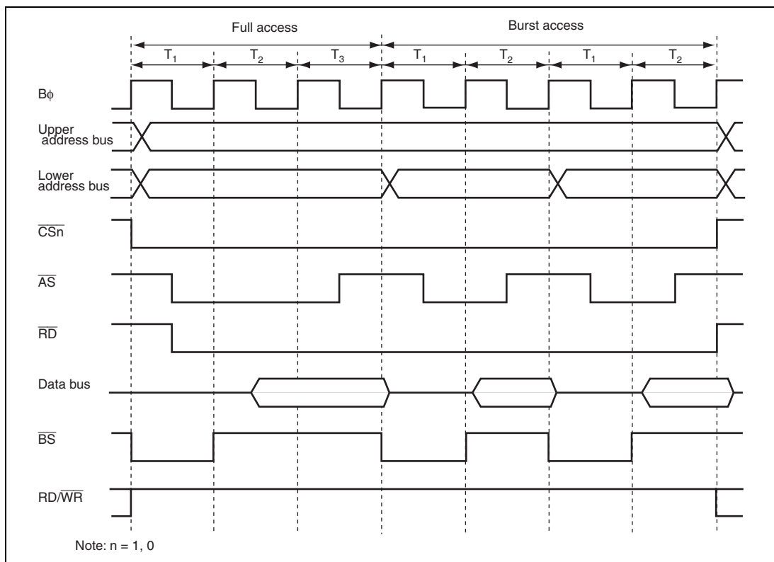
Figure 6.29 Example of Burst ROM Access Timing (AST n = 1, Two Burst Cycles)
