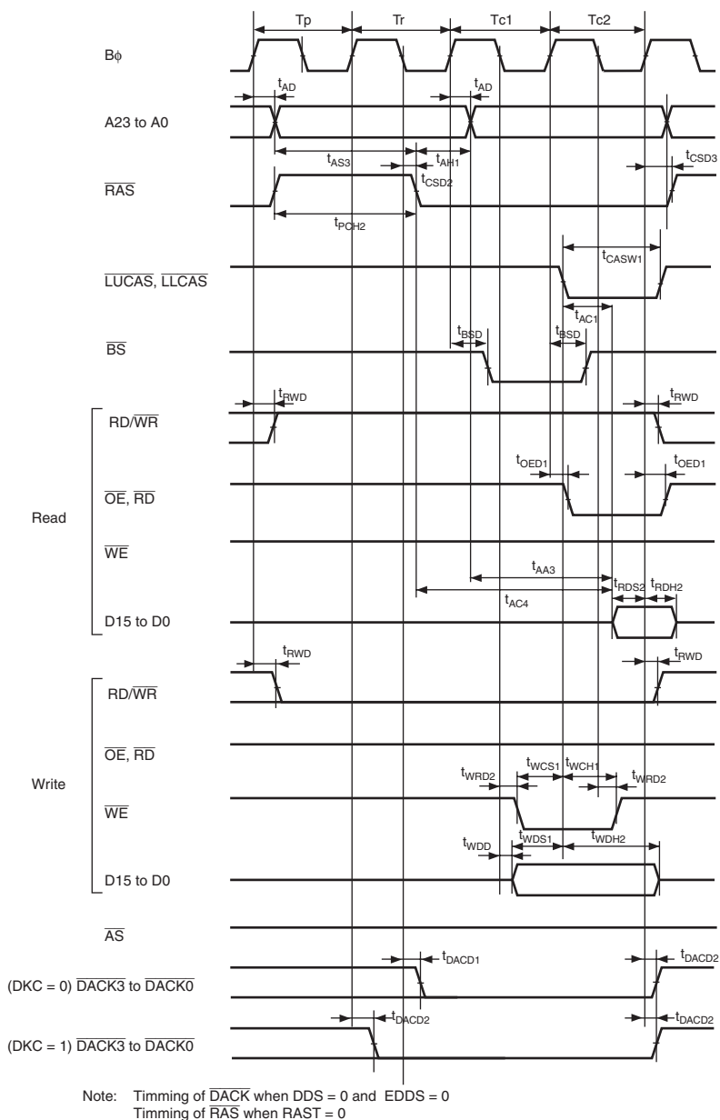
Figure 25.19 DRAM Access Timing: Two-State Access
