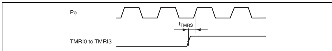
Figure 25.44 8-Bit Timer Reset Input Timing
