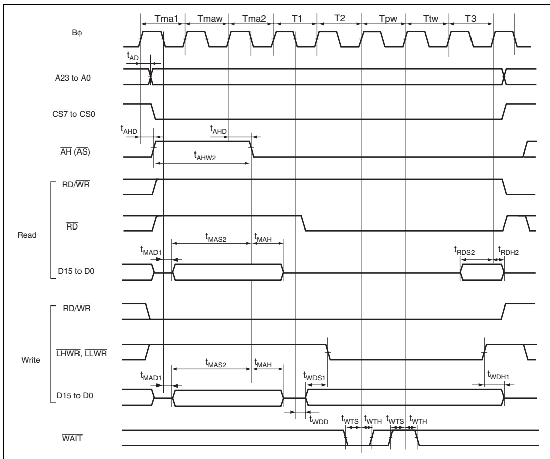
Figure 25.18 Address/Data Multiplexed Access Timing (Wait Control) (Address Cycle Program Wait \times 1 + Data Cycle Program Wait \times 1 + Data Cycle Pin Wait \times 1)
