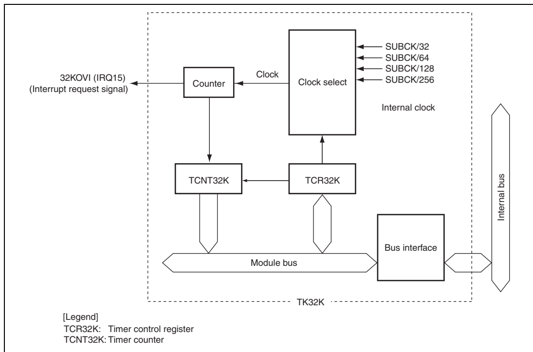
Figure 13.1 Block Diagram of TM32K
