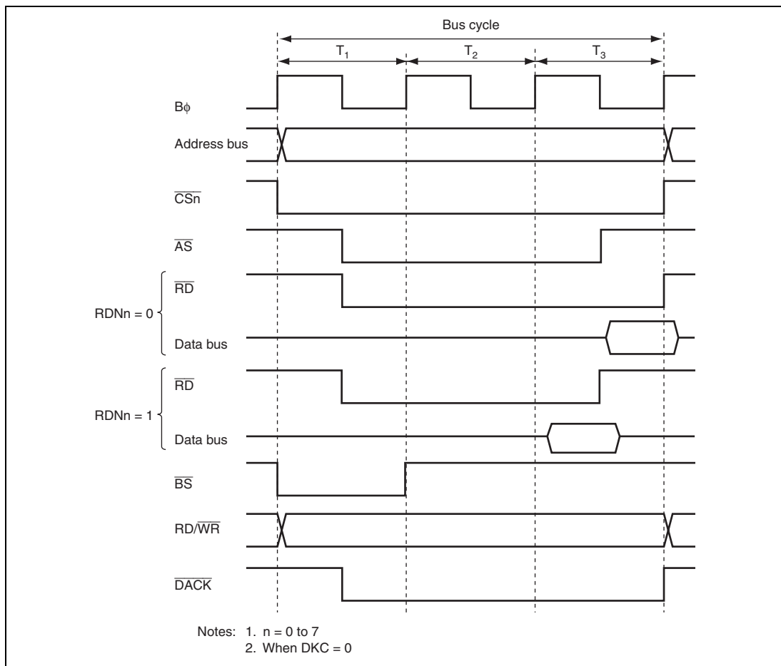
Figure 6.22 Example of Read Strobe Timing
