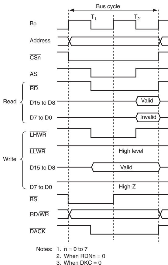
Figure 6.15 16-Bit 2-State Access Space Bus Timing (Byte Access for Even Address)
