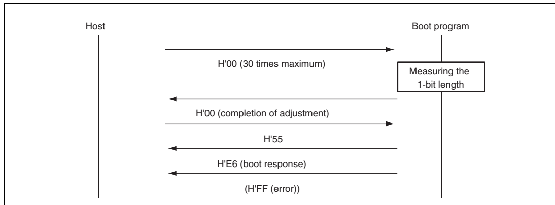
Figure 21.21 Bit-Rate-Adjustment Sequence
