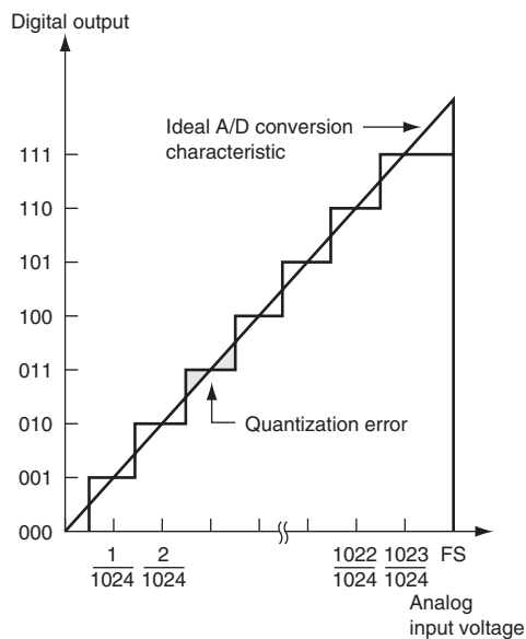
Figure 18.6 A/D Conversion Accuracy Definitions
