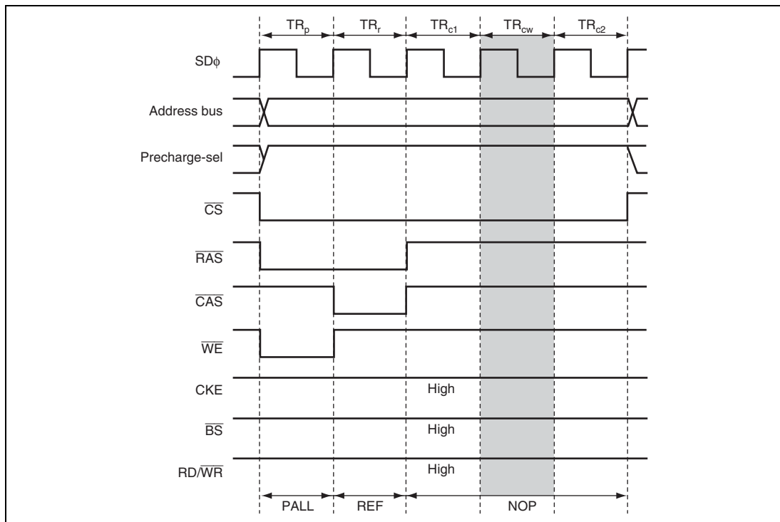
Figure 6.78 Auto-Refresh Timing (TPC1 = 0, TPC0 = 0, RLW2 = 0, RLW1 = 0, RLW0 = 1)
