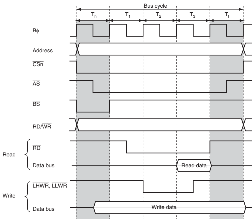
Figure 6.3 \overline{CS} and Address Assertion Period Extension (Example of Basic Bus Interface, 3-State Access Space, and RDNn = 0 )
