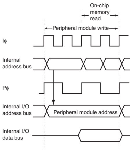
Figure 6.102 Example of Timing when Peripheral Module Write Data Buffer Function is Used
