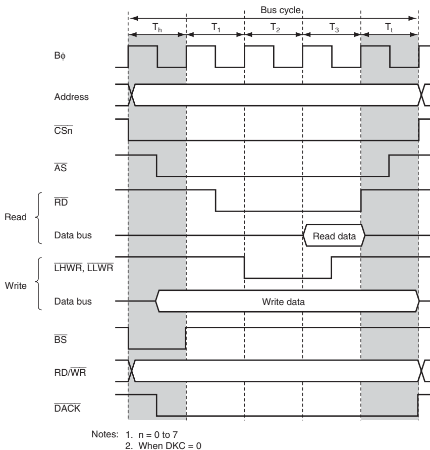
Figure 6.23 Example of Timing when Chip Select Assertion Period is Extended
