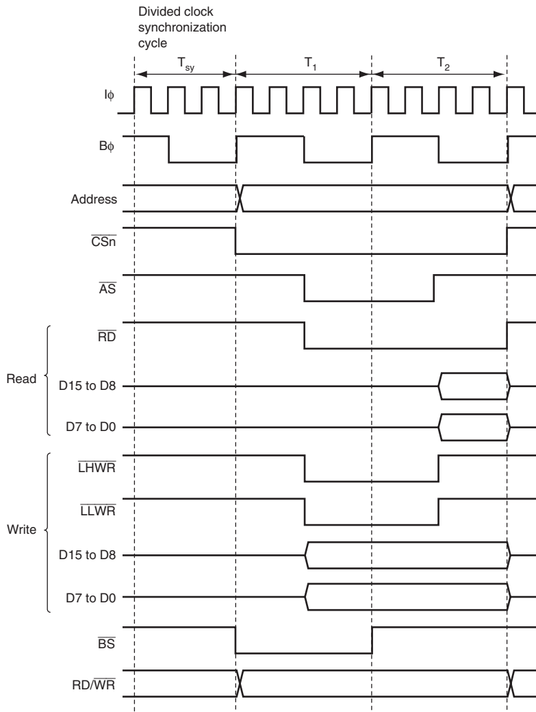
Figure 6.6 System Clock: External Bus Clock = 4:1, External 2-State Access
