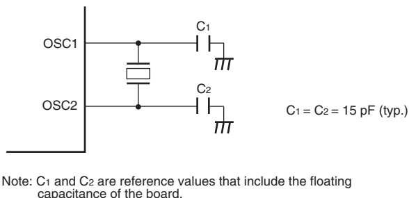
Figure 22.6 Connection Example of 32.768-kHz Crystal Resonator
