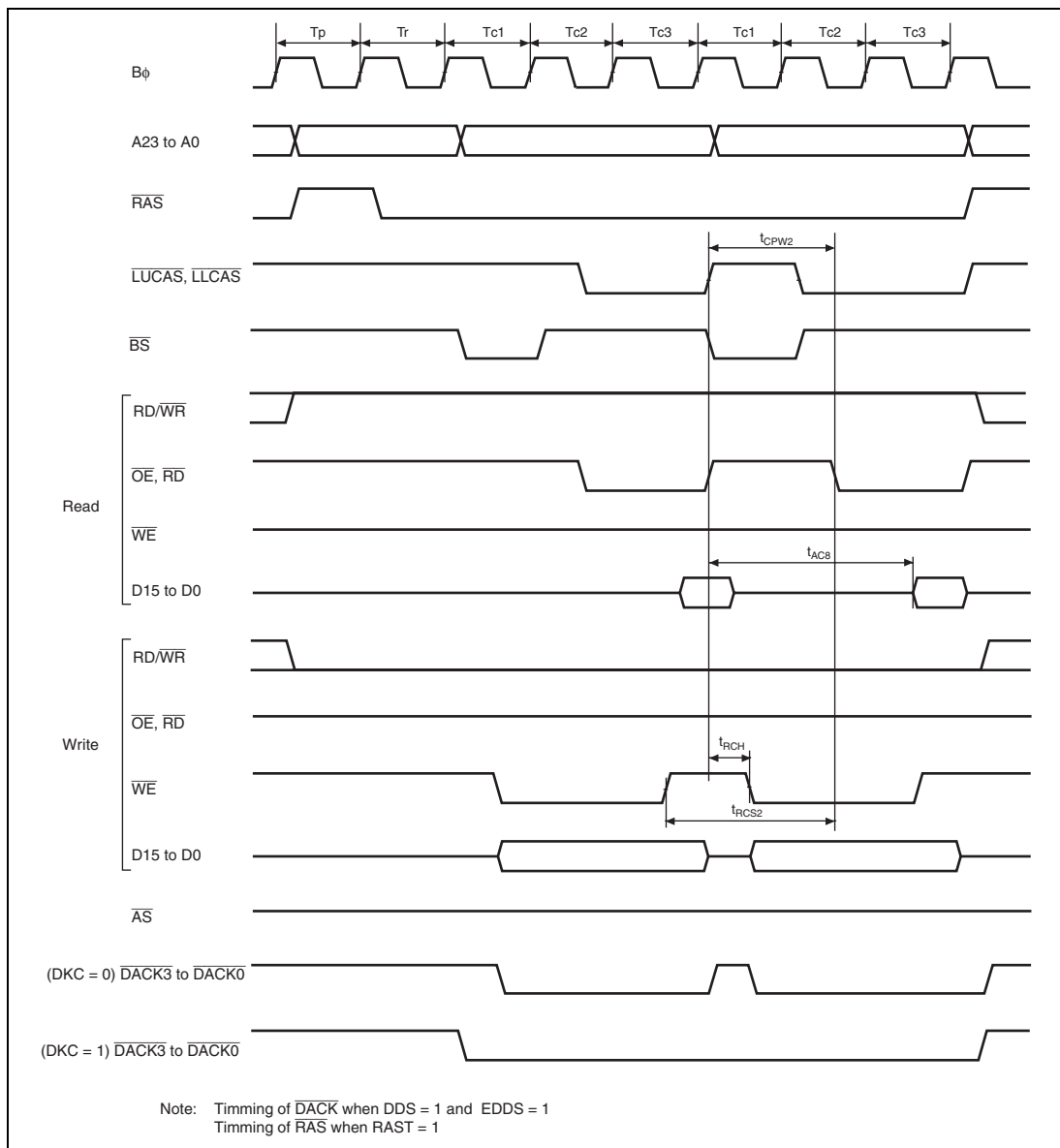
Figure 25.24 DRAM Access Timing: Three-State Burst Access
