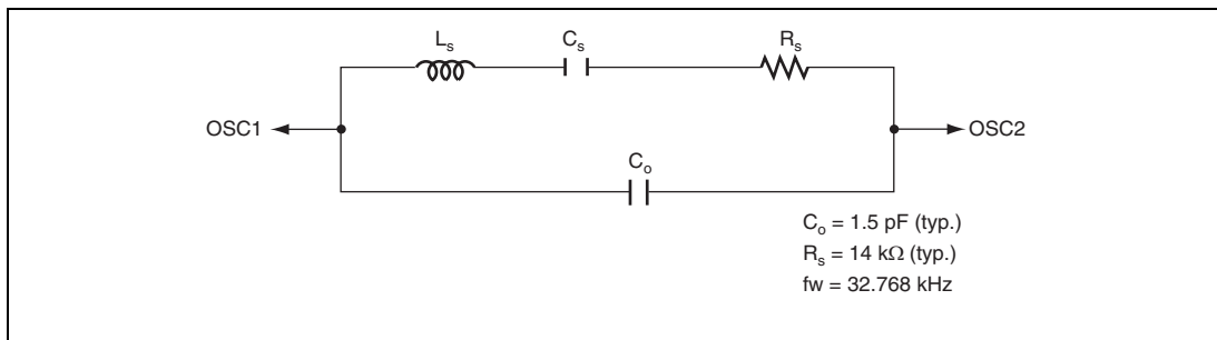
Figure 22.7 Equivalent Circuit for 32.768-kHz Crystal Resonator
