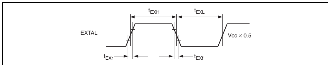
Figure 25.5 External Input Clock Timing
