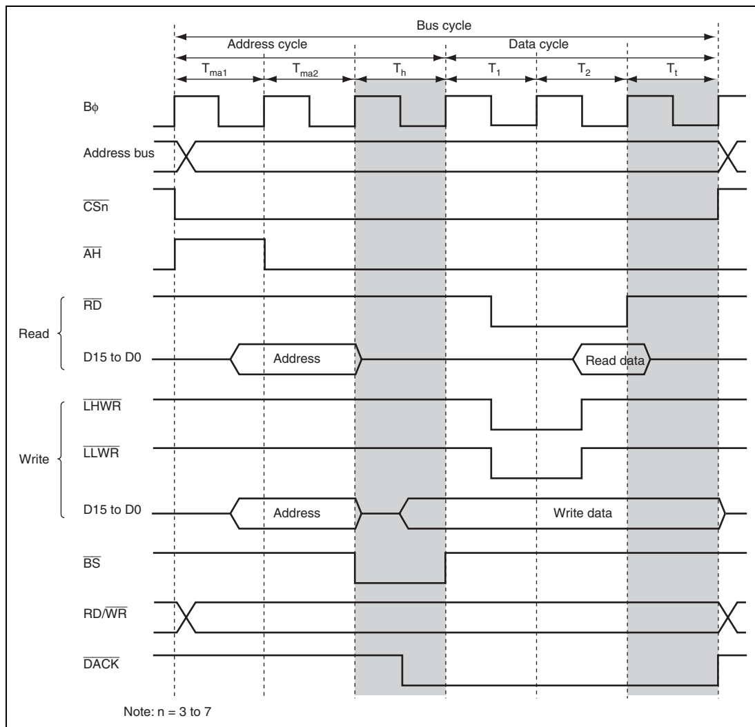
Figure 6.35 Chip Select ( \overline{\text{CS}} ) Assertion Period Extension Timing in Data Cycle
