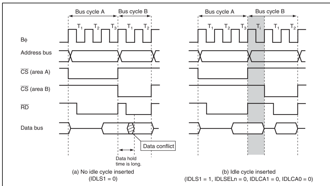
Figure 6.90 Example of Idle Cycle Operation (Consecutive Reads in Different Areas)
