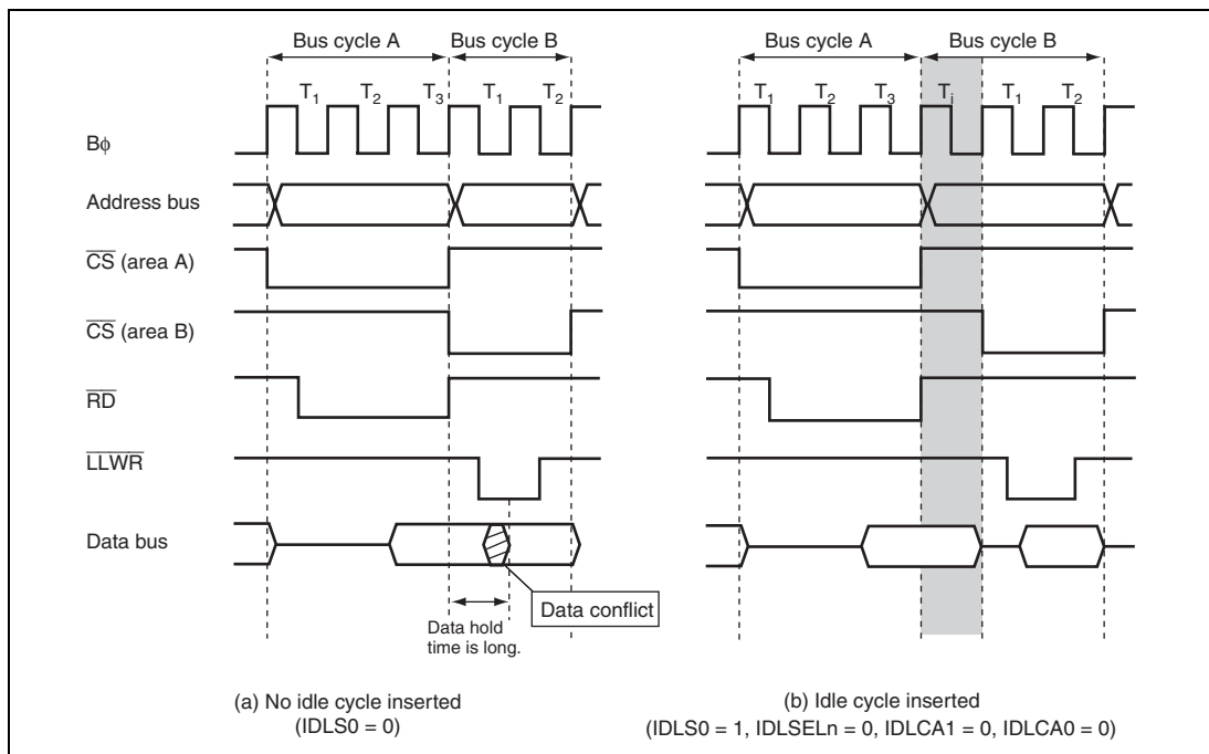
Figure 6.91 Example of Idle Cycle Operation (Write after Read)
