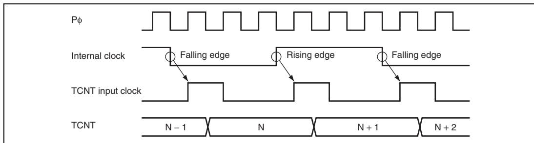
Figure 10.30 Count Timing in Internal Clock Operation
