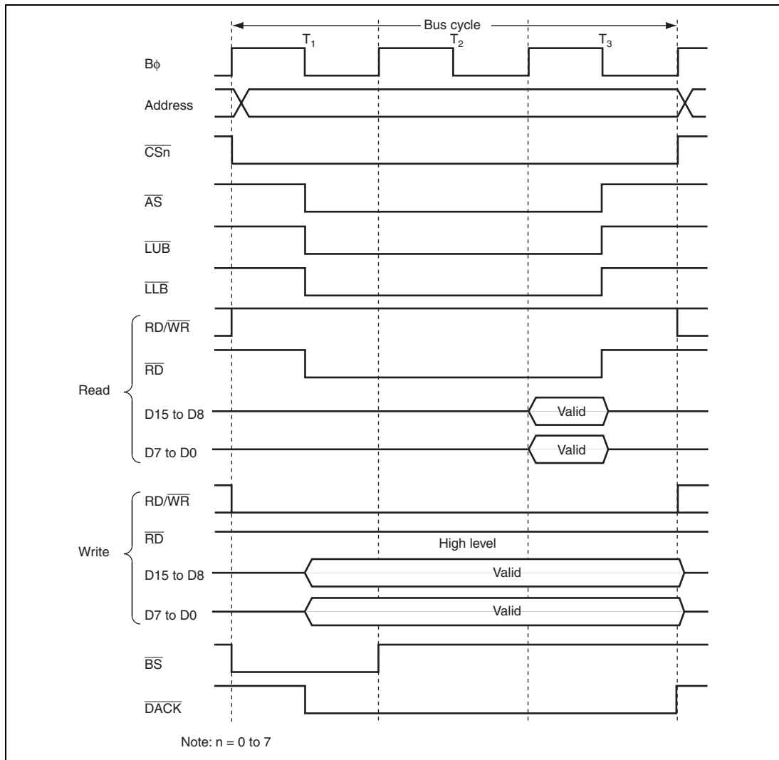
Figure 6.26 16-Bit 3-State Access Space Bus Timing
