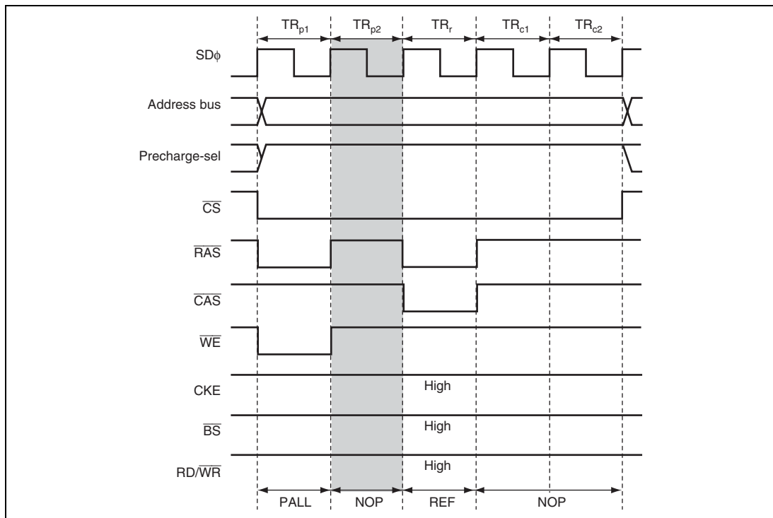
Figure 6.77 Auto-Refresh Timing (TPC1 = 0, TPC0 = 1)
