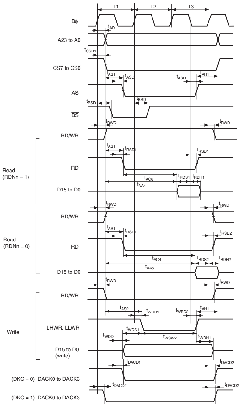
Figure 25.9 Basic Bus Timing: Three-State Access
