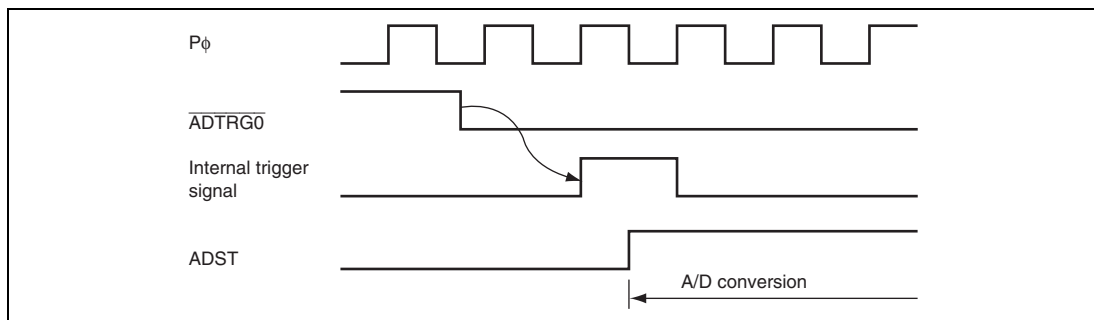
Figure 18.5 External Trigger Input Timing
