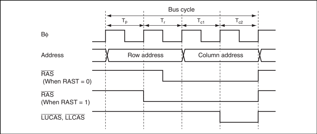
Figure 6.4 \overline{\text{RAS}} Assertion Timing (Column Address Output for 2 cycles in Full Access Mode)
