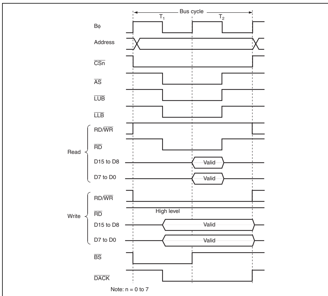
Figure 6.25 16-Bit 2-State Access Space Bus Timing
