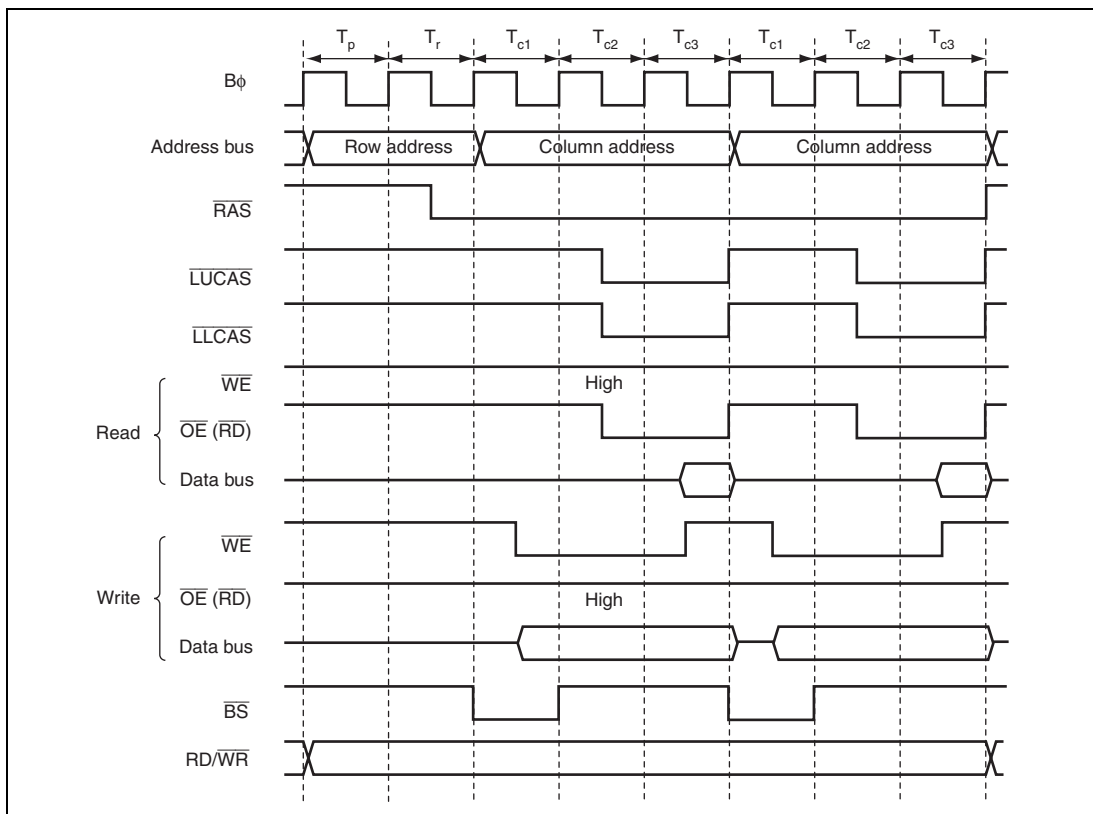
Figure 6.49 Operation Timing of Fast-Page Mode (RAST = 0, CAST = 1)
