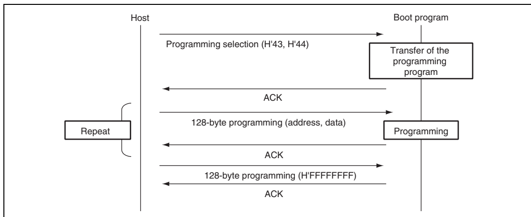
Figure 21.24 Programming Sequence
