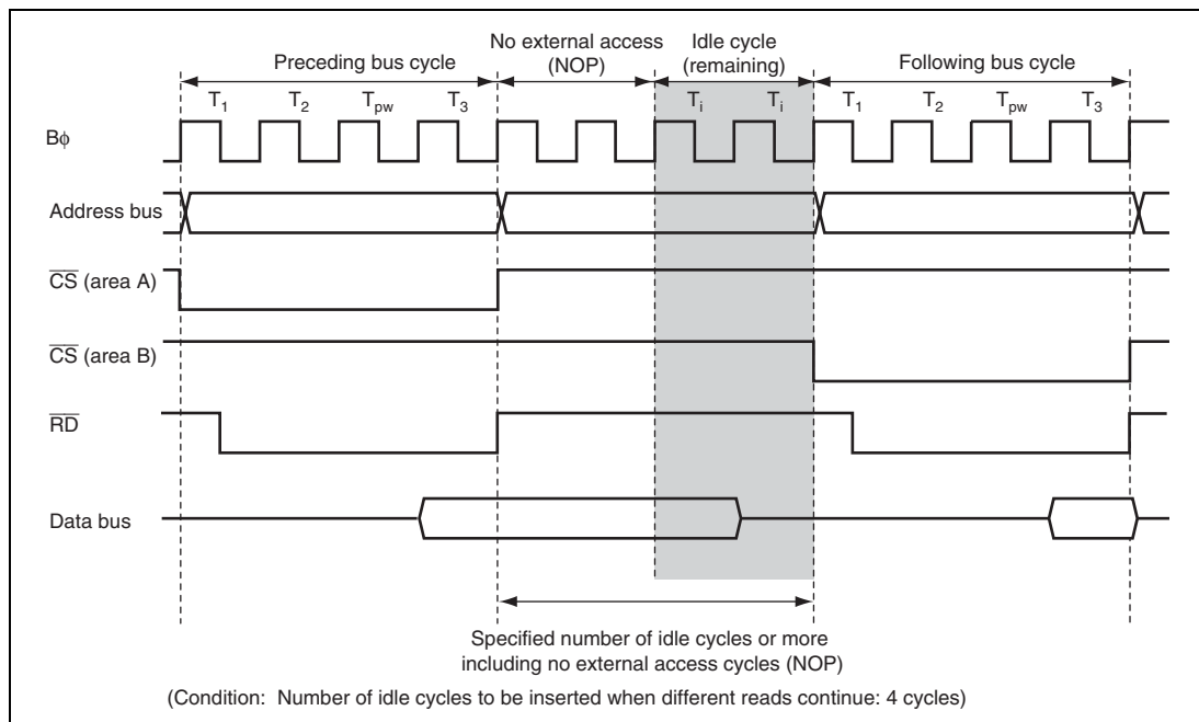
Figure 6.94 Idle Cycle Insertion Example
