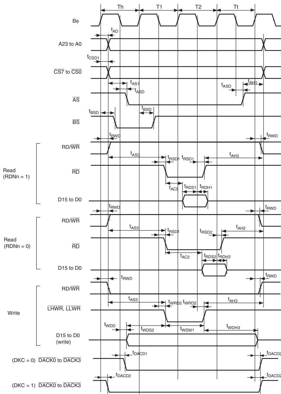
Figure 25.11 Basic Bus Timing: Two-State Access ( \overline{CS} Assertion Period Extended)
