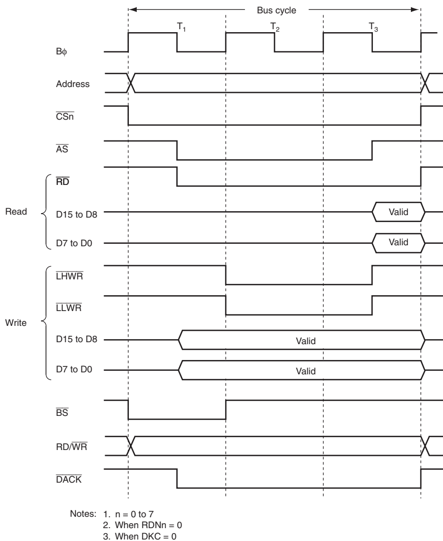
Figure 6.20 16-Bit 3-State Access Space Bus Timing (Word Access for Even Address)
