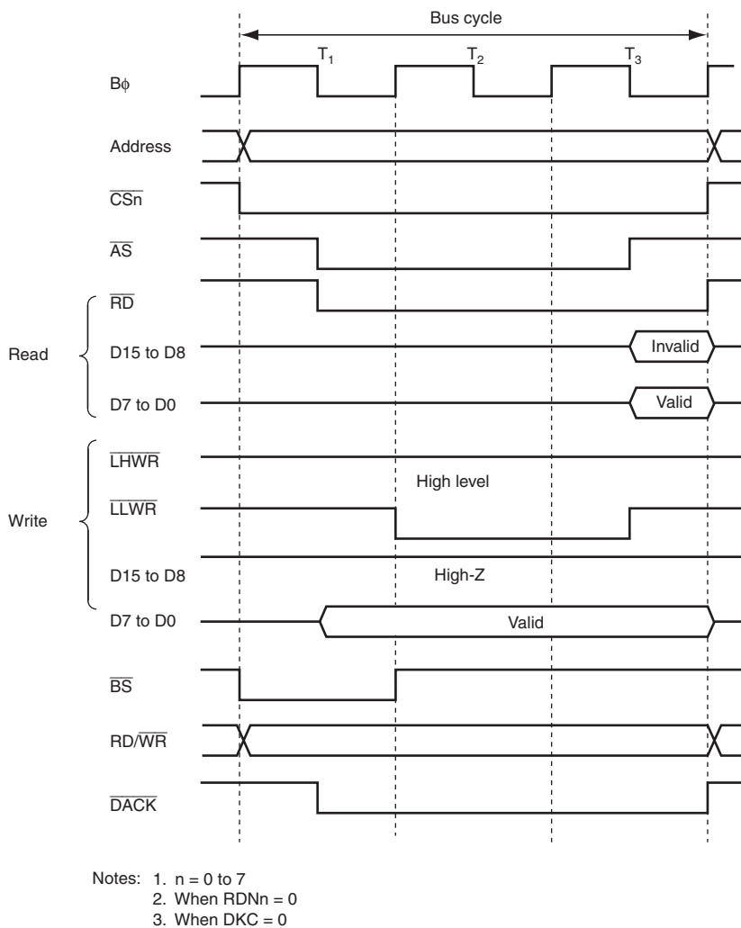
Figure 6.19 16-Bit 3-State Access Space Bus Timing (Word Access for Odd Address)
