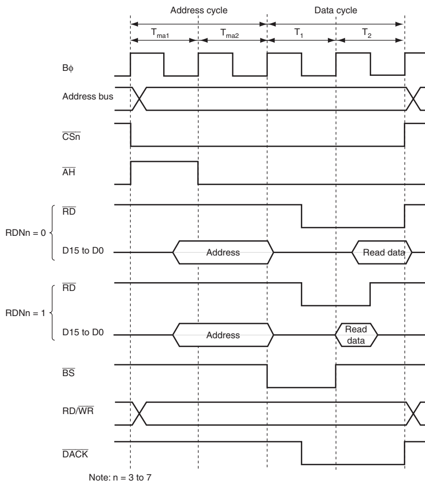
Figure 6.34 Read Strobe Timing
