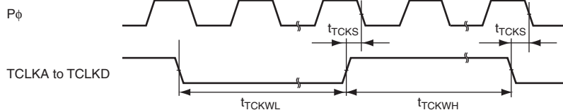
Figure 25.41 TPU Clock Input Timing
