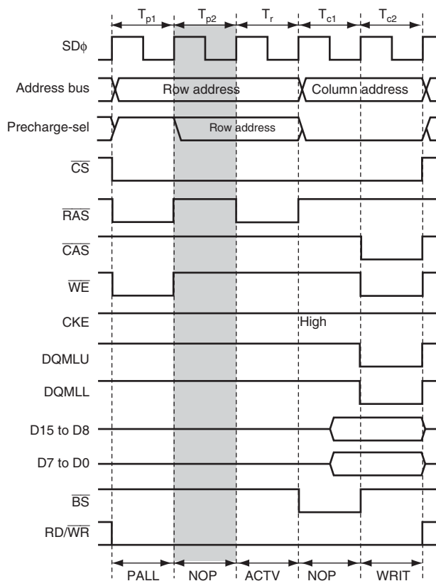
Figure 6.66 Write Timing Example of Two Precharge Cycles (TPC1 = 0, TPC0 = 1)
