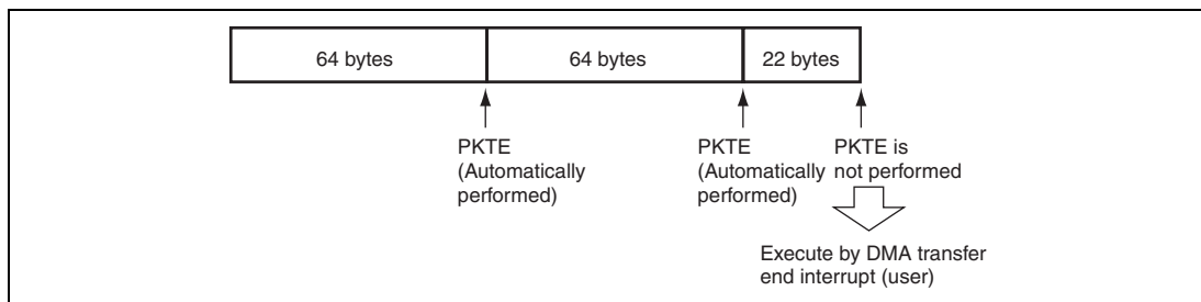
Figure 16.21 PKTE Bit Operation for EP2
