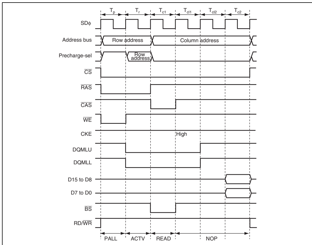
Figure 6.62 Timing Example of CAS Latency (CAS Latency = 3)
