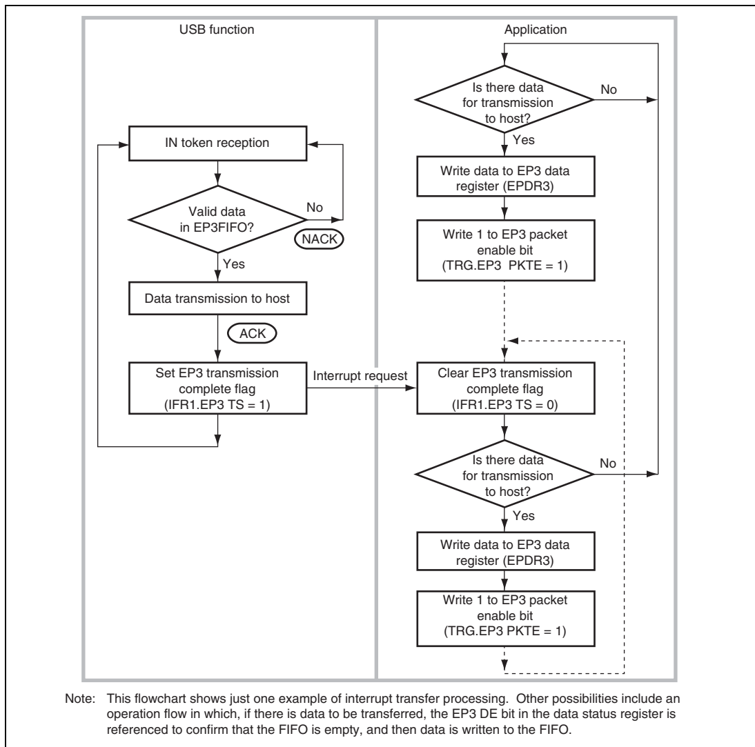
Figure 16.17 Operation of EP3 Interrupt-In Transfer
