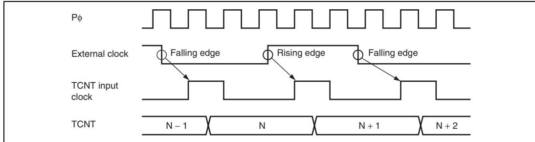
Figure 10.31 Count Timing in External Clock Operation
