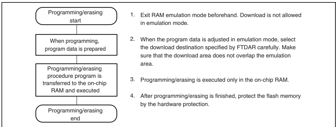
Figure 21.11 Programming/Erasing Flow
