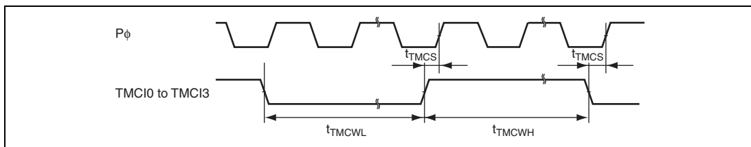
Figure 25.45 8-Bit Timer Clock Input Timing
