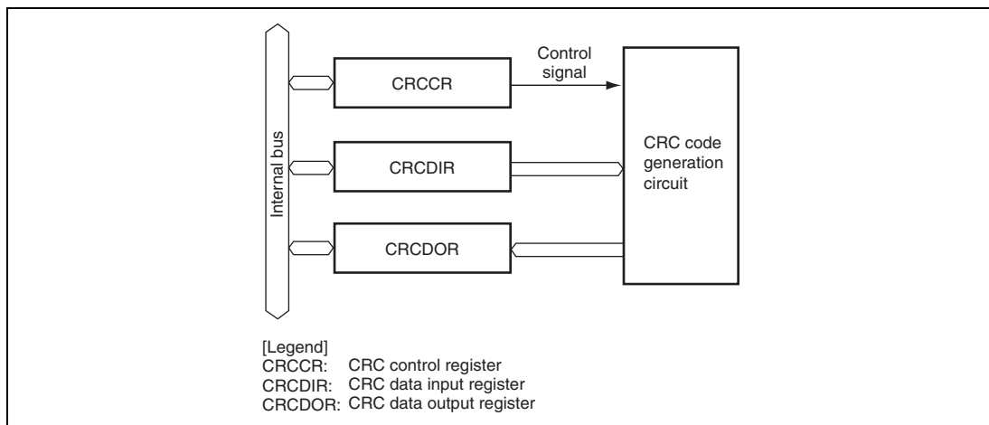
Figure 15.43 Block Diagram of CRC Operation Circuit
