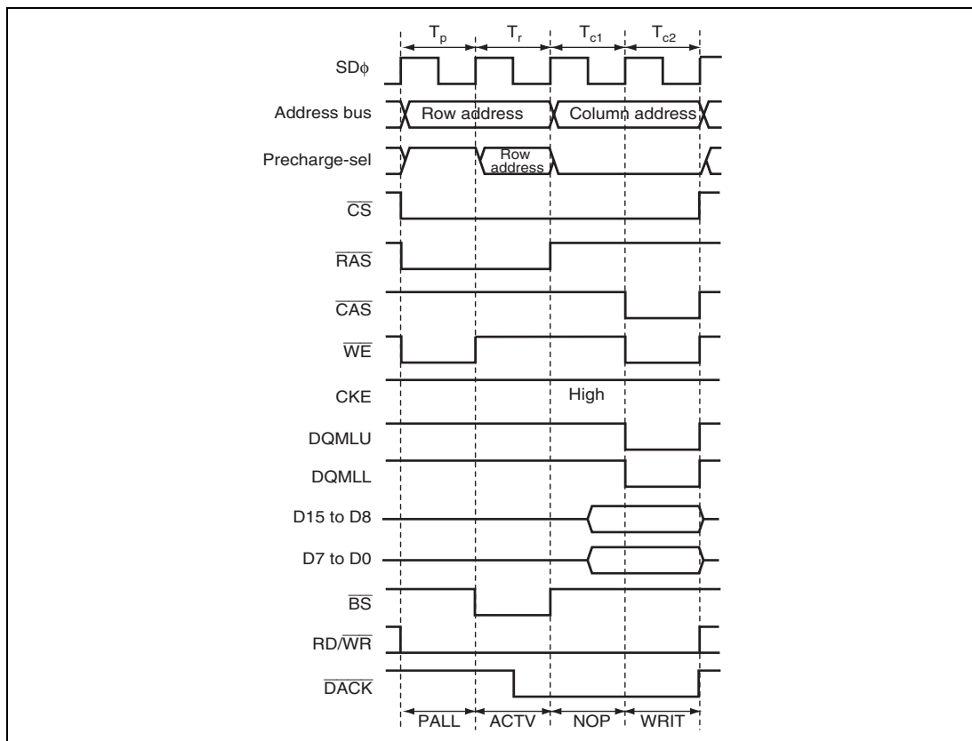
Figure 6.84 Output Timing Example of \overline{\text{DACK}} when DDS = 0 (Write)
