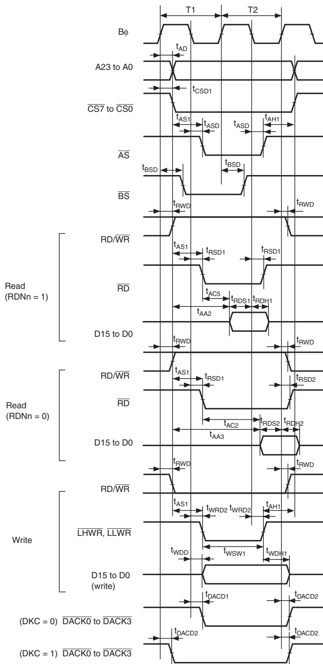
Figure 25.8 Basic Bus Timing: Two-State Access
