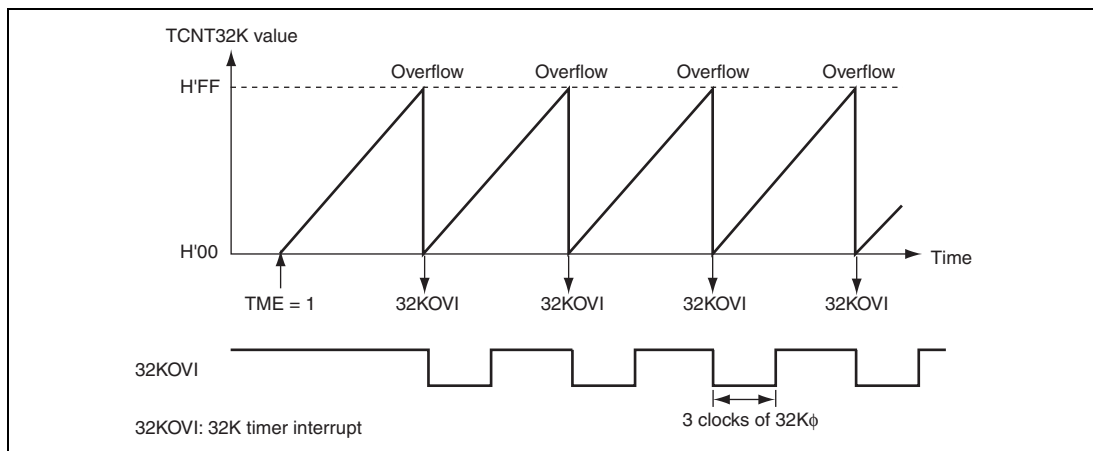
Figure 13.2 32K Timer Operation
