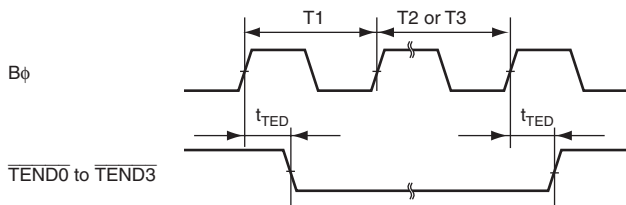
Figure 25.36 DMAC ( \overline{\text{TEND}} ) Output Timing
