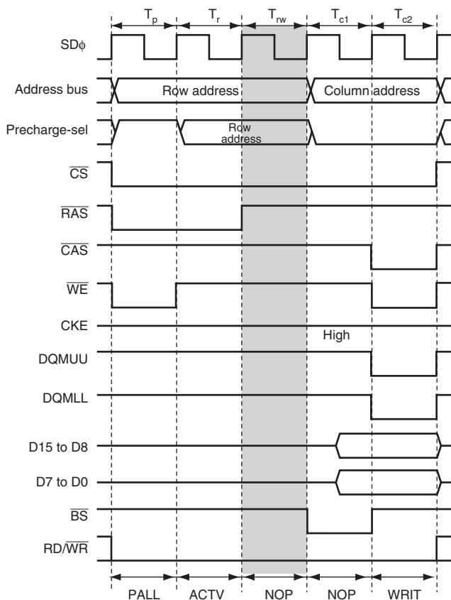
Figure 6.64 Write Timing Example of Row Address Output Retained for 1 Clock Cycle (RCD1 = 0, RCD0 = 1)
