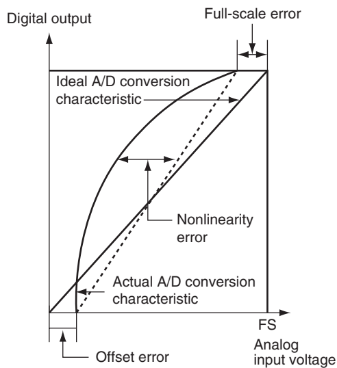
Figure 18.7 A/D Conversion Accuracy Definitions
