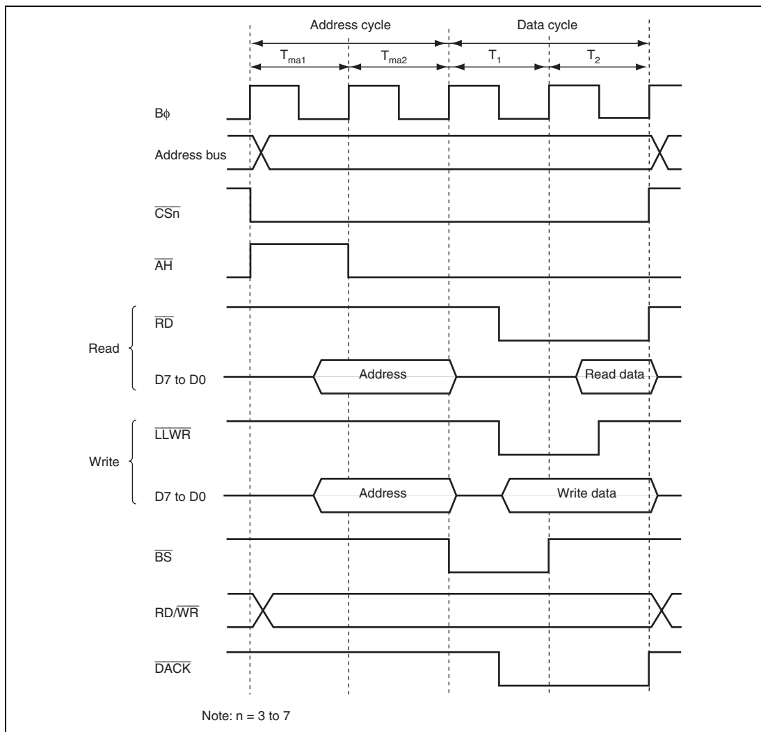
Figure 6.31 8-Bit Access Space Access Timing (ABWHn = 1, ABWLn = 1)
