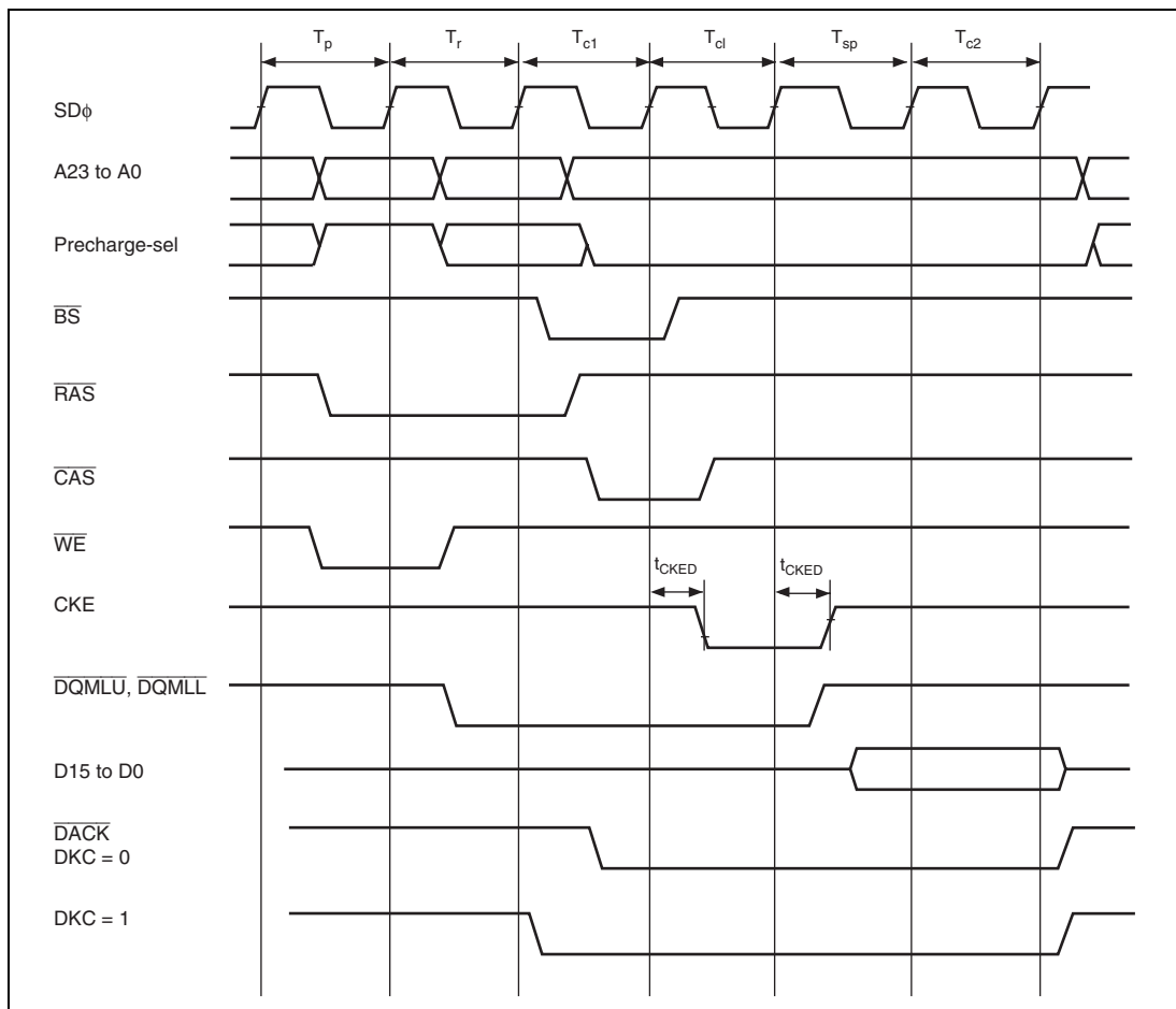
Figure 25.31 Extended Read Data Cycle (CAS Latency 2)
