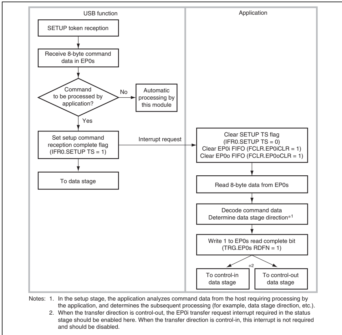
Figure 16.10 Setup Stage Operation
