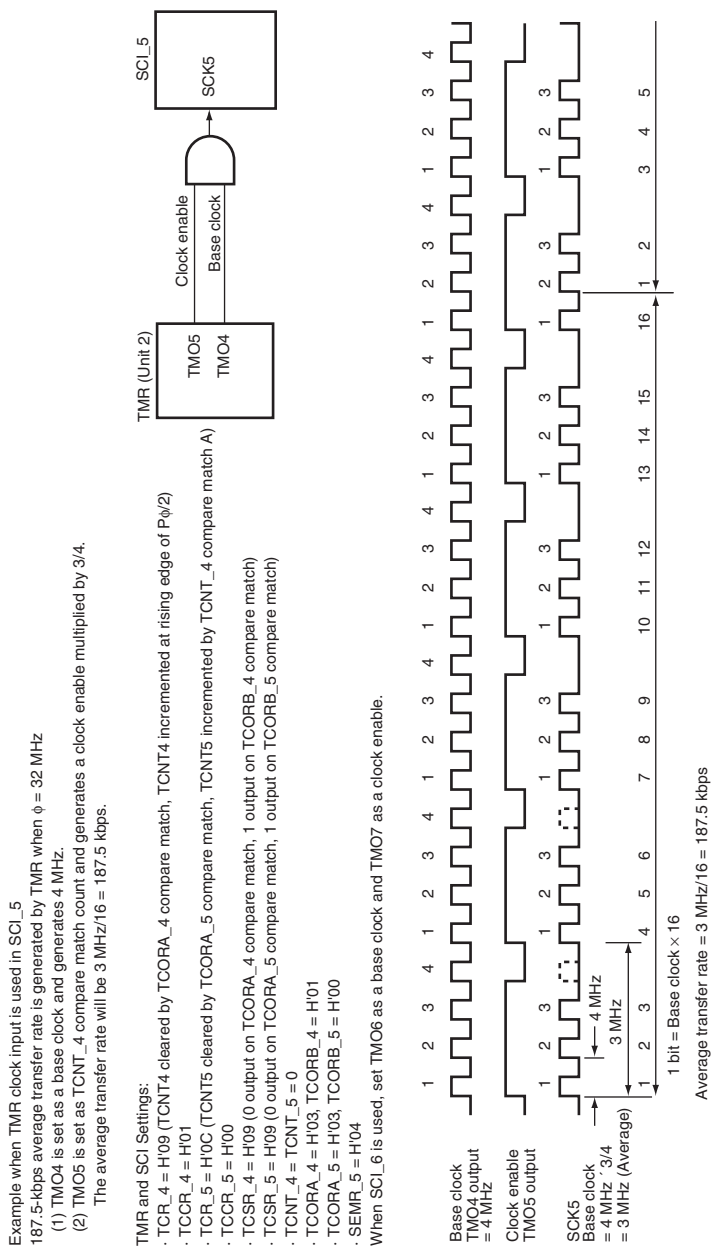
Figure 15.4 Example of Average Transfer Rate Setting when TMR Clock Is Input
