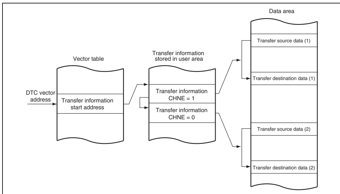
Figure 8.10 Operation of Chain Transfer
