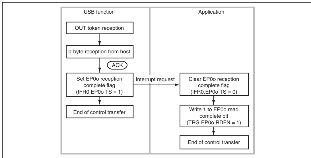
Figure 16.13 Status Stage (Control-In) Operation
