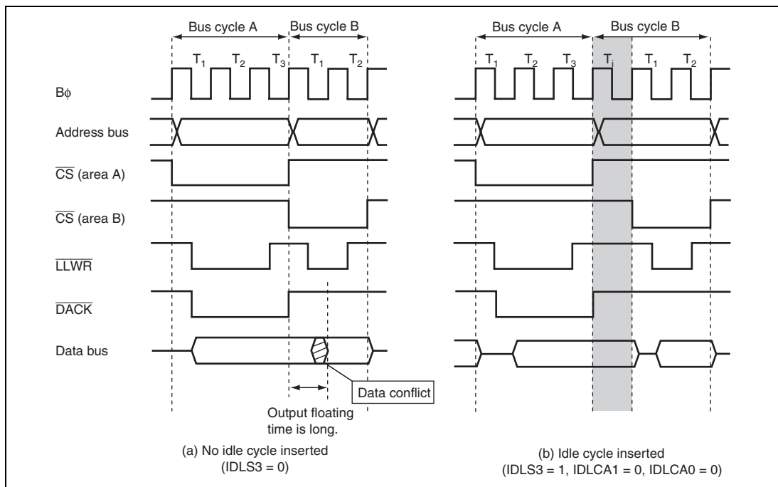
Figure 6.93 Example of Idle Cycle Operation (Write after Single Address Transfer Write)
