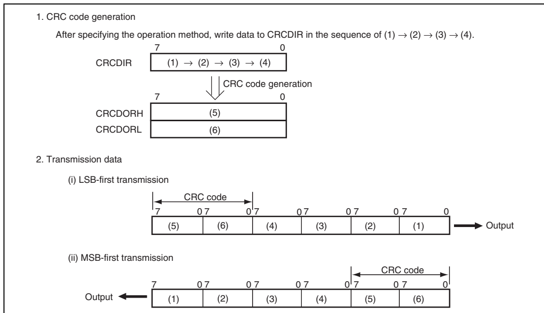
Figure 15.48 LSB-First and MSB-First Transmit Data
