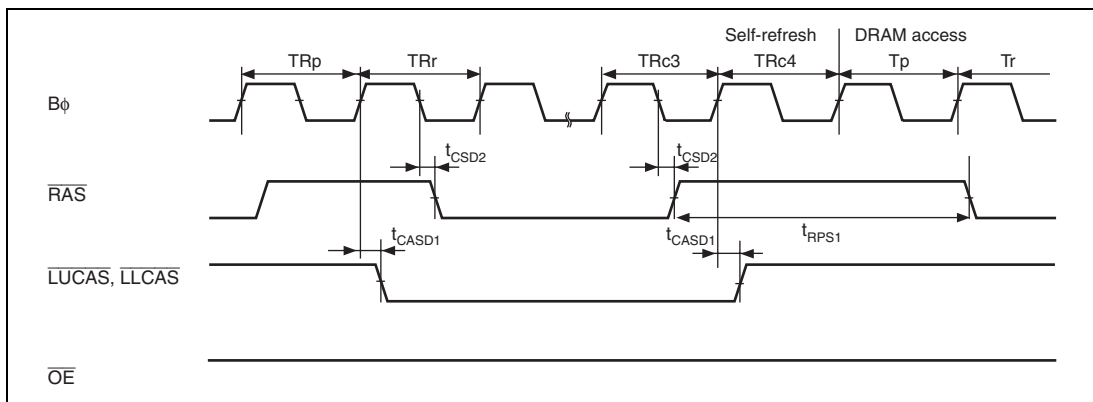
Figure 25.28 Self-Refresh Timing (After Leaving Software Standby: RAST = 1)
