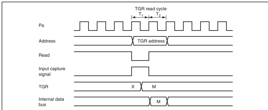
Figure 10.50 Conflict between TGR Read and Input Capture
