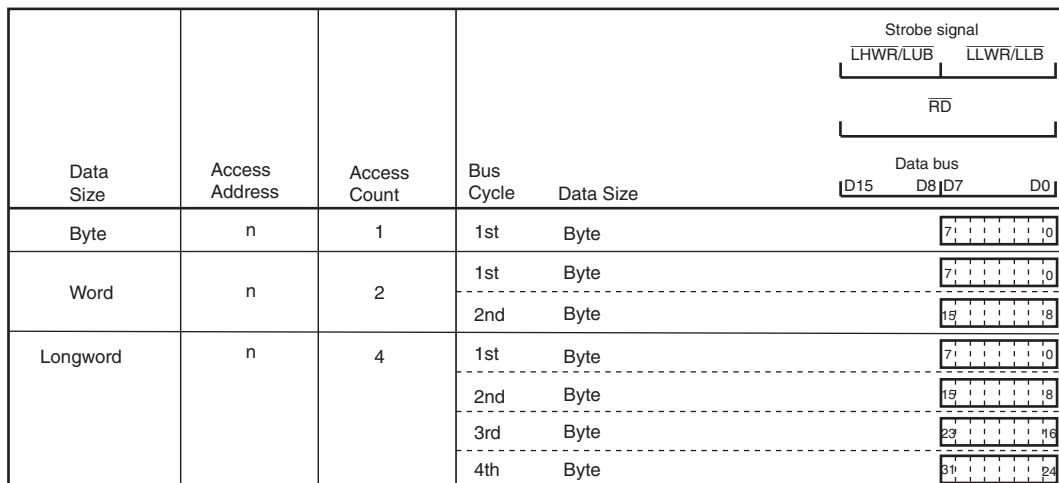
Figure 6.12 Access Sizes and Data Alignment Control for 8-Bit Access Space (Little Endian)
