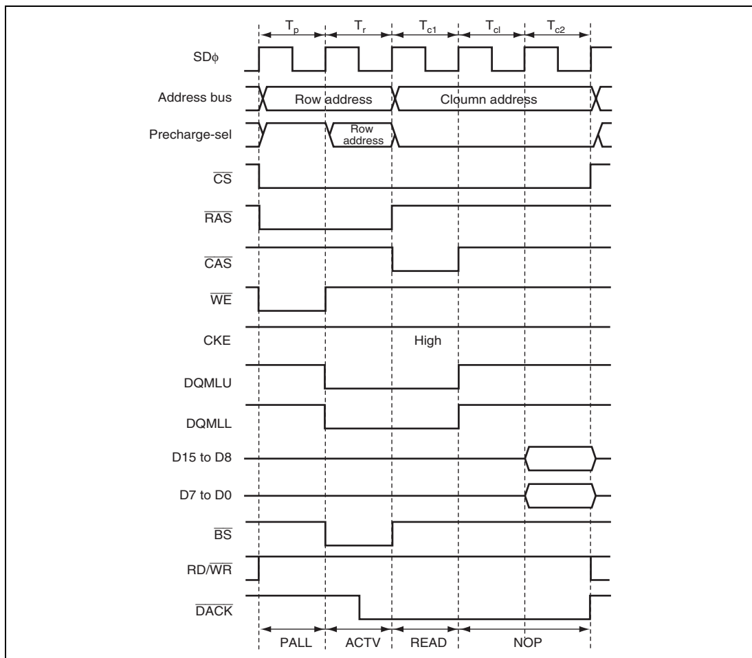
Figure 6.85 Output Timing Example of \overline{DACK} when DDS = 0 (Read, CAS Latency = 2)
