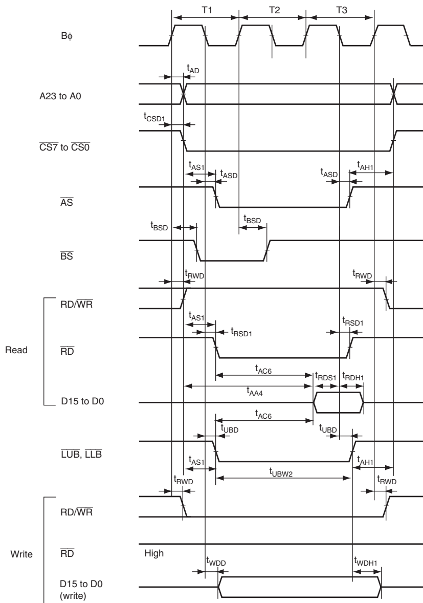
Figure 25.14 Byte Control SRAM: Three-State Read/Write Access
