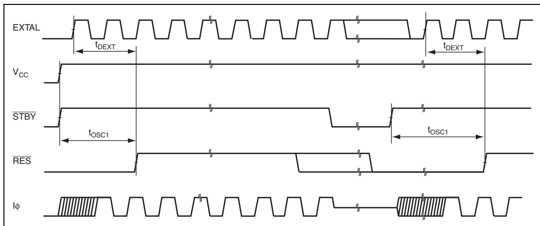
Figure 25.4 Oscillation Settling Timing
