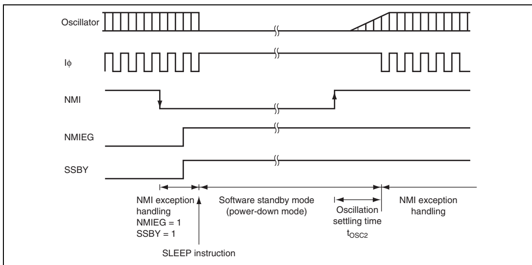
Figure 23.2 Software Standby Mode Application Example
