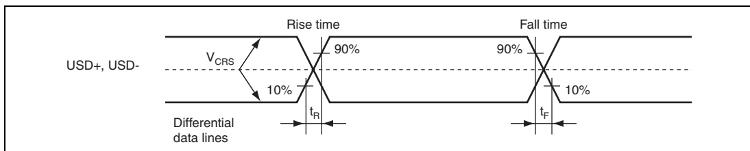
Figure 25.51 Data Signal Timing
