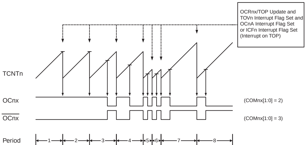
Figure 12-7. Fast PWM Mode, Timing Diagram
