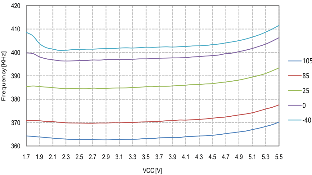
Figure 26-90. ULP 512kHz Oscillator, Frequency vs. Operating Voltage
