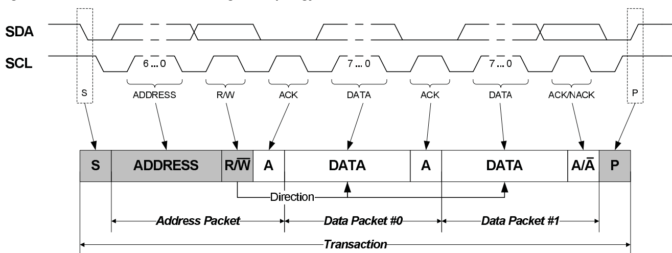
Figure 20-2. Basic TWI Transaction Diagram Topology
