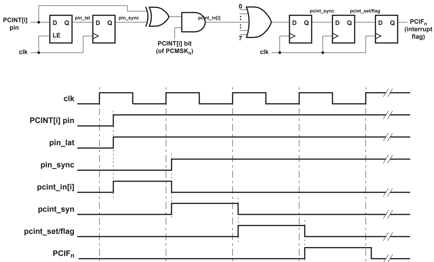
Figure 14-1. Timing of pin change interrupts
