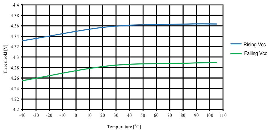
Figure 30-32. BOD Threshold vs. Temperature ( V_{CC} = 4.3V )
