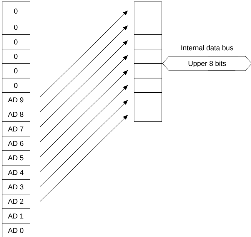
Figure 15.3 ADDR Read Operation (2)
