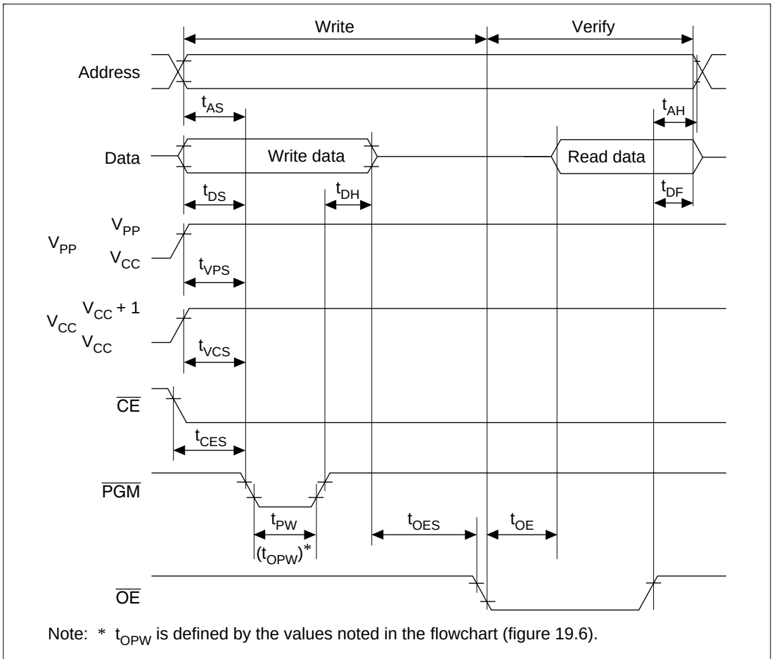
Figure 21.7 Write/Verify Timing
