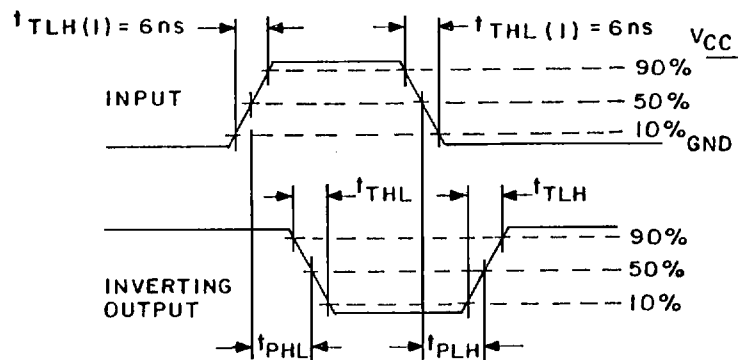
FIGURE 3. Switching waveform.
