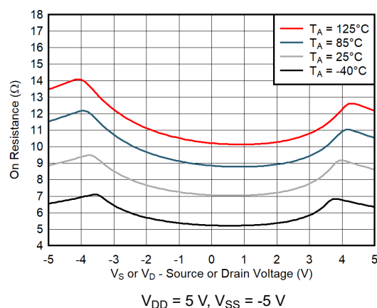
Figure 6-4. On-Resistance vs Temperature
