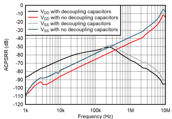
Figure 6-20. ACPSR vs Frequency
