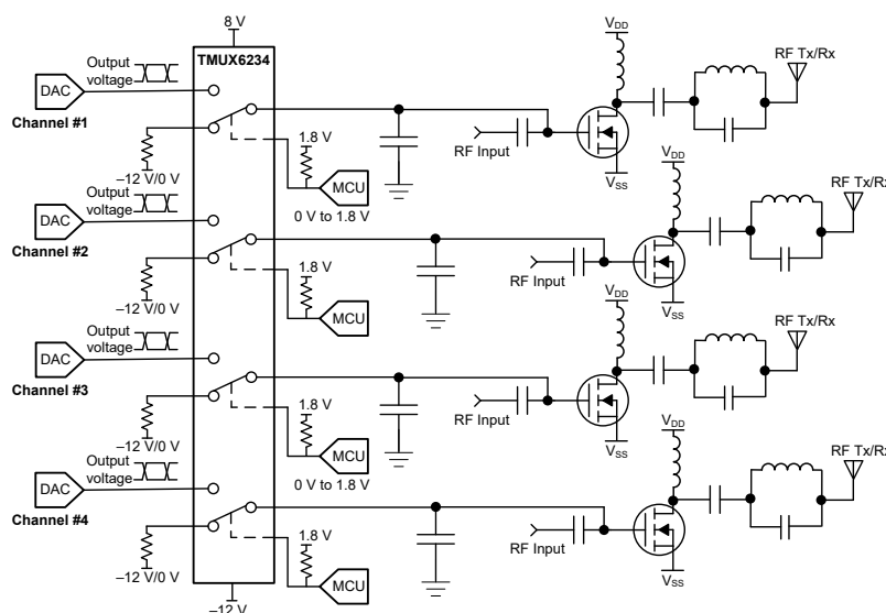
Typical Application
