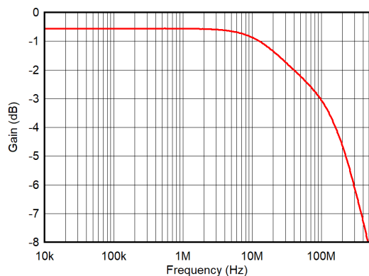
Figure 6-19. On Response vs Frequency
