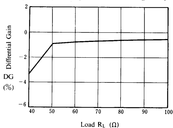
Differential Gain vs. R_L
