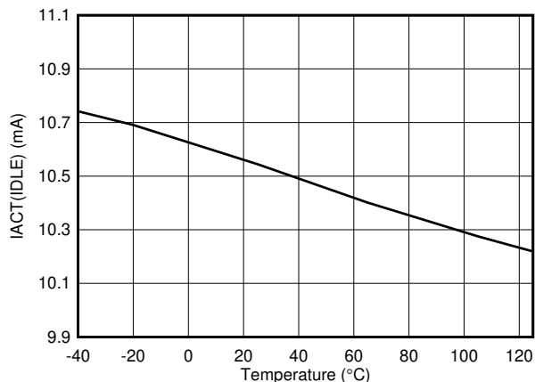
Figure 8-2. IACT (IDLE) vs Temperature
