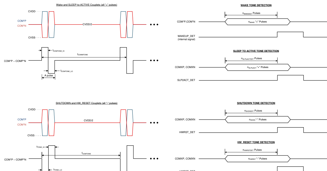
Figure 9-63. Communication Tones
