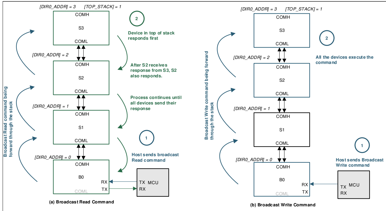
Figure 9-30. Broadcast Read/Write
