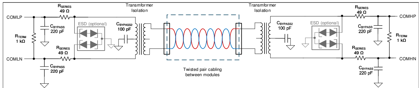
Figure 10-9. Transformer Isolation
