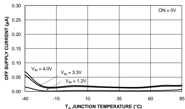
Figure 9. Off Supply Current vs. Temperature (FPF1205, V_{OUT} Floating)
