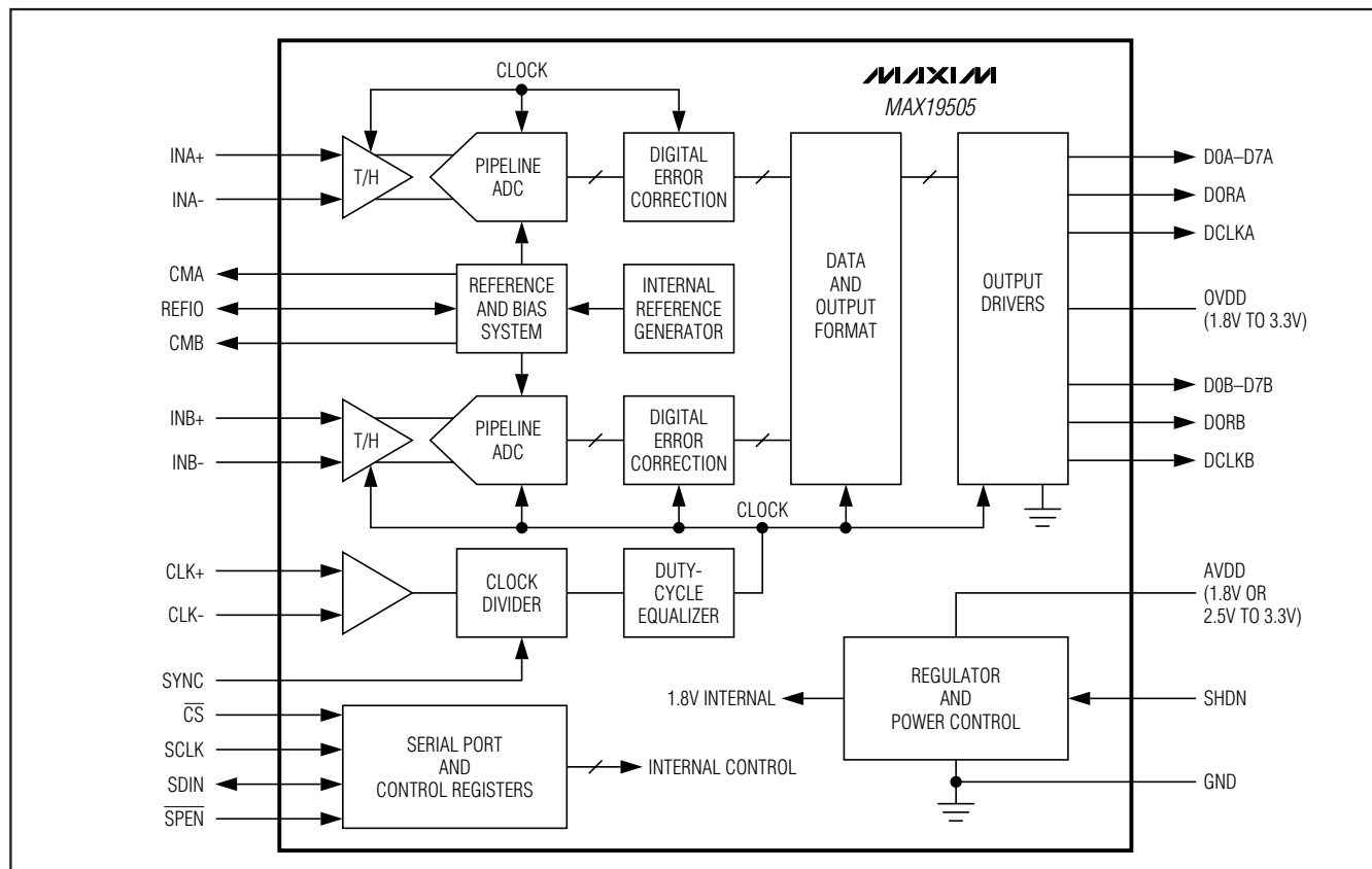
Figure 2. Functional Diagram
