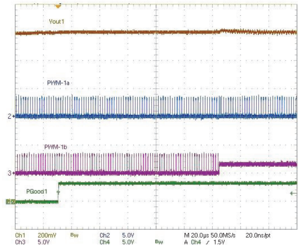
Figure 28: Phase Shed 2 \Phi à 1 \Phi at startup
