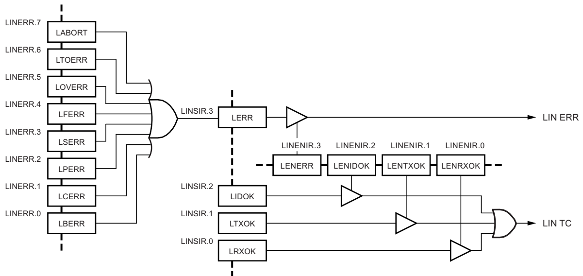
Figure 15-13.LIN Interrupt Mapping
