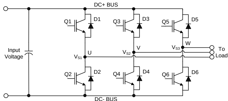
Figure 22: Three phase inverter
