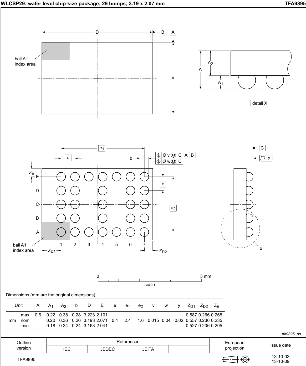
Fig 7. Package outline TFA9895 (WLCSP29)
