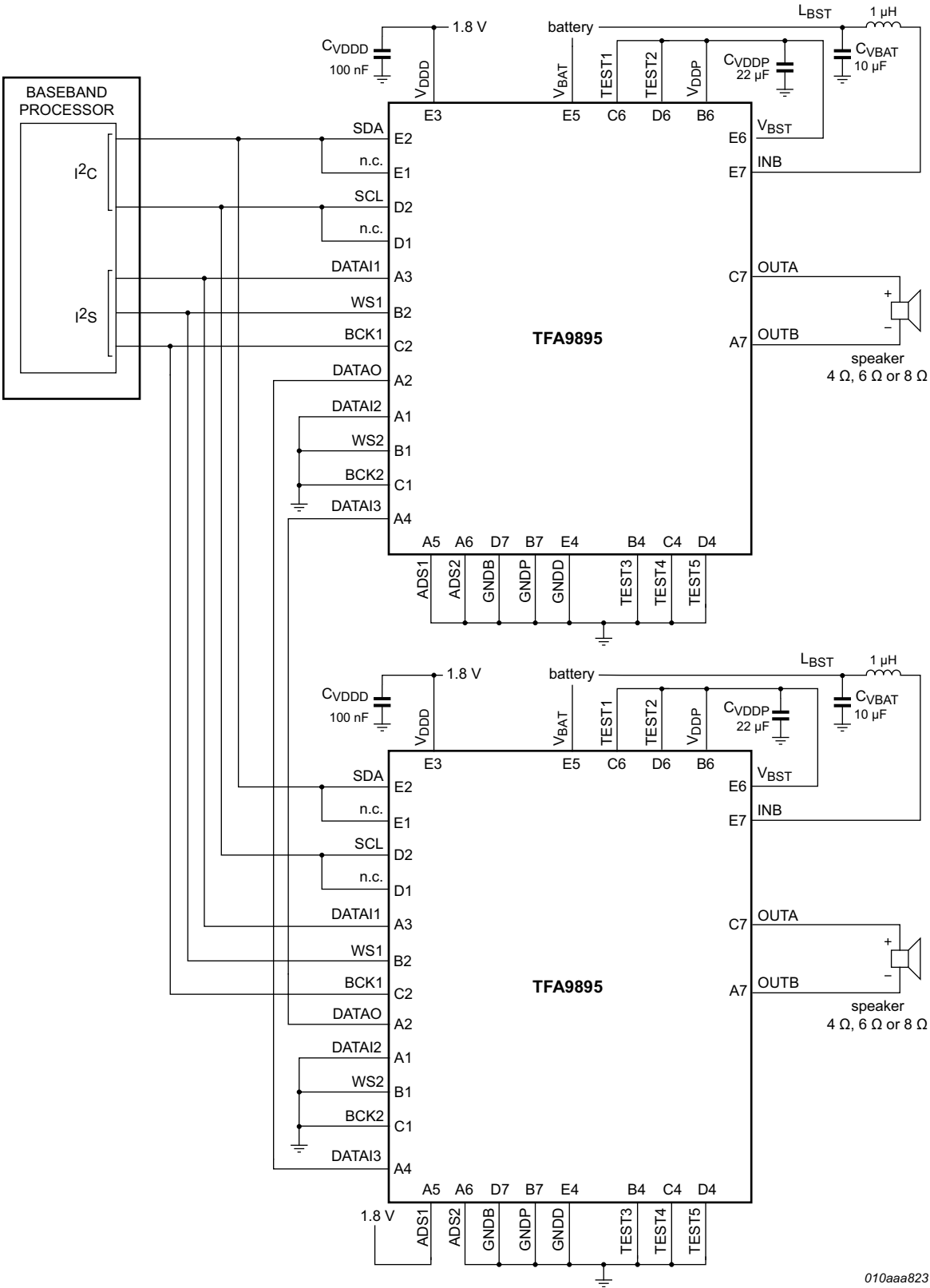
Fig 5. Typical stereo application (simplified) TFA9895_SDSAll information provided in this document is subject to legal disclaimers.© NXP B.V. 2013. All rights reserved. Product short data sheetRev. 1 — 23 October 201313 of 21
