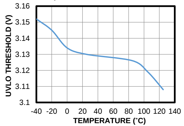
VG UVLO Threshold vs. Temperature
