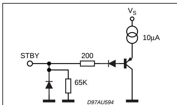
Figure 15. PIN: STBY
