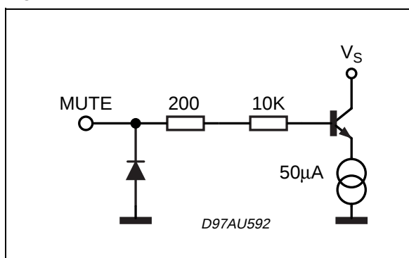
Figure 17. PIN: MUTE
