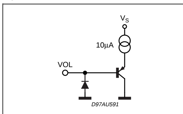
Figure 13. PIN: VOLUME
