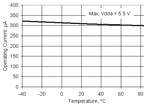
Figure 11-48. VDAC Operating Current vs Temperature, 1 V Mode, High speed mode
