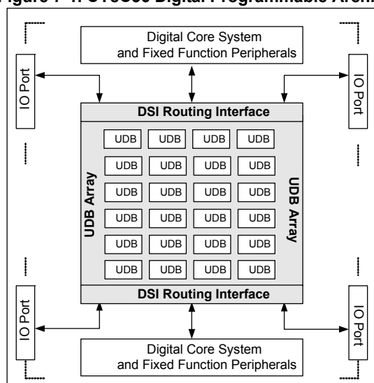
Figure 7-1. CY8C36 Digital Programmable Architecture
