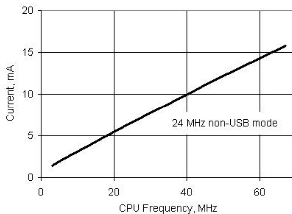
Figure 11-1. Active Mode Current vs F_{CPU} , V_{DD} = 3.3\text{ V} , Temperature = 25\text{ }^{\circ}\text{C}
