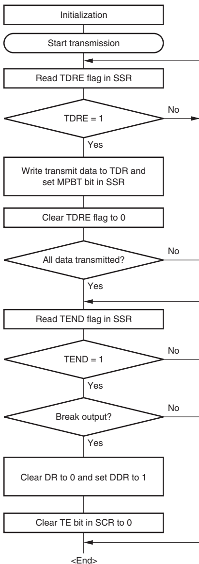
Figure 12.11 Sample Multiprocessor Serial Transmission Flowchart
