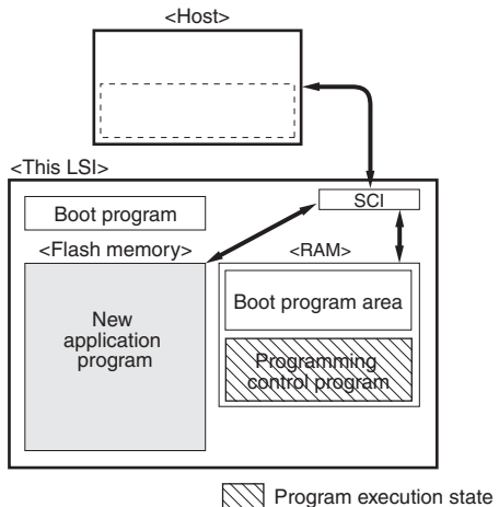
Figure 16.3 Boot Mode
