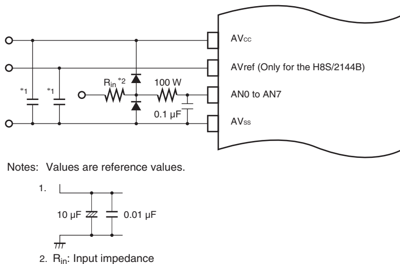
Figure 14.8 Example of Analog Input Protection Circuit
