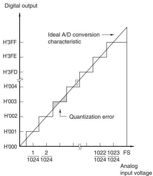
Figure 14.5 A/D Conversion Accuracy Definitions
