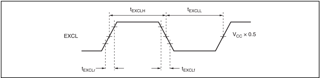
Figure 17.7 Subclock Input Timing
