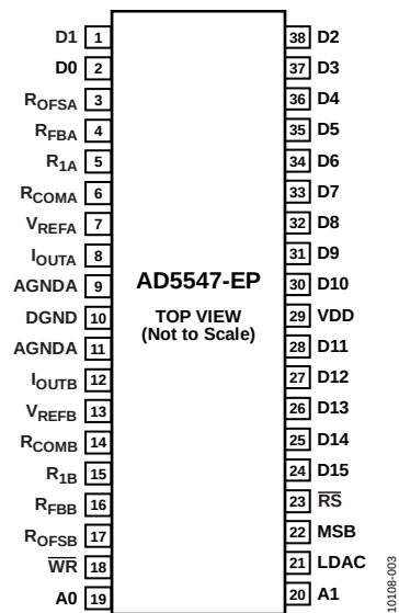
Figure 4. Pin Configuration
