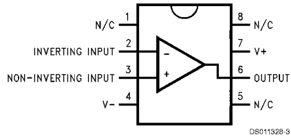
8-Pin Dual-In-Line Package (N)/ Small Outline (M-8)
