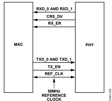
Figure 23. MII MAC to PHY Interface Signals
