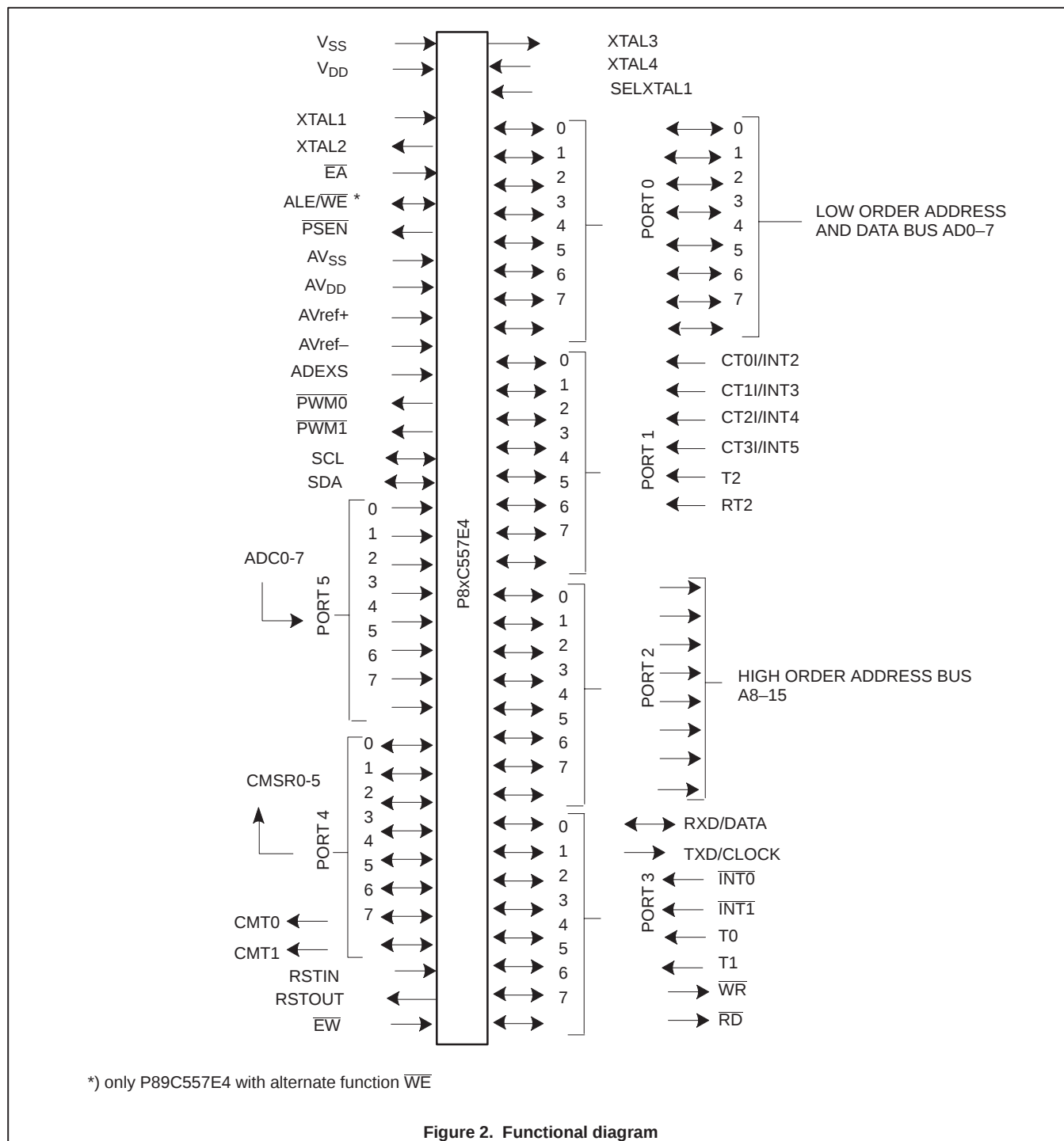
Figure 2. Functional diagram
