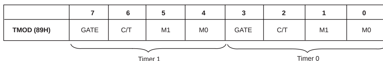
Figure 19. Timer/Counter mode control (TMOD) register.
