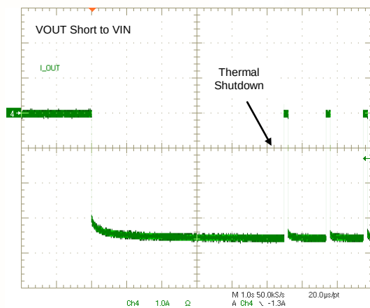
Current Limit Test (VIN=1.5V)
