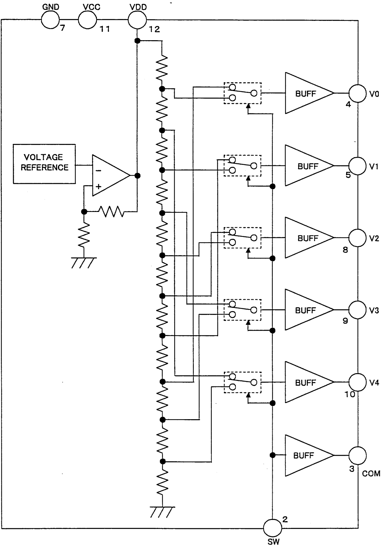
4. Block Diagram
