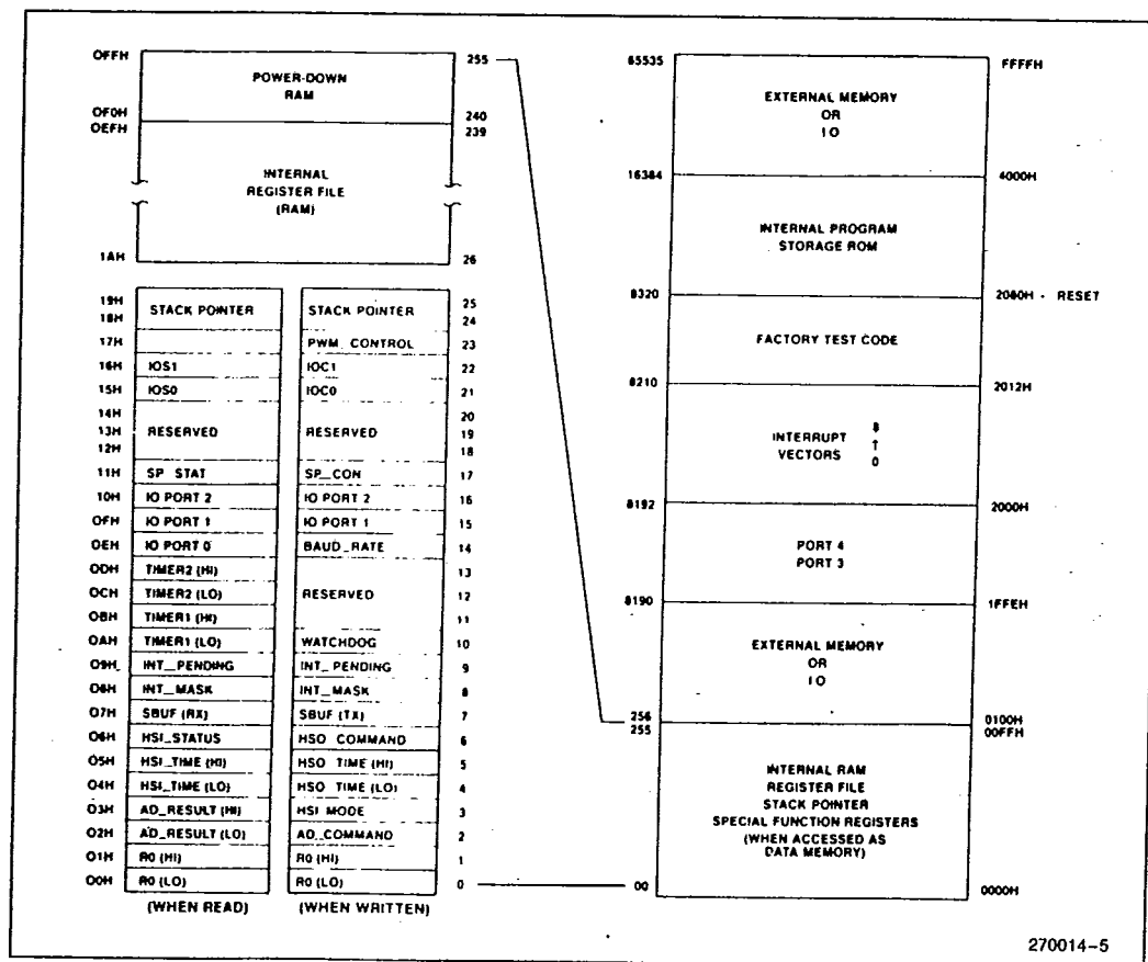
Figure 5. Memory Map
