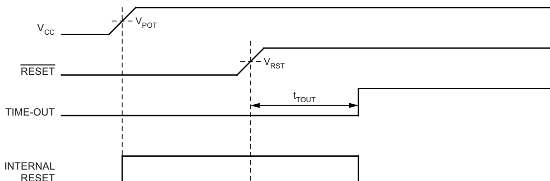
Figure 9-3. MCU Start-up, RESET Extended Externally
