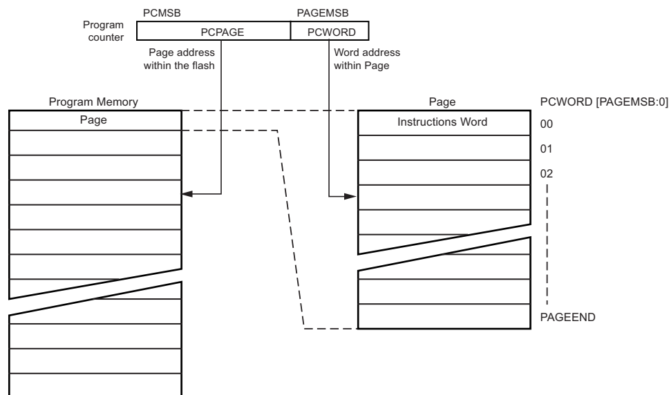
Figure 22-2. Addressing the Flash Which is Organized in Pages (1)
