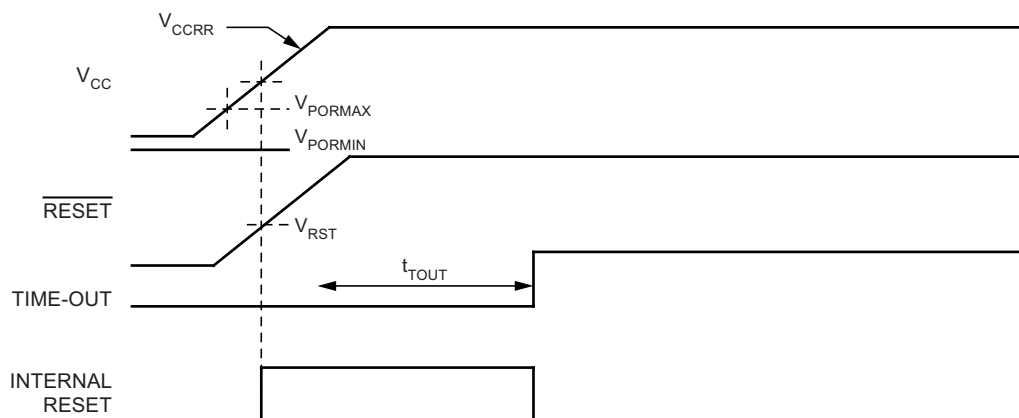
Figure 9-2. MCU Start-up, RESET Tied to V_{CC}
