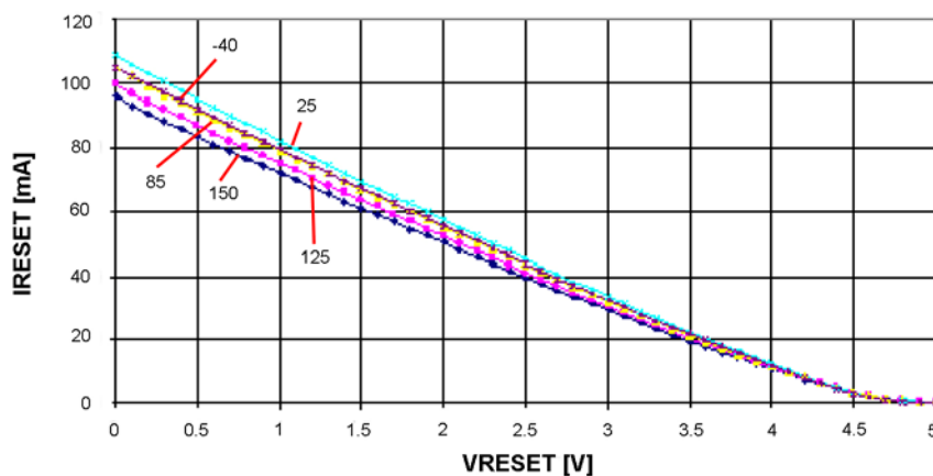
Figure 24-7. Reset Pull-up Resistor Current versus Reset Pin Voltage ( V_{CC} = 5V )
