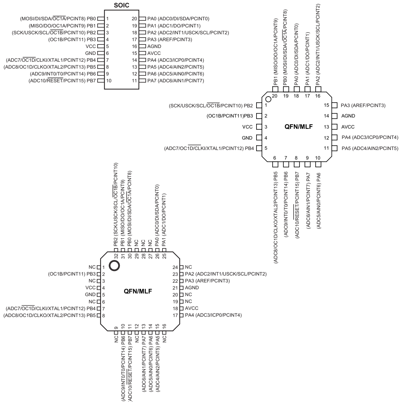
Figure 1-1. Pinout ATtiny261/461/861
