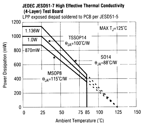
Figure 3. Package Power Dissipation vs Ambient Temperature
