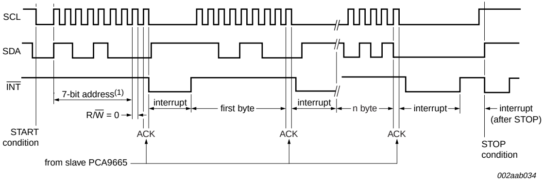
Slave PCA9665 is written to by external master transmitter.
