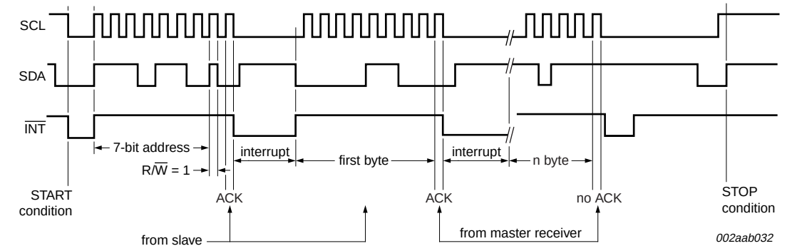
Master PCA9665 reads data from slave transmitter.
