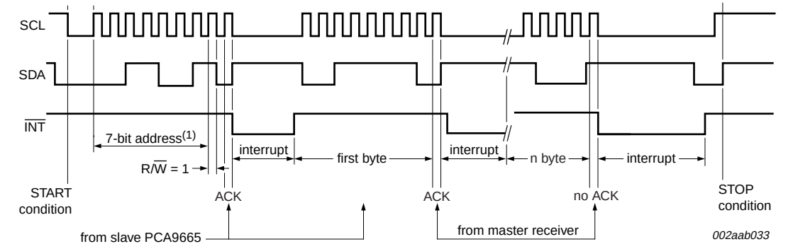
External master receiver reads data from PCA9665.
