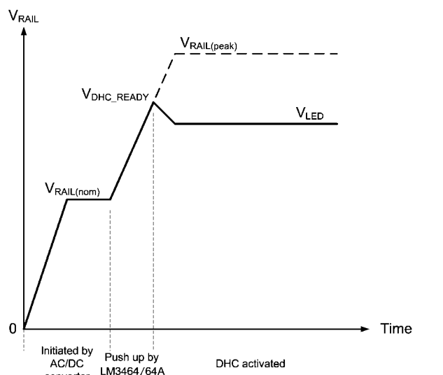
FIGURE 3. Changes of Rail Voltage Upon Power Up
