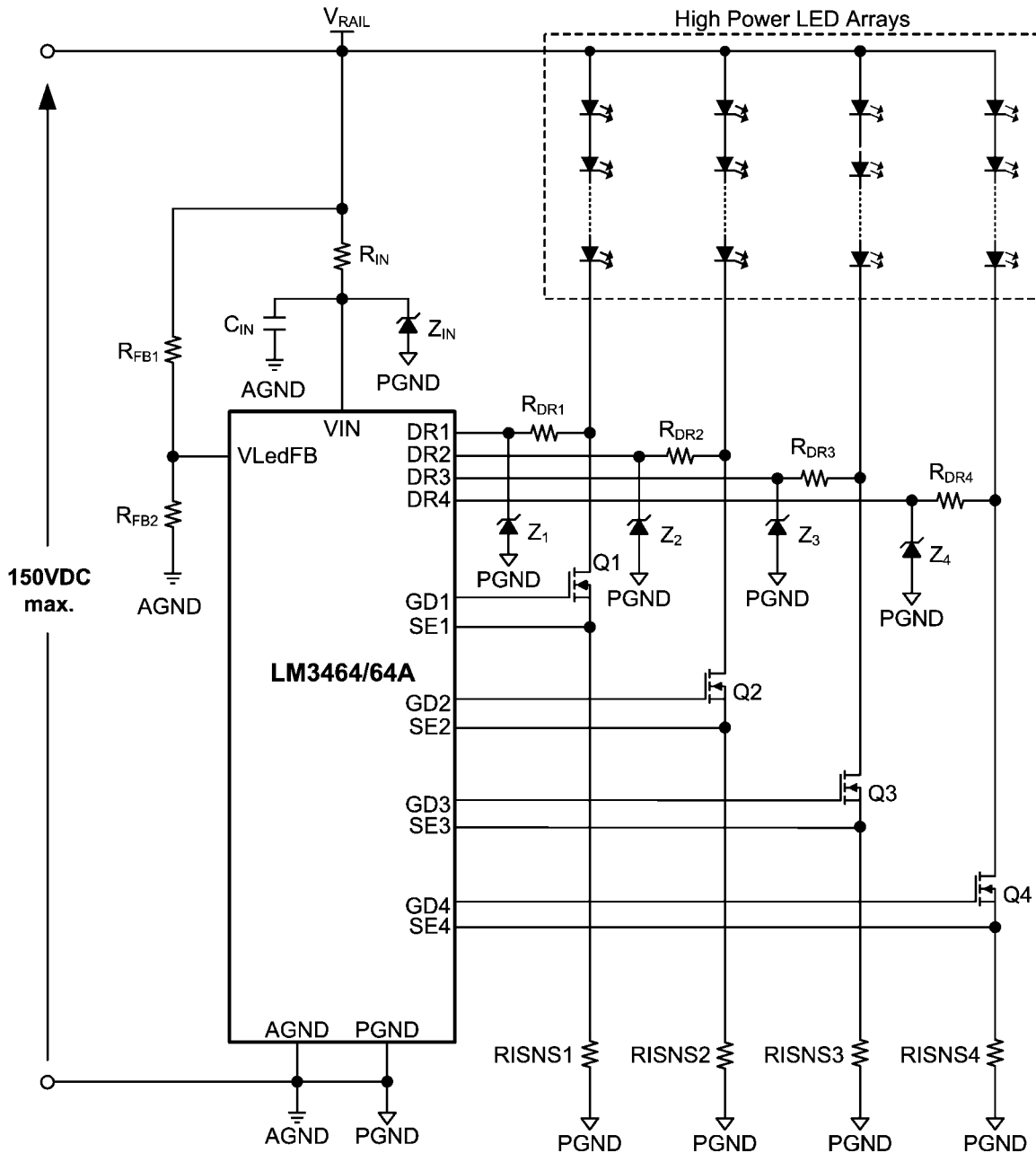
FIGURE 13. Additional Voltage Clamping Circuits for V_{\text{RAIL(peak)}} > 80\text{V}/95\text{V} (LM3464/64A)
