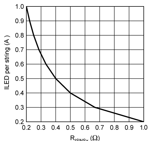
FIGURE 6. LED Current vs R_{\text{SNSx}}
