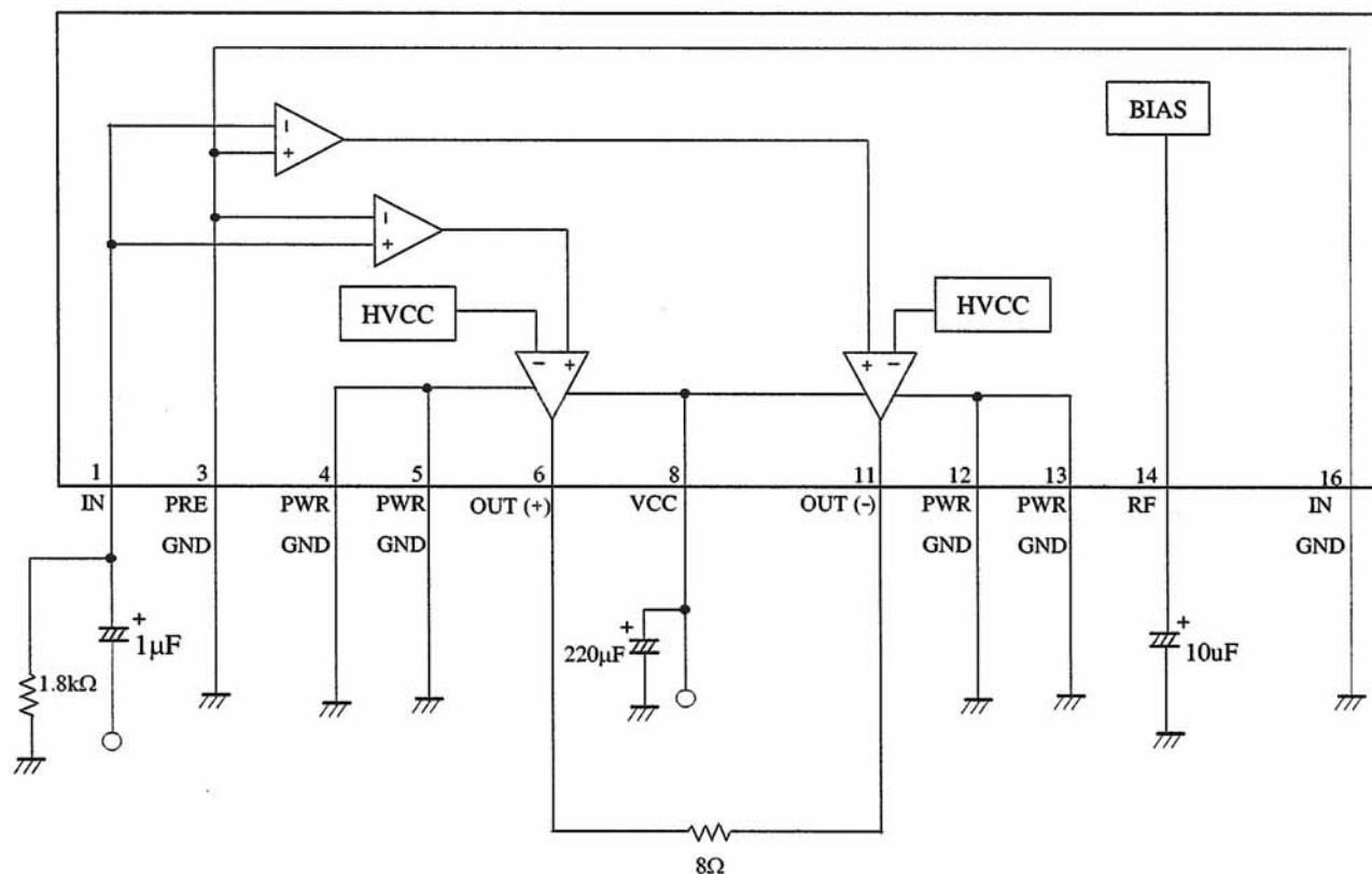
Test Circuit 1
