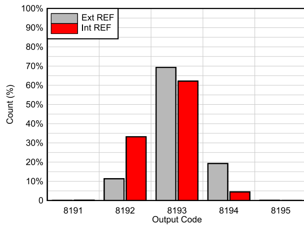
Figure 6-13. DC Histogram
