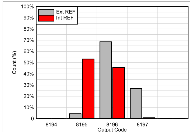
Figure 6-34. DC Histogram
