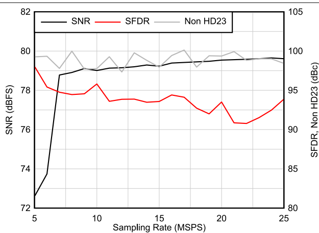
Figure 6-28. AC Performance vs Sampling Rate
