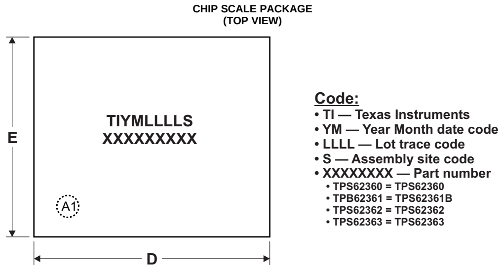
Figure 53. Package Marking and Dimensions
