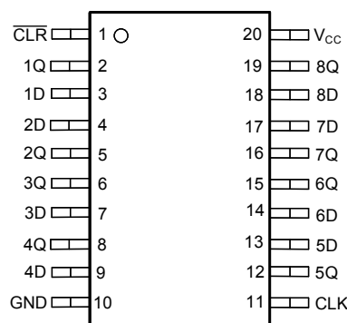
Figure 5-2. SN74LV273A-Q1 DGS Package, 20-Pin VSSOP (Top View)
